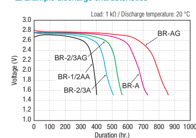
■ Example discharge characteristics
