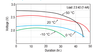
■ Discharge temperature characteristics (Example: BR435)
