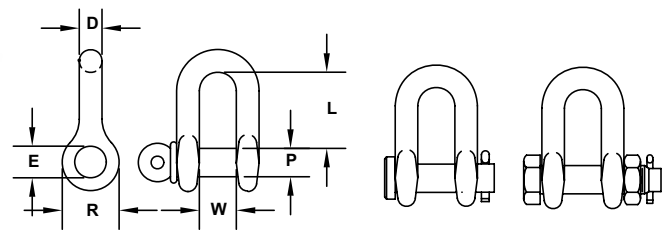
Screw Pin
