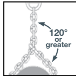
SINGLE CHOKER
