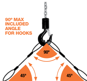
CORRECT INCORRECT
