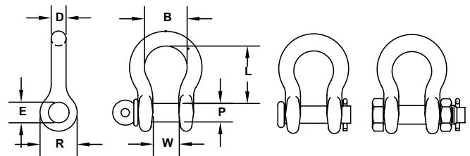
Round Pin
