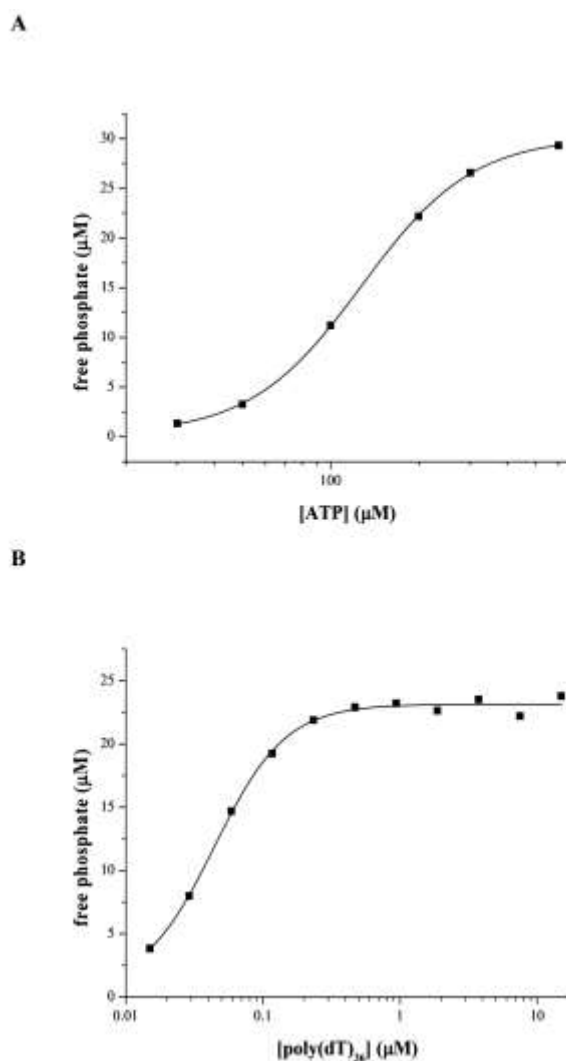
Fig. 1. Semi-log plot of free phosphate produced by RecA ATPase activity as function of A) concentrations of ATP, B) concentrations of poly(dT) 36 . All the experiments were performed in triplicate. Experimental error never exceeds 5%.
