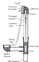
Trip Lever Bath Waste
