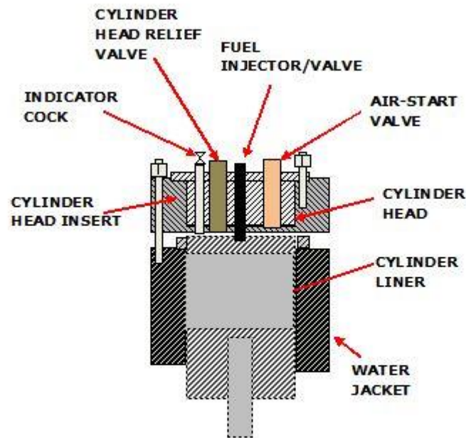
SECTIONS THROUGH CYLINDER HEAD AND INSERT ON SULZER RD ENGINE
