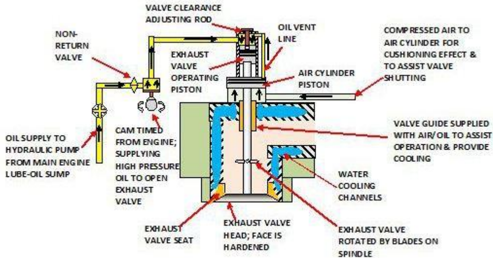
SECTION THROUGH TYPICAL EXHAUST VALVE USED ON MODERN TWO-STROKE MARINE DIESEL ENGINES
