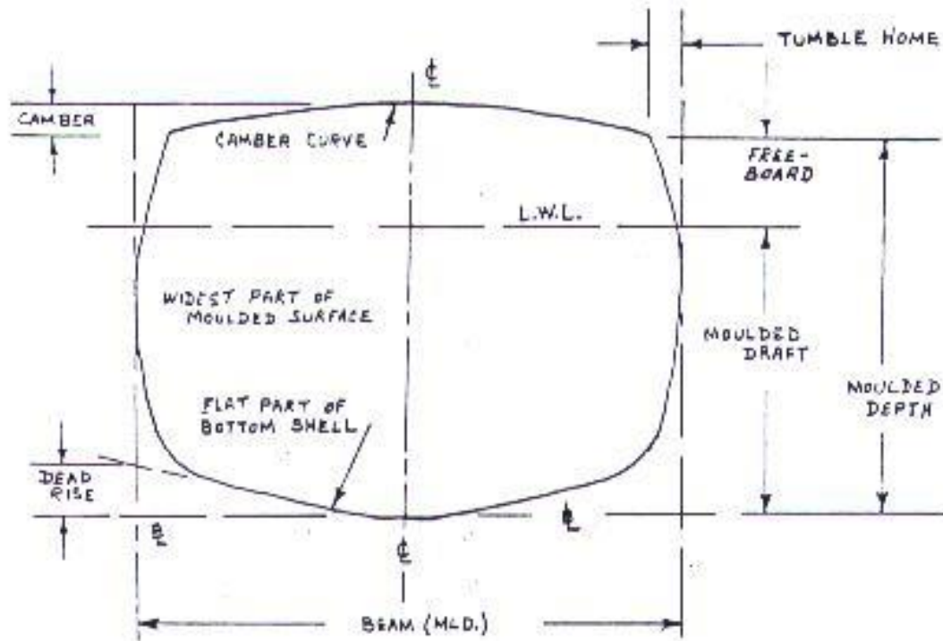
FIG. 3 - Moulded Dimensions at Midship Section
