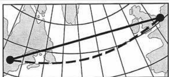
— Great Circle 3150 NM - - - Rhumb line 3290 NM
