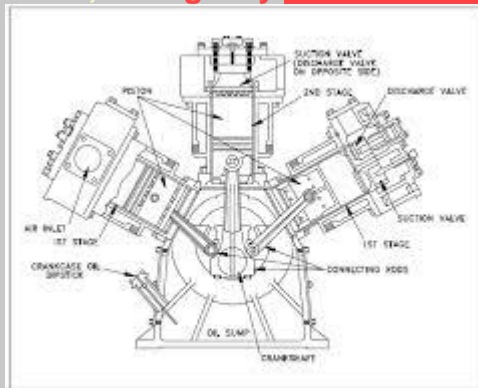
Figure 3 Reciprocating Air Compressor
