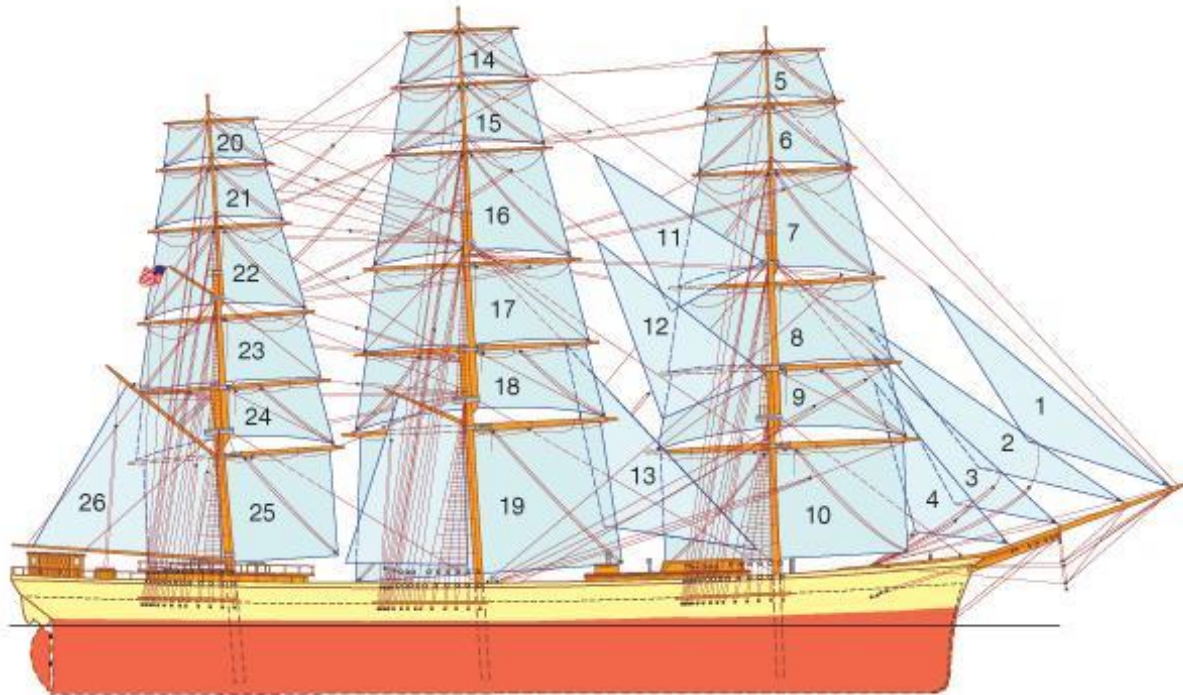
(1) flying jib. (2) outer jib. (3) inner jib. (4) jib. (5) fore skysail. (6) fore royal. (7) fore topgallant sail. (8) fore upper topsail. (9) fore lower topsail. (10) foresail. (11) main royal staysail. (12) main topgallant staysail. (13) main topmast staysail. (14) main skysail. (15) main royal. (16) main topgallant sail. (17) main upper topsail. (18) main lower topsail. (19) mainsail. (20) mizzen skysail. (21) mizzen royal. (22) mizzen topgallant sail. (23) mizzen upper topsail. (24) mizzen lower topsail. (25) crossjack. (26) spanker or driver.
