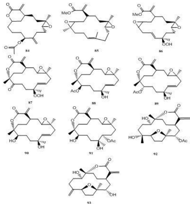
Figure 9: Diversity of flexilarins A (84) - J (93) from the Taiwanese S. flexibilis .
