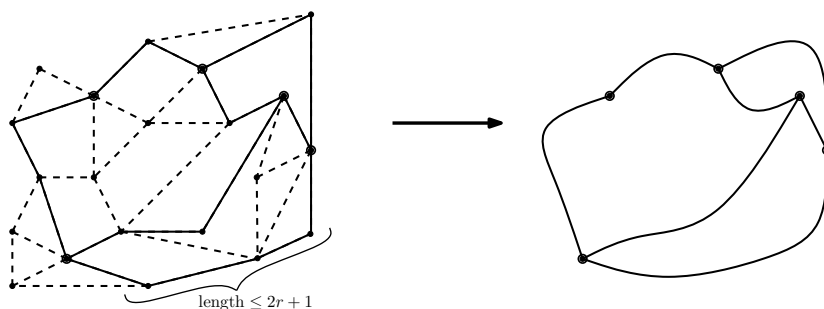
Figure 2: A shallow topological minor of depth r of a graph G is a simple subgraph of a minor of G obtained by contracting internally vertex disjoint paths of length at most 2r + 1
