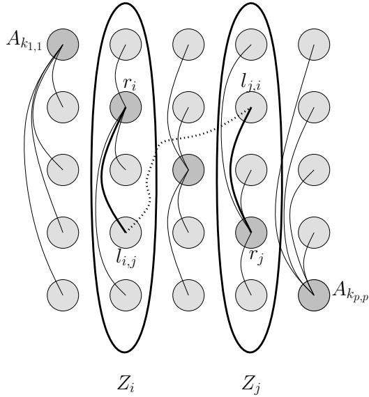
Figure 3: Finding a \leq (9k + 10) -subdivision of K_p . The dotted line corresponds to the path L_{k_{i,j}, k_{j,i}} .
