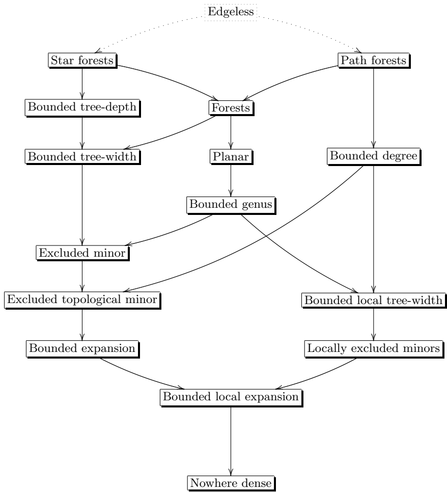
Figure 4: Inclusion map of classes of graphs and structures
