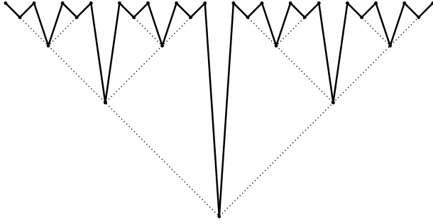
Figure 6: The tree-depth of a path is logarithmic in the order of the path
