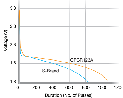
1200mA pulse discharge to 1.3V at -20°C
