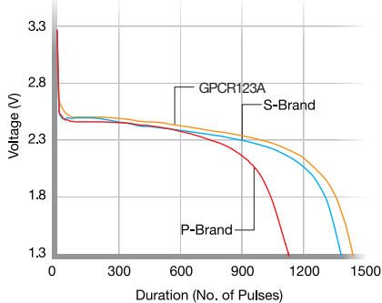
1200mA pulse discharge to 1.3V at 23°C
