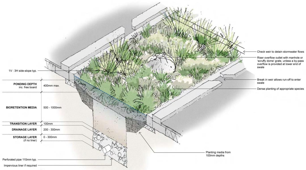
Figure 20: Schematic of bioretention swale
