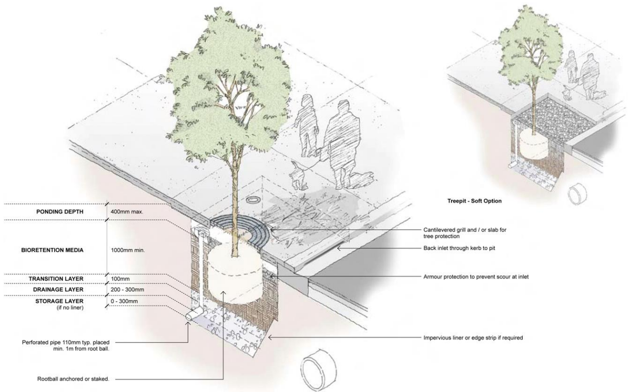
Figure 18: Schematic of stormwater tree pit
