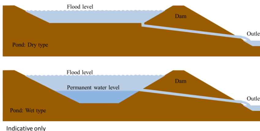
Figure 54: Schematic of dry and wet pond profiles
