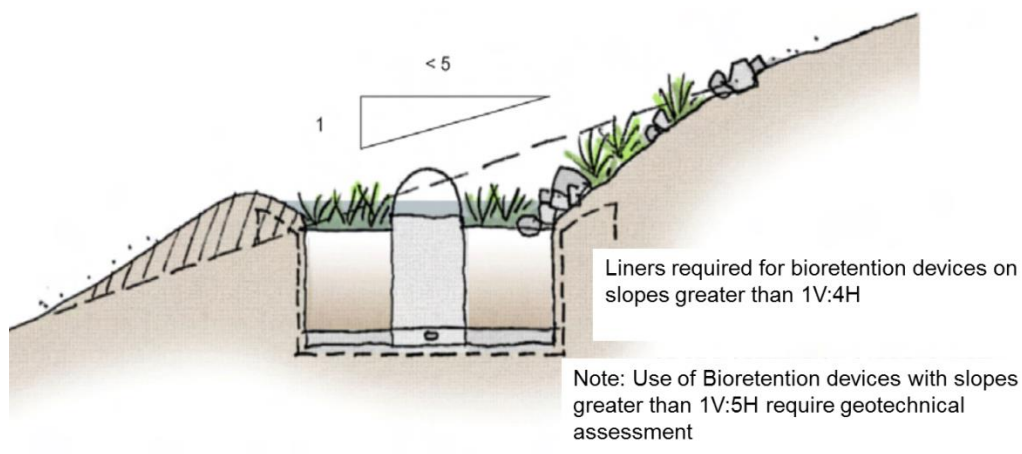
Figure 22: Schematic of slope constraints and liner use
