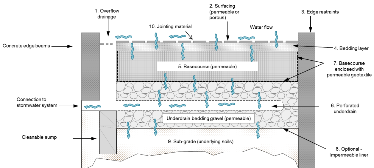
Figure 13: Schematic of pervious paving
