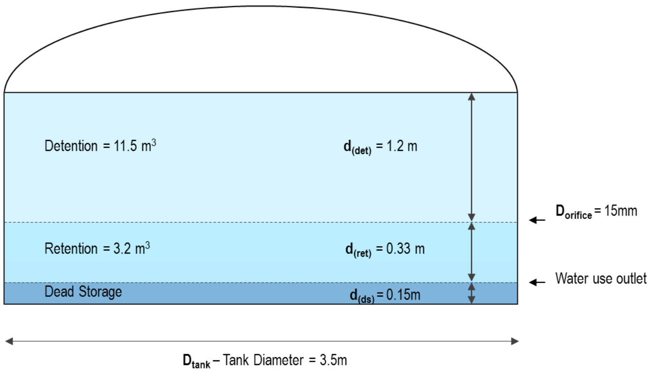
Figure 40: Rainwater tank specifications for mitigation of 800 m 2 roof (15000 L)
