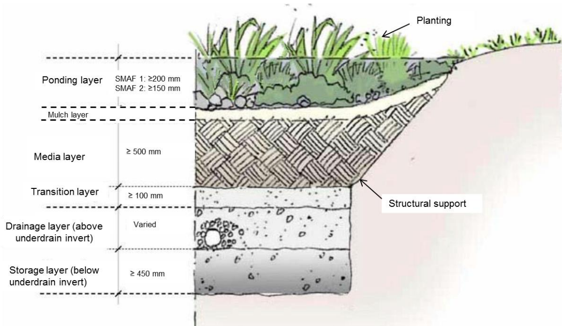
Figure 15: Schematic of rain garden cross-section
