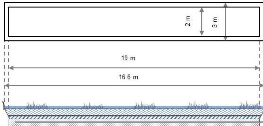
Figure 25: Rain garden design for 1000 m 2 carpark
