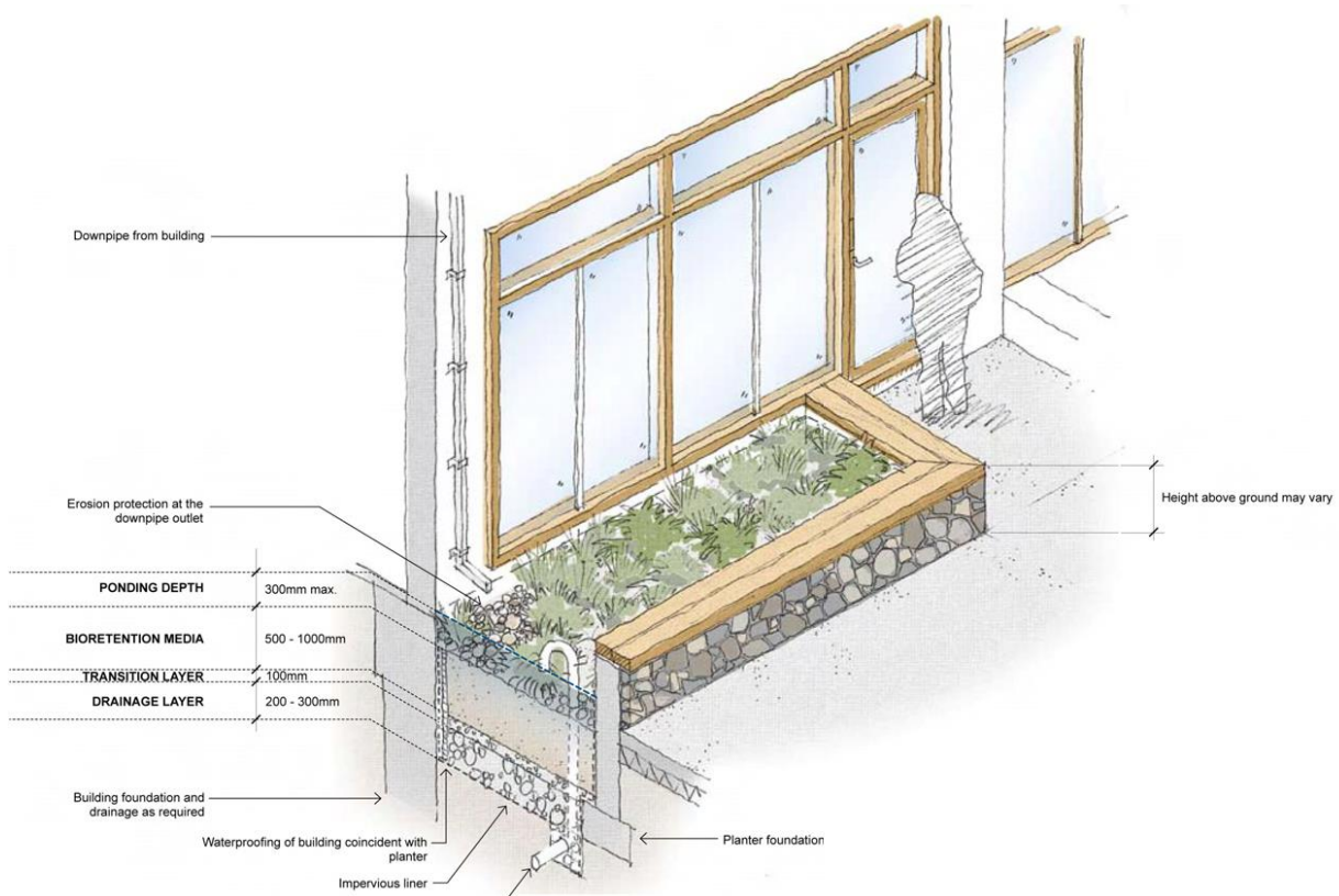
Figure 17: Schematic of planter box
