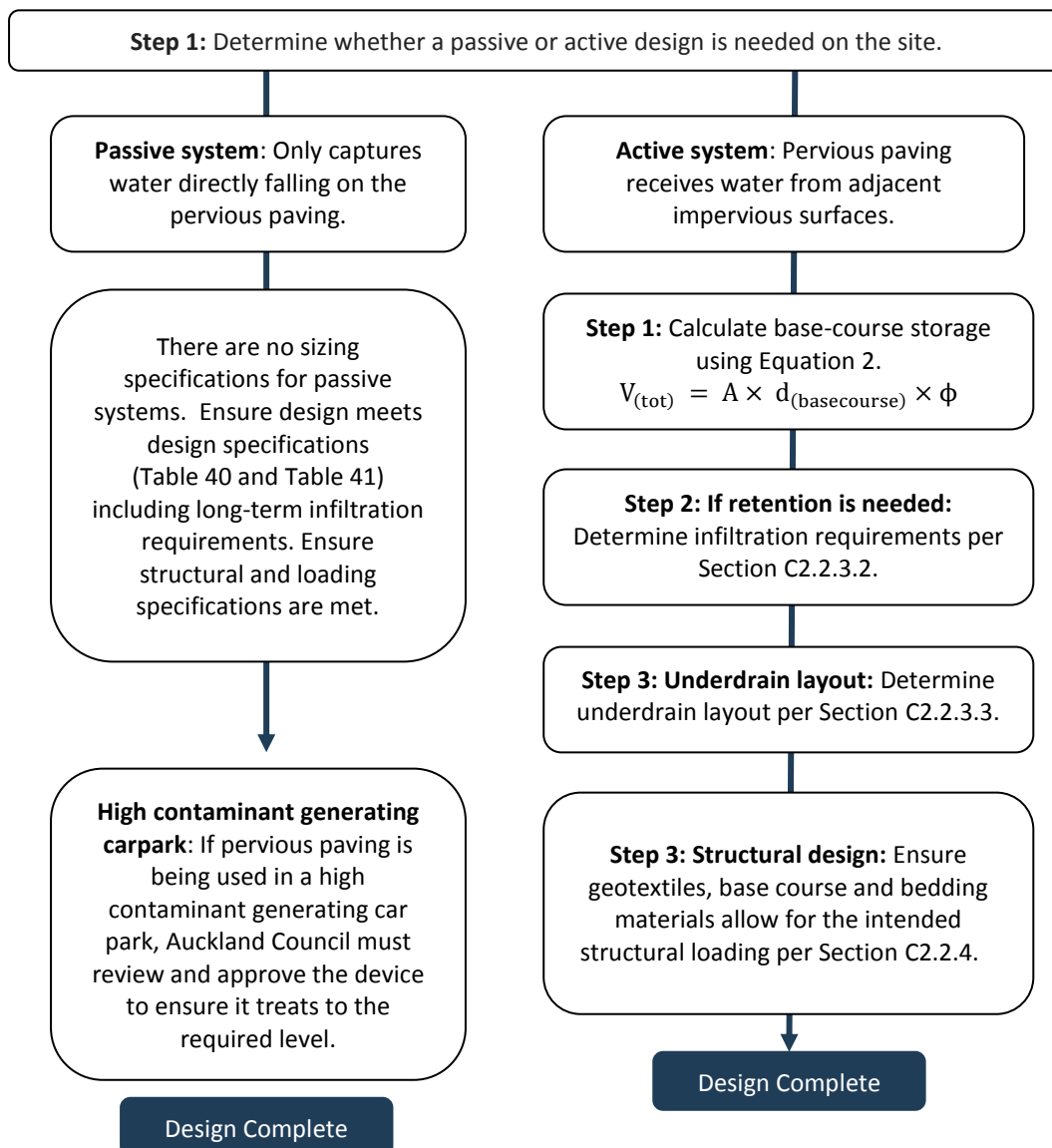
Figure 14: Pervious paving design flow chart
