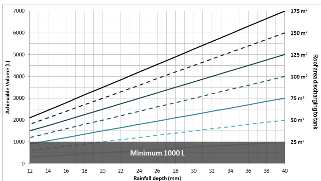
Figure 32: Total detention volume for impervious surface area 25 m 2 to 175 m 2 based on rainfall depth and connected area (for detention tank)
