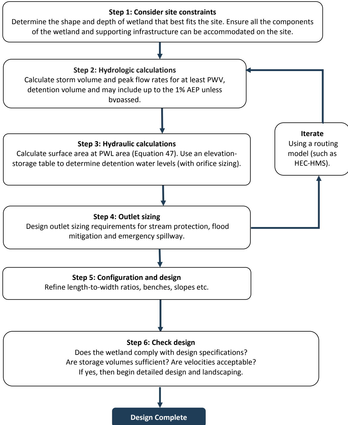
Figure 52: Constructed wetland design flow chart
