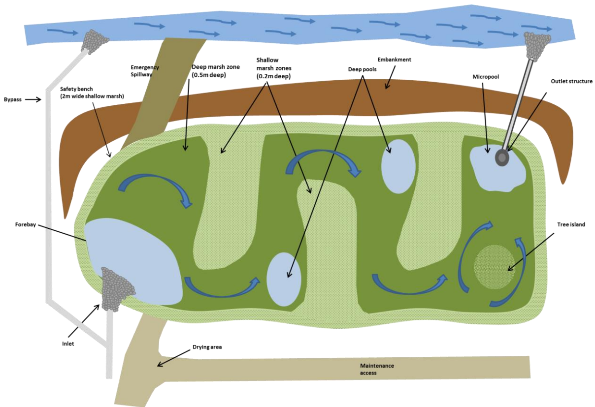
Figure 51: Example schematic of a sinuous bathymetry wetland
