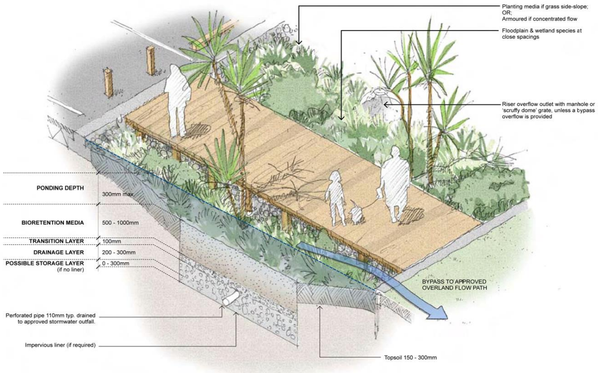
Figure 16: Schematic of rain garden cross-section
