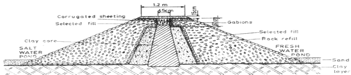
Fig.56: Embanked pens
