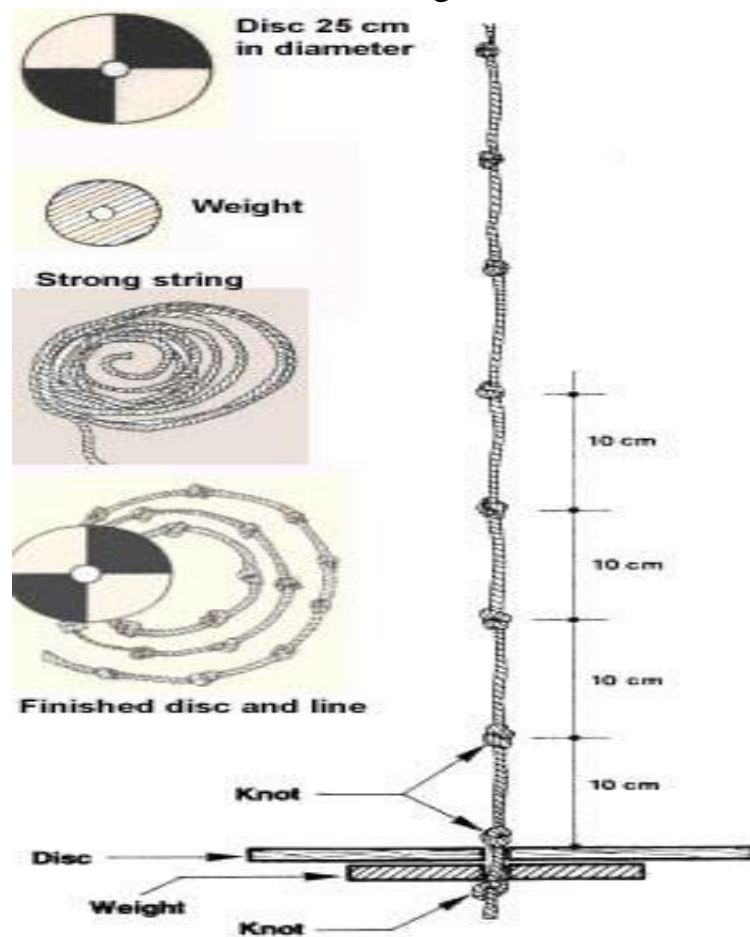
Fig. 15: Preparation of secchi disc
