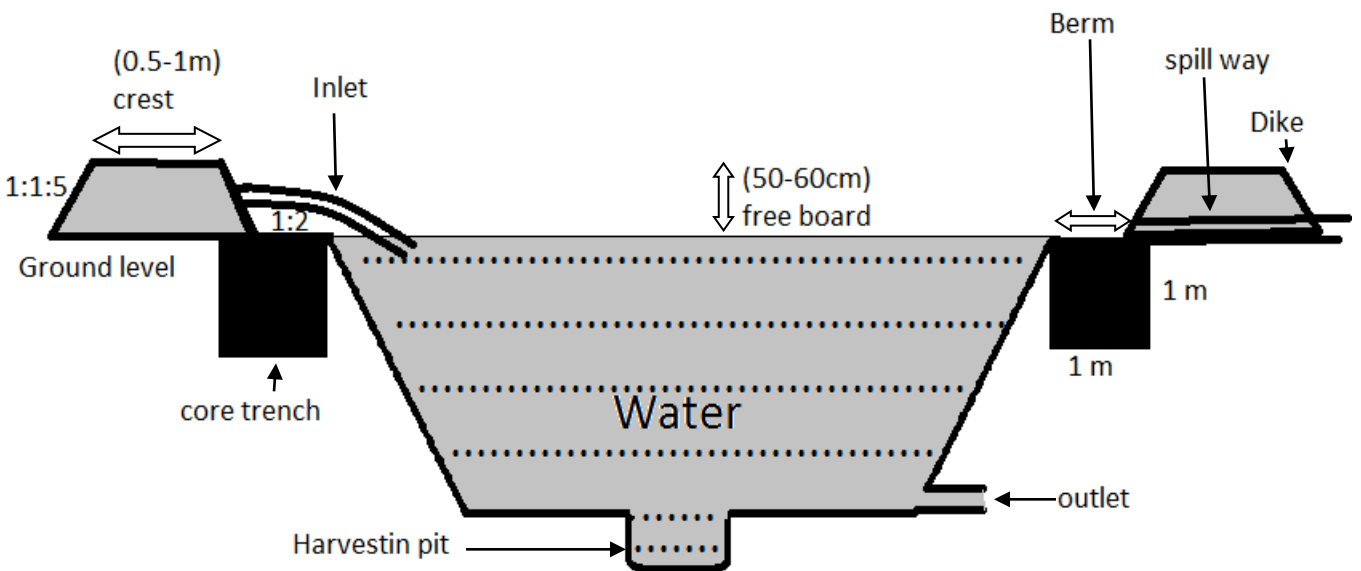
Fig.4: Cross section view of pond
