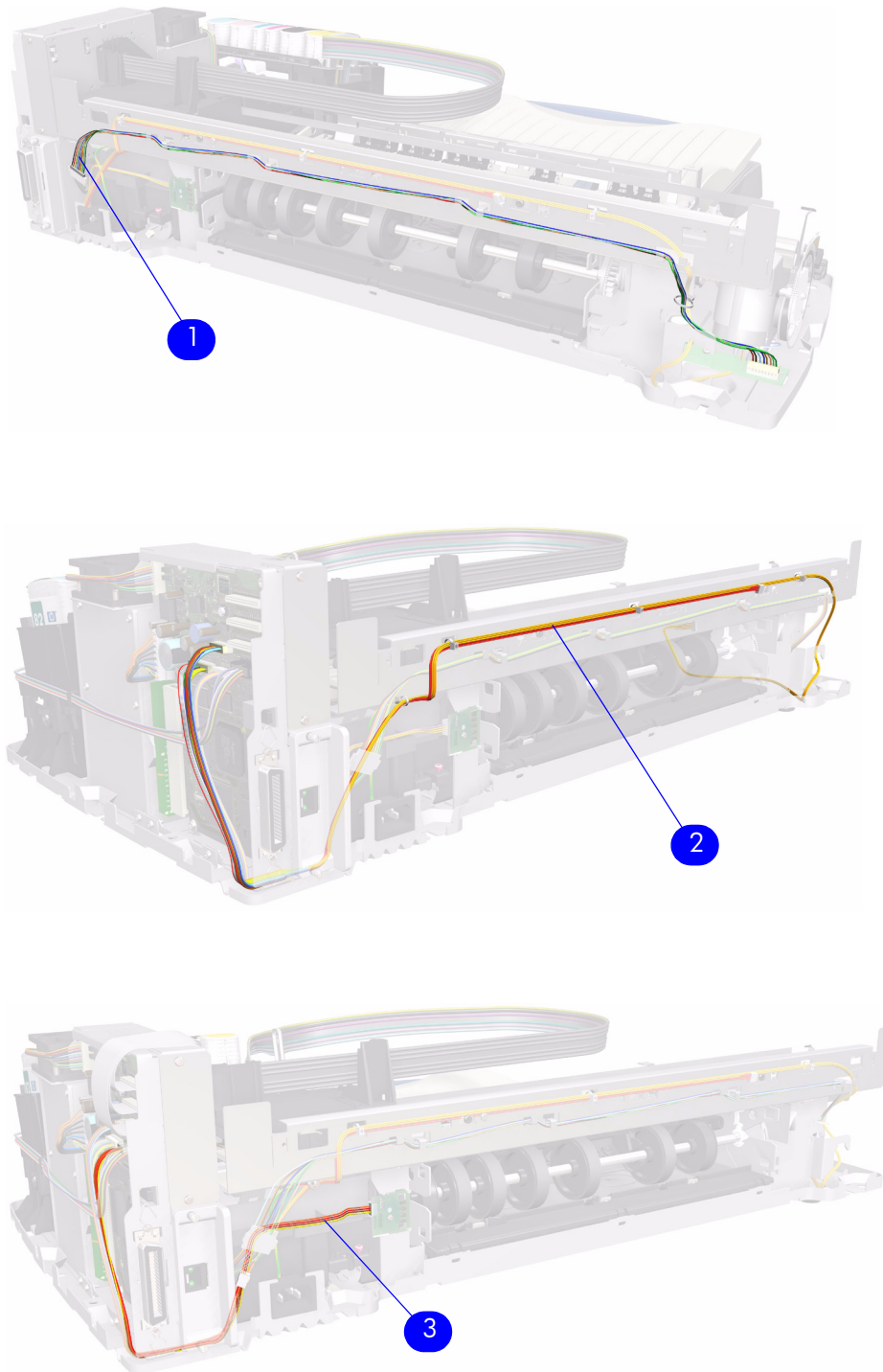
Figure 11: Cable Harnesses
