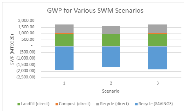
Fig. 8 GWP for Various SWM Scenarios
