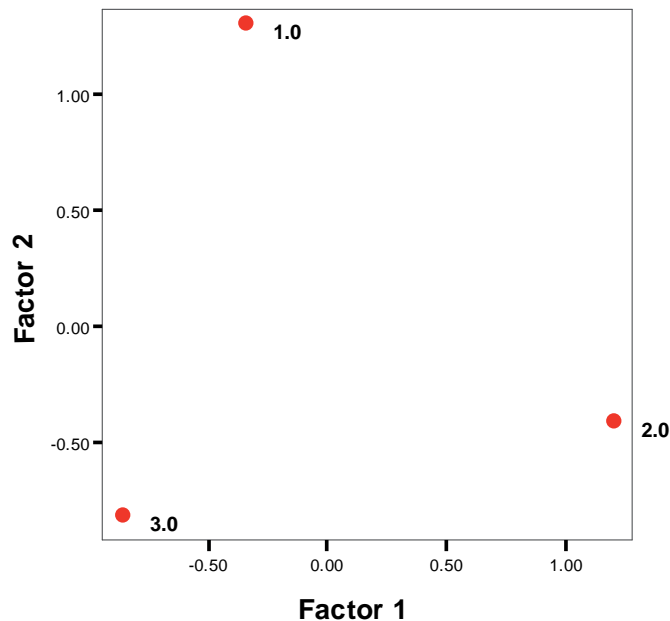
Figure 3.1 Factor analysis of mean abundance of fish families by site groupings in Shark Bay.
