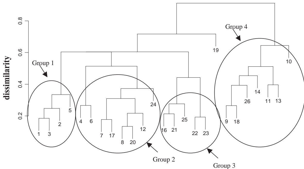
Figure 3.33 Divisive cluster analysis of Exmouth Gulf and Onslow invertibrate abundance data based on all three surveys.
