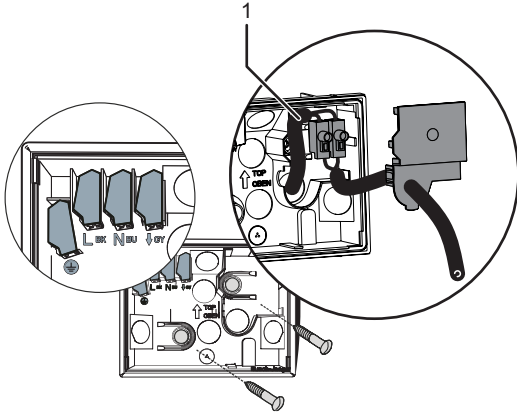
Fig. 10: Mounting the bottom of the device
