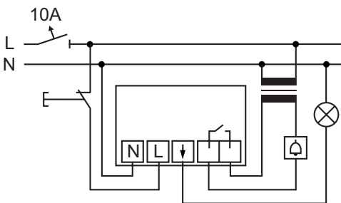
Fig. 12: Universal relay insert with external signal generators
