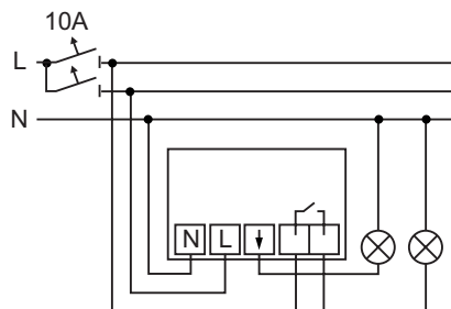
Fig. 13: Universal relay insert with 2 circuit breakers
