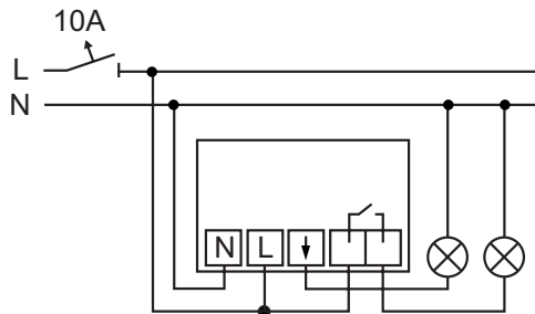
Fig. 11: Universal relay insert
