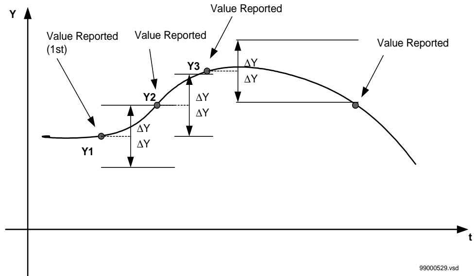
Figure 225: Amplitude dead-band supervision reporting
