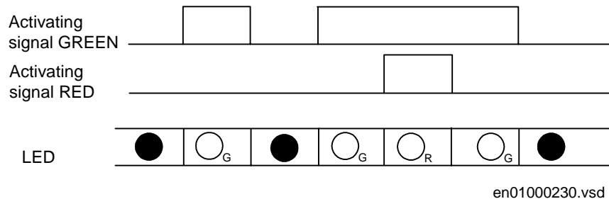
Figure 199: Operating sequence 1, two colors
