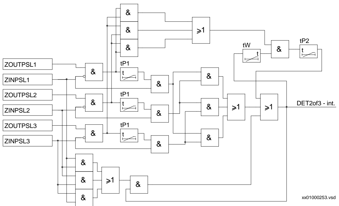
Figure 69: Simplified logic diagram for a two-out-of-three oscillation detection logic.
