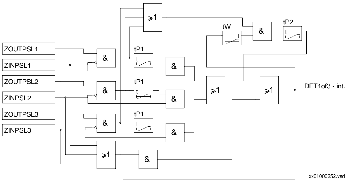
Figure 68: Simplified logic diagram for a one-out-of-three oscillation detection logic
