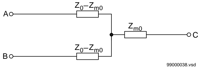
Figure 42: Equivalent zero sequence impedance circuit of the double-circuit, parallel, operating line with a single phase-to-earth fault at the remote busbar
