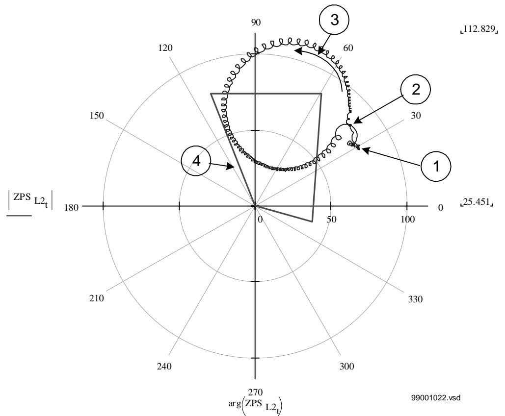
Figure 60: Impedance trajectory as seen by a L2-N impedance measuring element.
