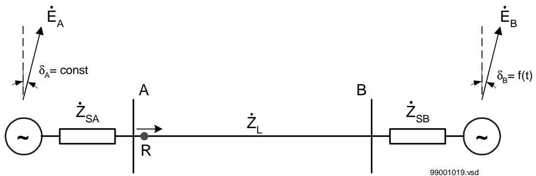
Figure 57: Two machine system.
