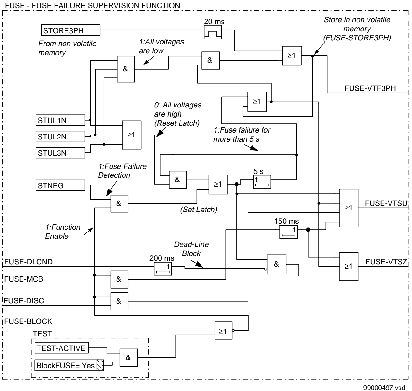
Figure 149: Simplified logic diagram for the fuse failure supervision function, negative sequence based.
