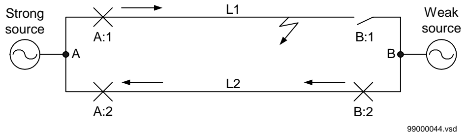
Figure 127: Current distribution after the breaker at B:1 is opened
