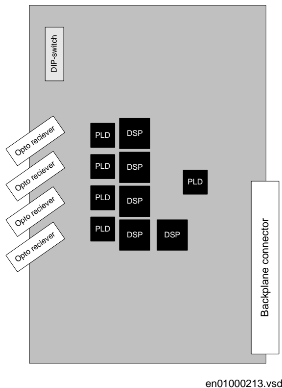
Figure 255: Block diagram for the ORM
