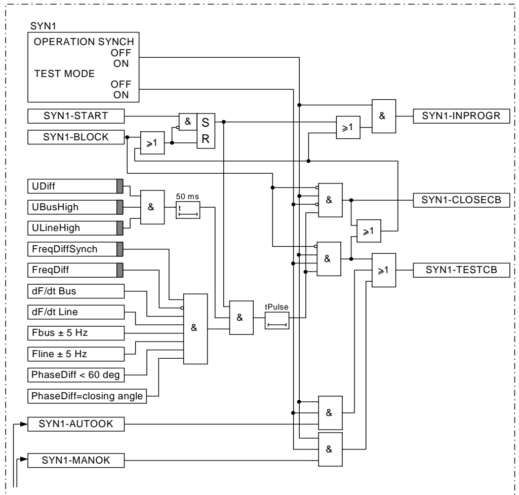
Figure 179: Simplified logic diagram - Phasing. The input signals SYN1-AUTOOK and SYN1-MANOK derive from the synchrocheck and energizing logic.
