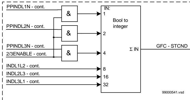
Figure 56: GFC start condition with phase preference
