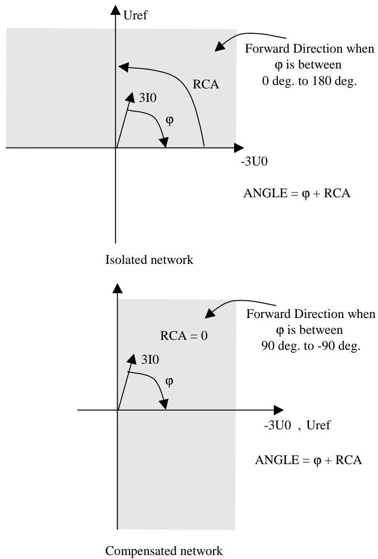
Figure 119: RCA with regard to compensated or isolated network
