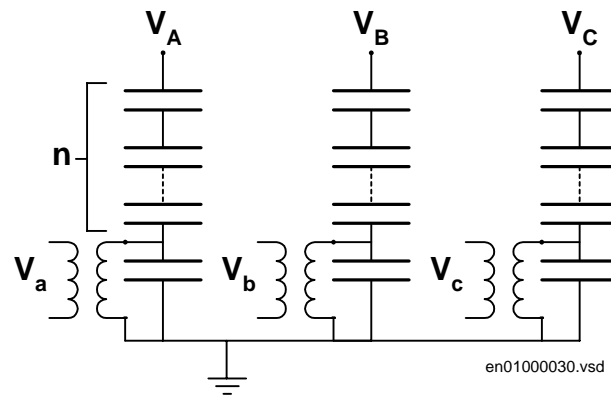
Figure 154: Capacitive voltage transformer
