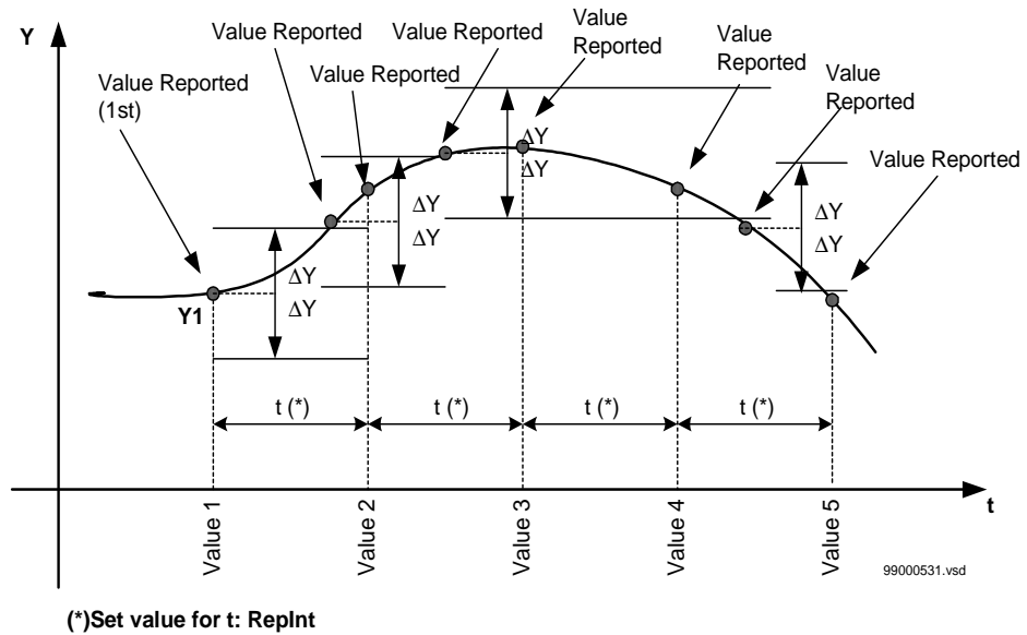
Figure 228: Periodic reporting with amplitude dead-band supervision in parallel.
