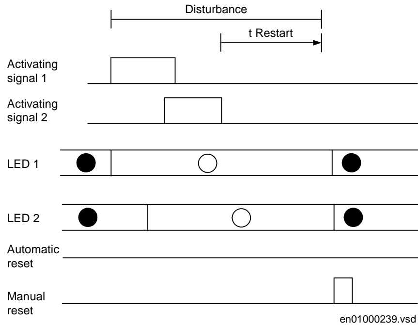
Figure 208: Operating sequence 6 (LatchedReset-S), two indications within same disturbance
