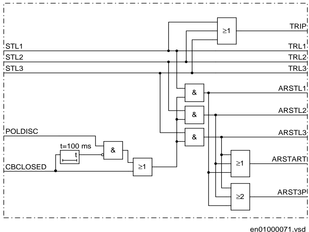
Figure 83: Trip and autorecloser start logic
