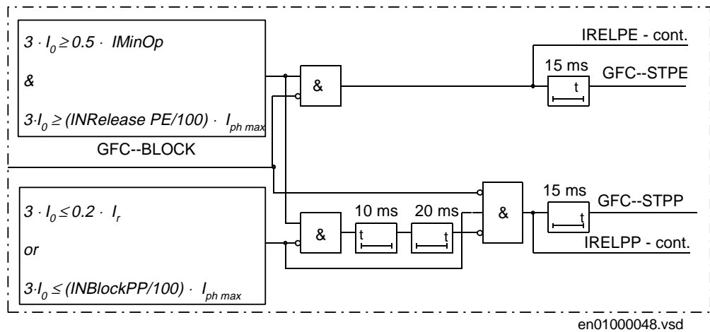
Figure 51: Detection of ph-E and ph-ph fault conditions
