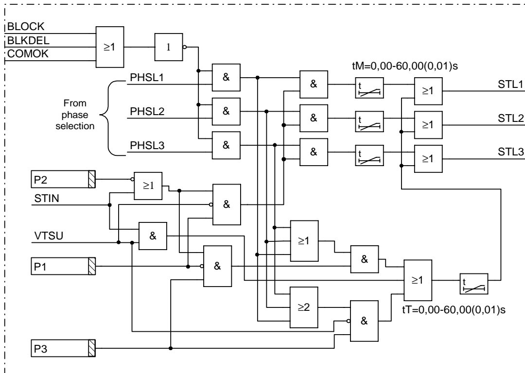
Figure 81: Function for delayed fault clearing
