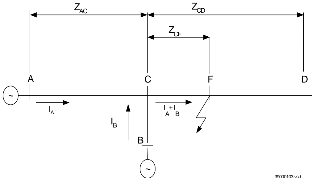
Figure 39: Network with line tied at an intermediate location
