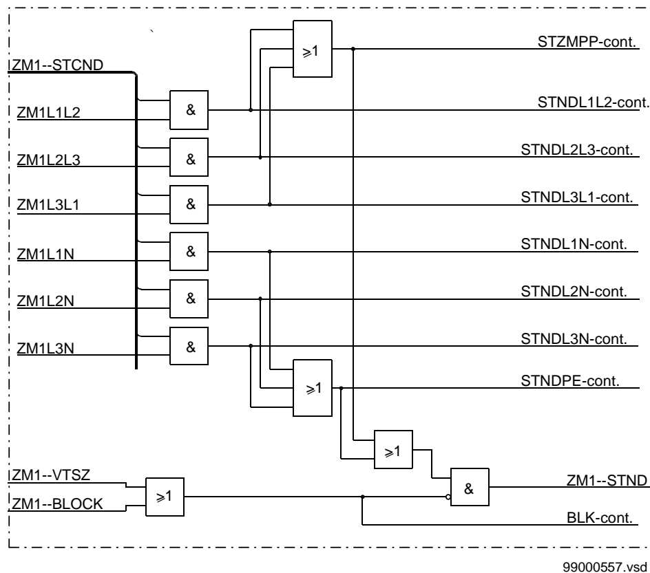
Figure 35: Conditioning by a group functional input signal ZM1--STCND
