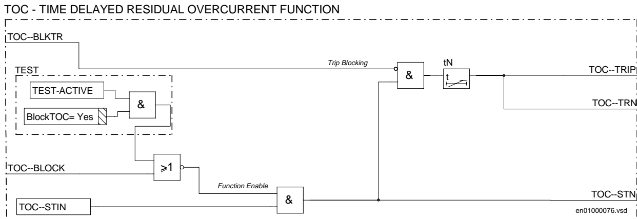
Figure 95: Simplified logic diagram of the TOC-- protection function.
