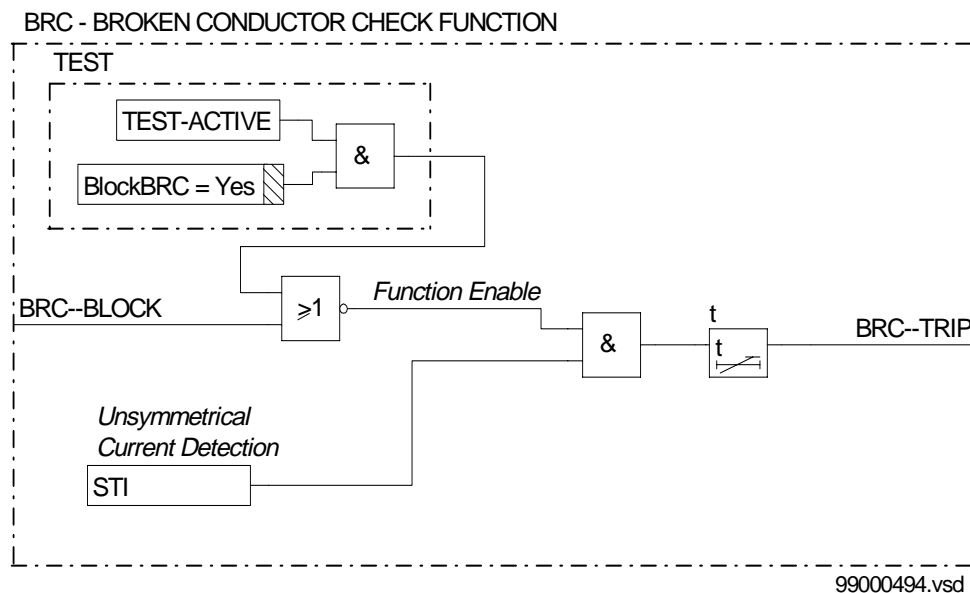
Figure 143: Simplified logic diagram of broken conductor check function
