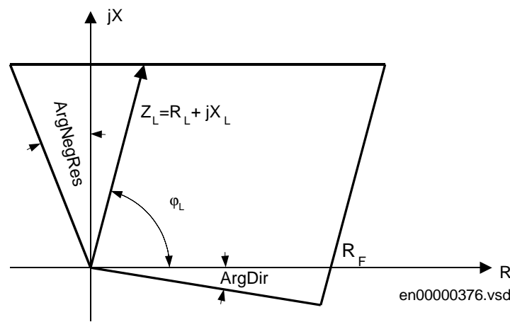
Figure 29: Typical characteristic of a distance protection zone.
