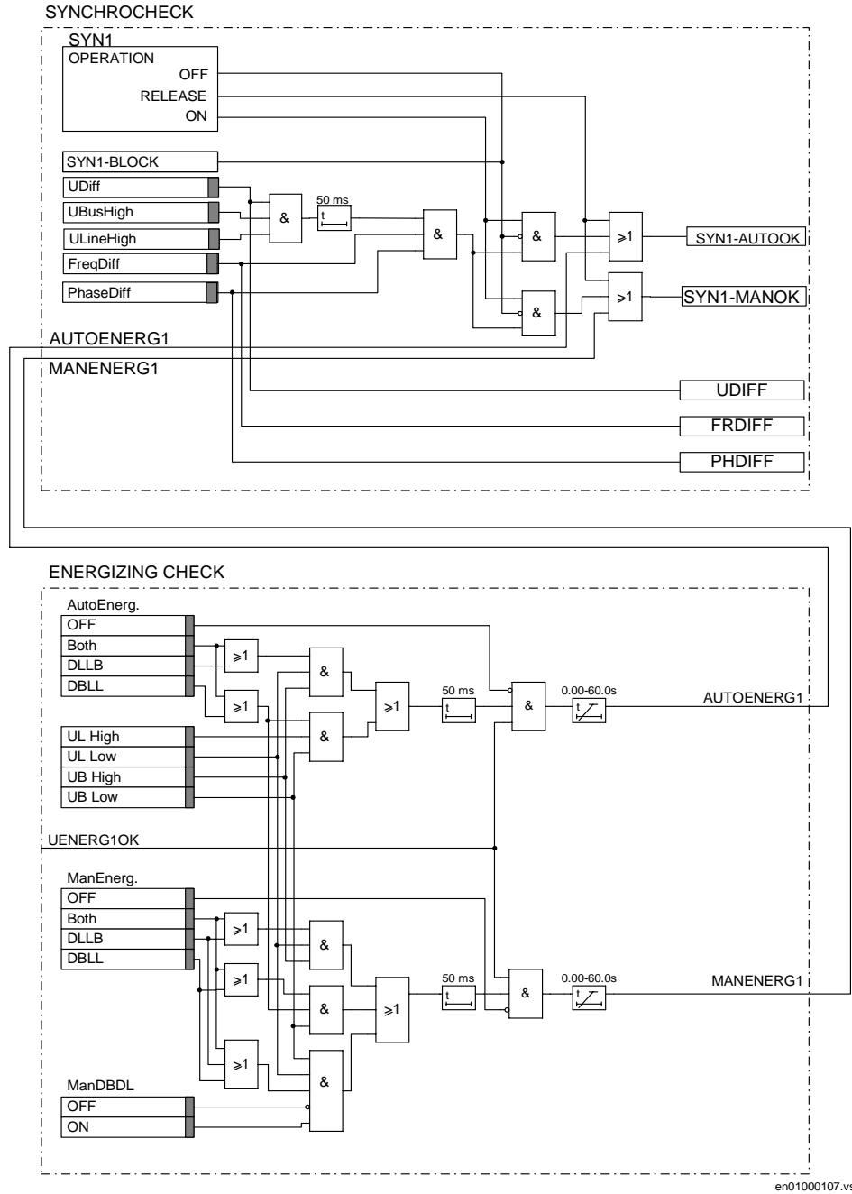
Figure 170: Simplified logic diagram - Synchrocheck and energizing check. The internal signal UENERG1OK refers to the voltage selection logic.
