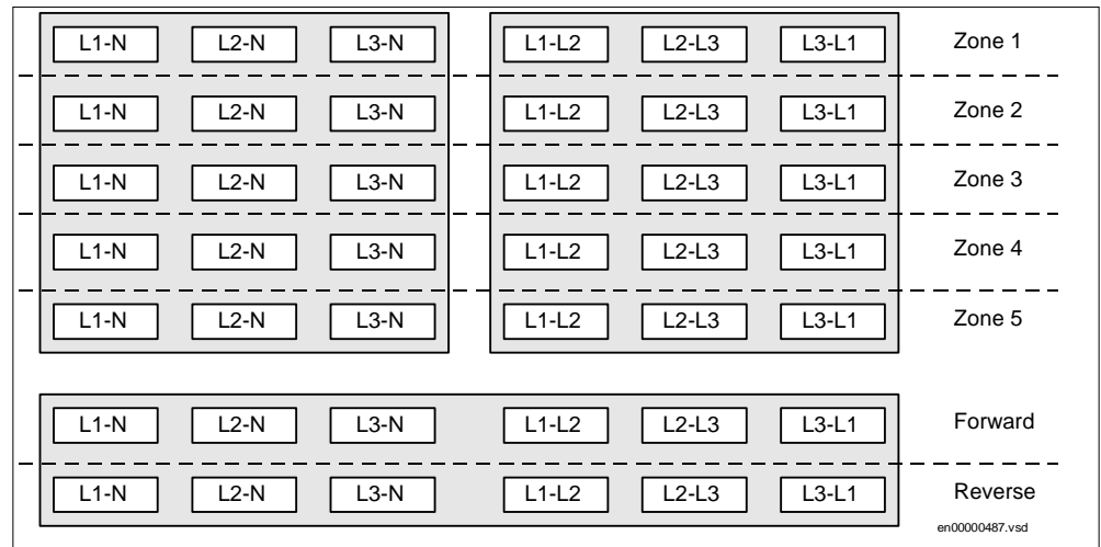
Figure 34: Location of different measuring loops within the three digital signal processors
