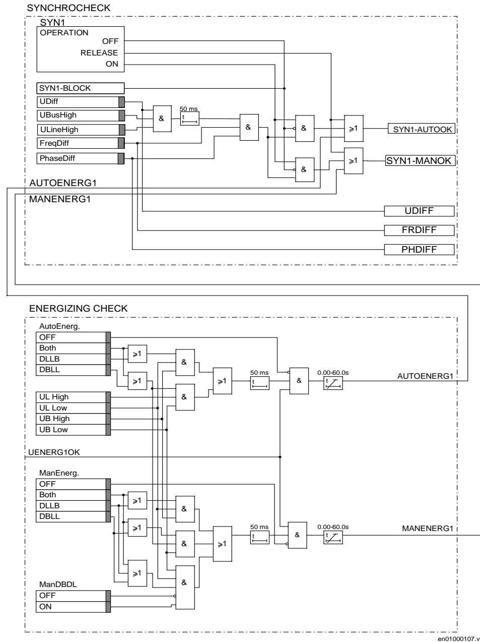
Figure 176: Simplified logic diagram - Synchrocheck and energizing check. The internal signal UENERG1OK refers to the voltage selection logic.
