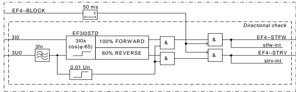
Figure 110: Simplified logic diagram of internal function Directional check.
