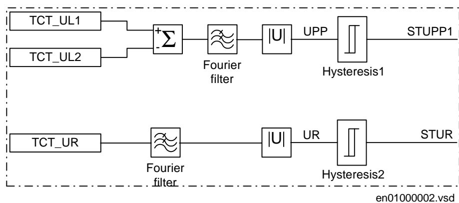
Figure 152: Phase-to-phase voltage and residual voltage measurement
