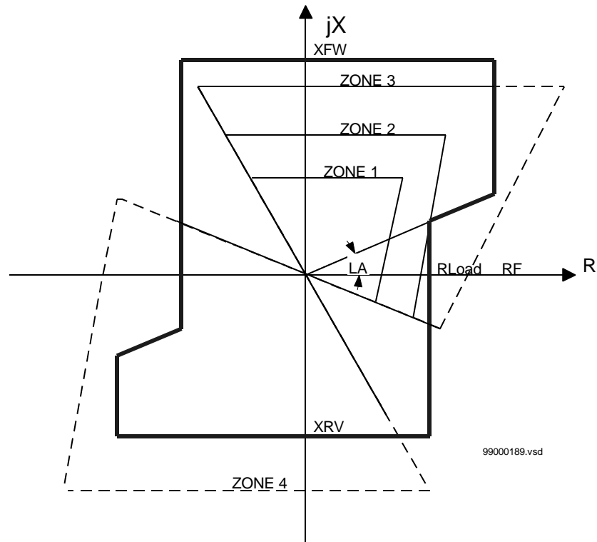
Figure 50: Operating characteristics of the GFC (impedance measuring principle) and zone measuring elements
