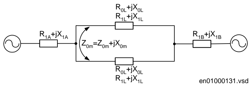
Figure 215: Simplified network configuration with network data, required for settings of the fault location-measuring function.
