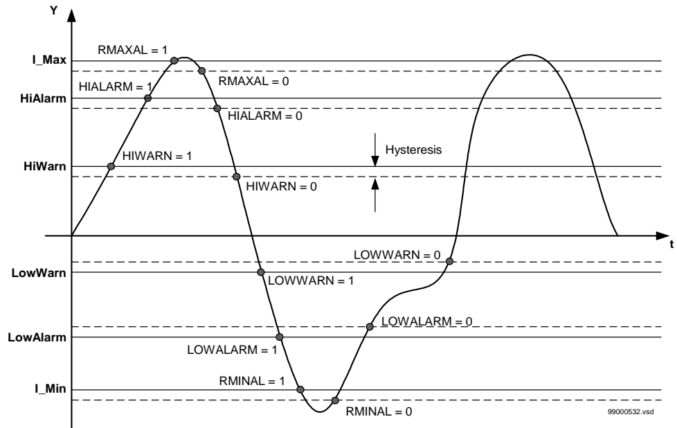
Figure 224: Presentation of the operating limits
