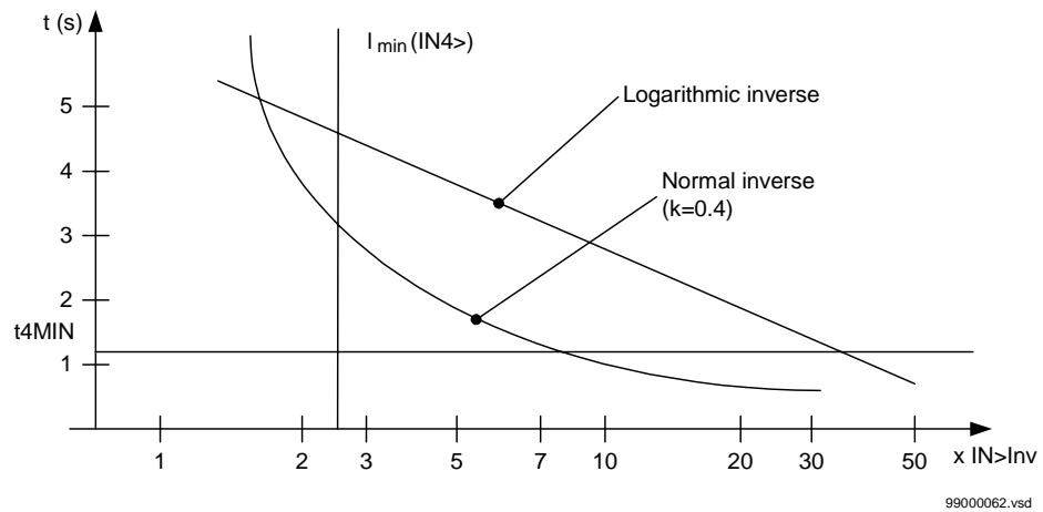
Figure 112: Normal inverse and logarithmic inverse time characteristics.
