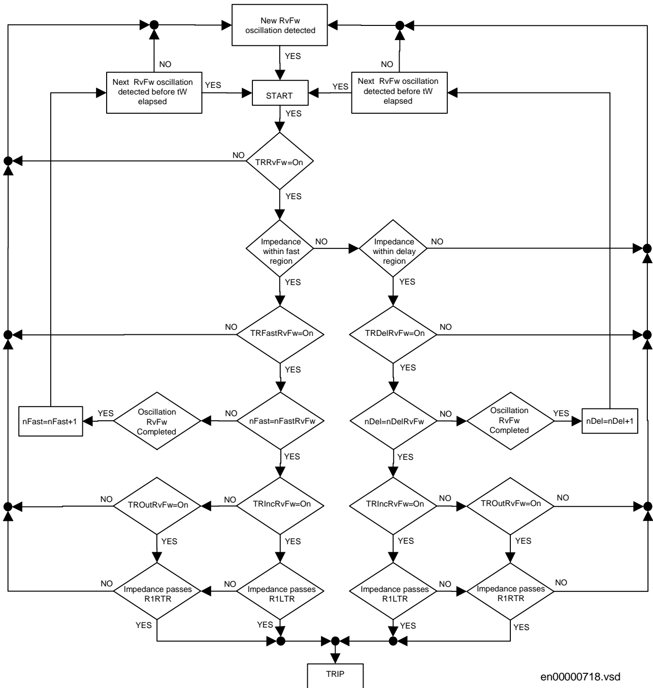
Figure 73: Flow-chart presenting the operation of the pole slip protection for the reverse to forward transition (RvFw) after the oscillation has been detected.
