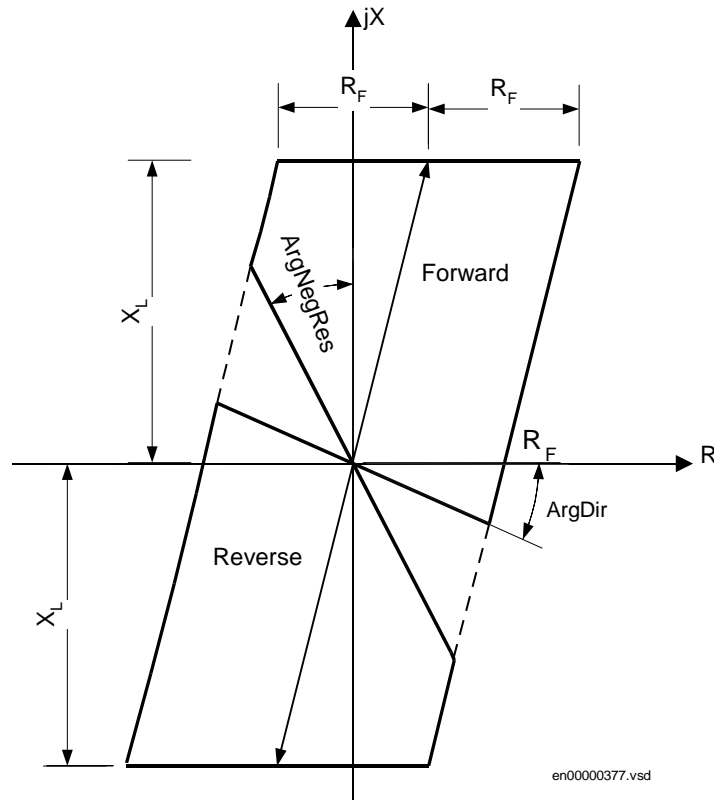
Figure 30: Nondirectional and directional (forward and reverse) operating characteristic
