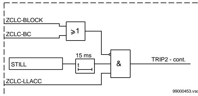
Figure 49: Loss-of-load acceleration - simplified logic diagram
