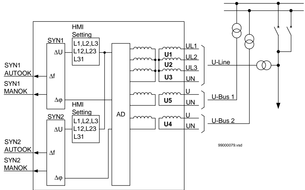
Figure 161: Connection of the synchrocheck function for one bay.
