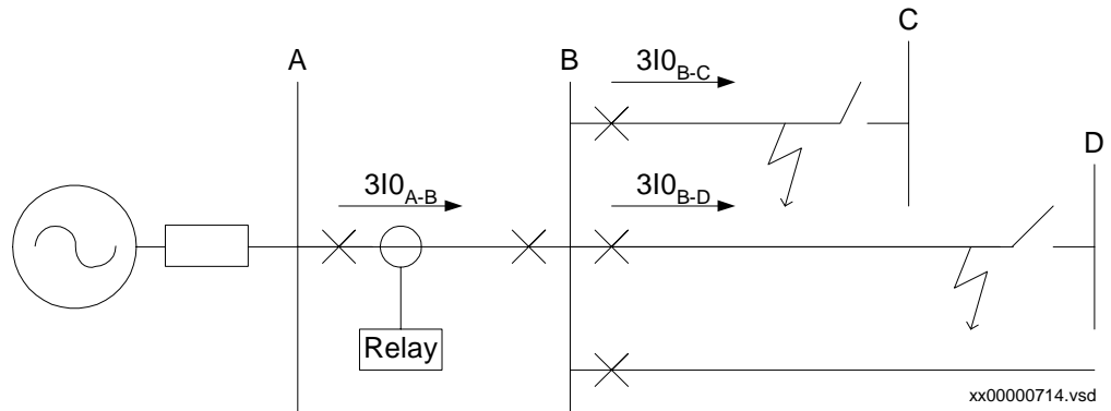
Figure 117: Example of fault cases between stations. Calculation of 3I0_{min} for step 2 (and step 3).
