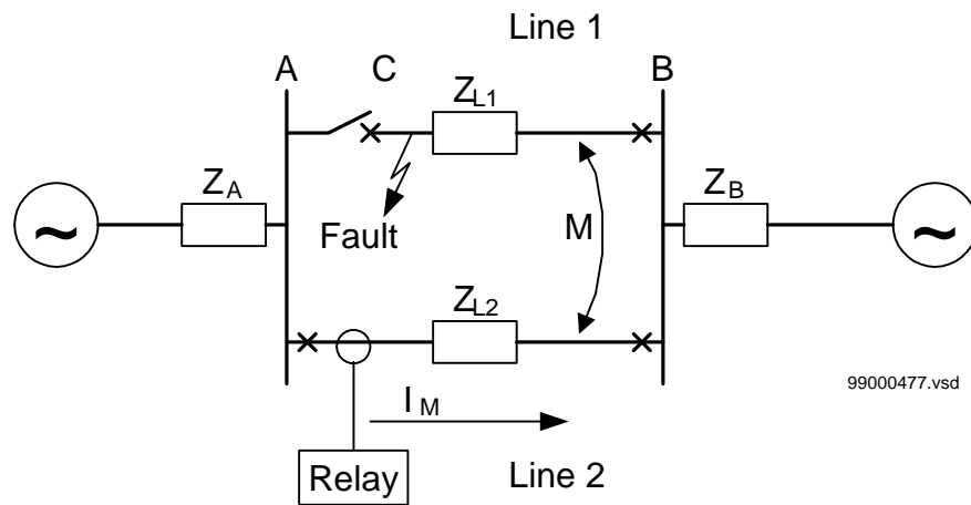
Figure 93: Two parallel lines. Influence from parallel line to the through fault current: I_M .
