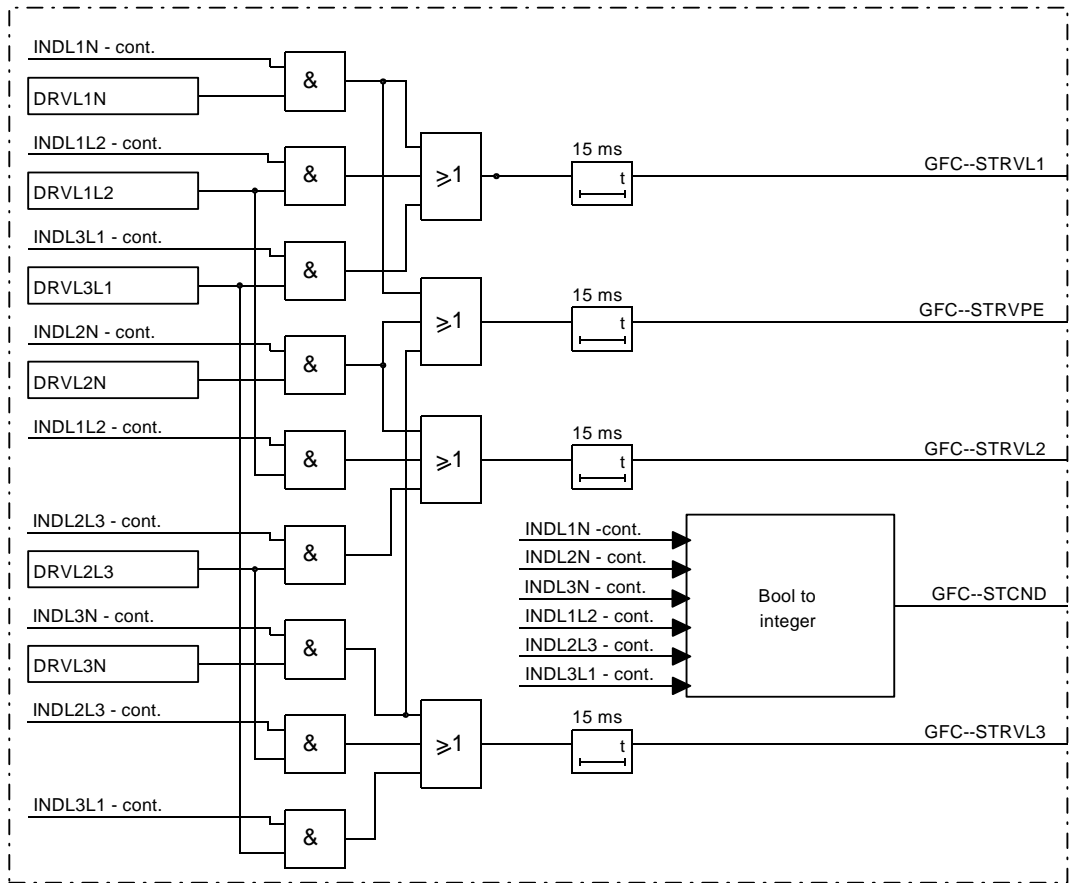
Figure 54: Composition of reverse directed GFC signals and measured impedance related zone starting conditions
