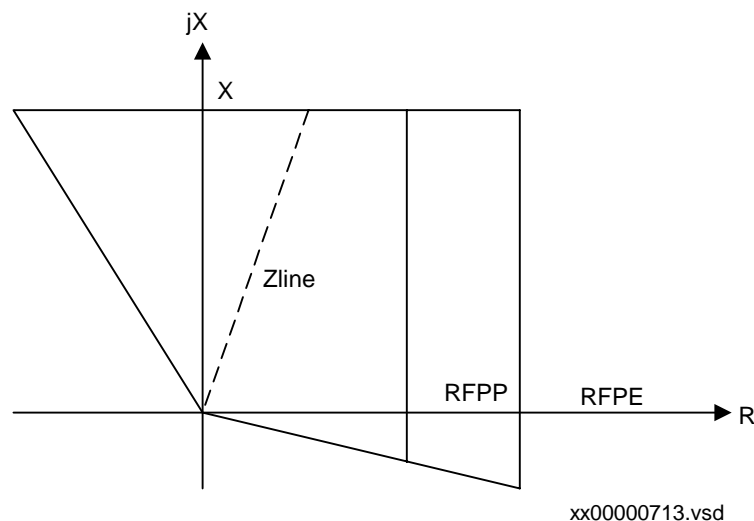
Figure 46: Simplified operating characteristic with R1PP or (R1PE and R0PE) or (R1 and R0 with simplified setting parameters) are set to their minimum values
