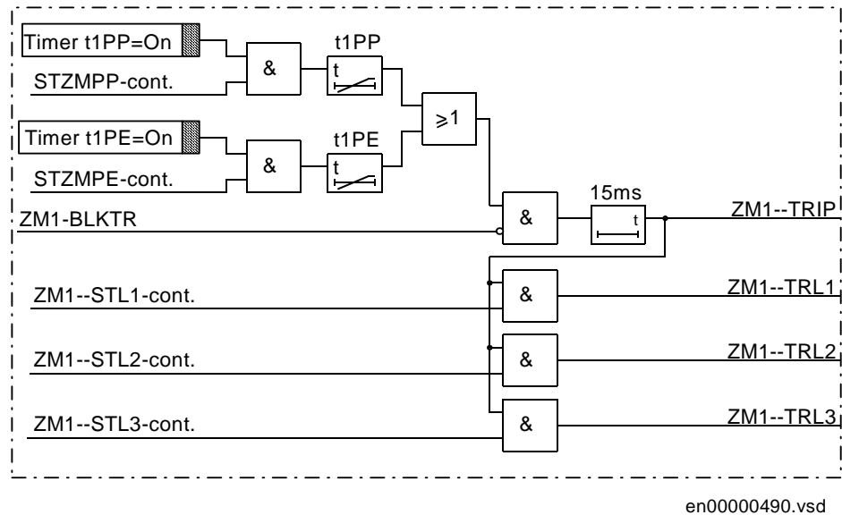
Figure 38: Tripping logic for the distance protection zone one
