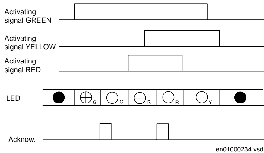
Figure 203: Operating sequence 3, three colors involved, alternative 2
