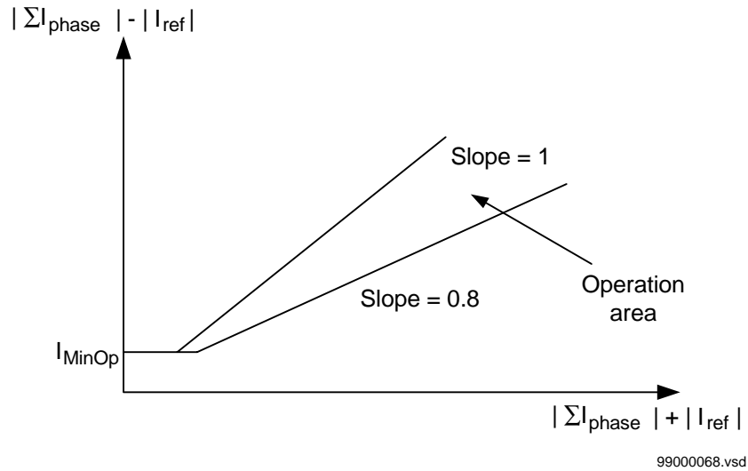
Figure 148: Operate characteristics
