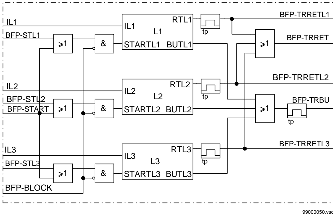
Figure 139: Breaker-failure protection
