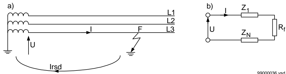
Figure 40: Equivalent circuits for measurement at single-phase-to-earth faults.
