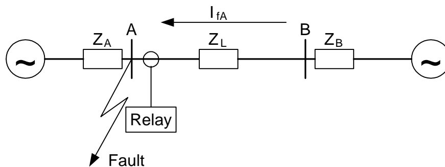
Figure 115: Through fault current from B to A: I_{fA}
