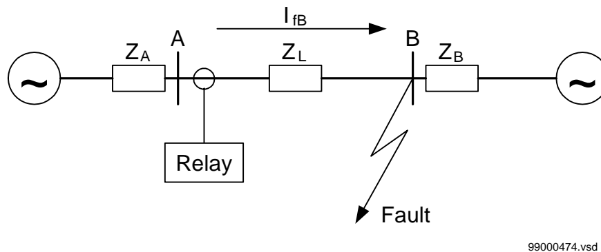
Figure 113: Through fault current from A to B: I_{fB}
