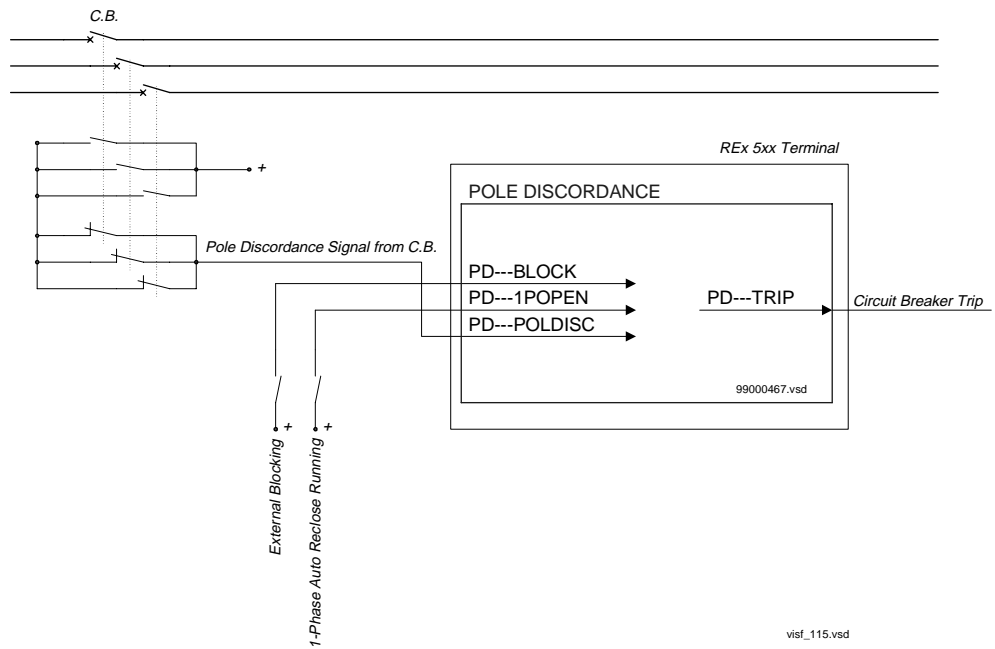
Figure 187: Typical connection diagram for pole discordance function - contact based
