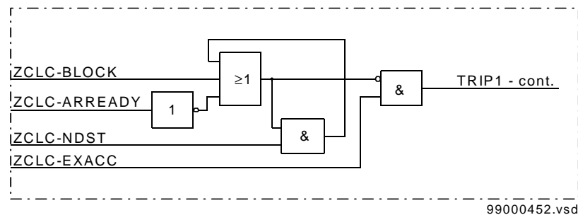
Figure 48: Simplified logic diagram for the local acceleration logic
