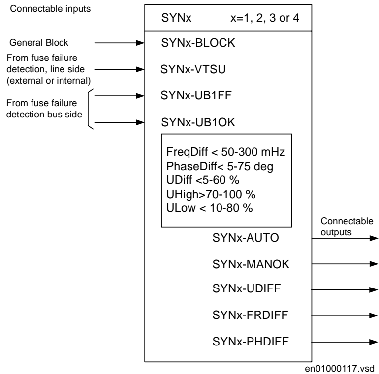
Figure 172: Input and output signals.
