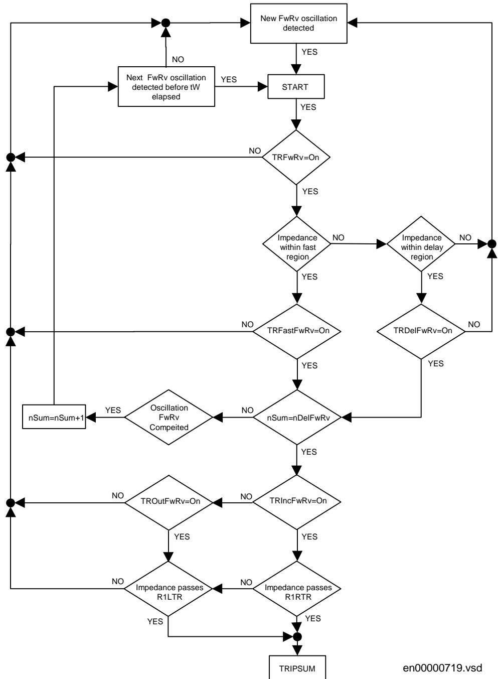
Figure 74: Flow-chart presenting summation trip (TRIPSUM) of the pole slip protection for the forward to reverse transition (FwRv).
