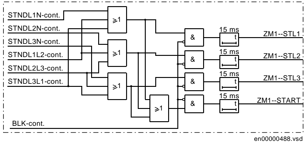
Figure 36: Composition of starting signals in non-directional operating mode
