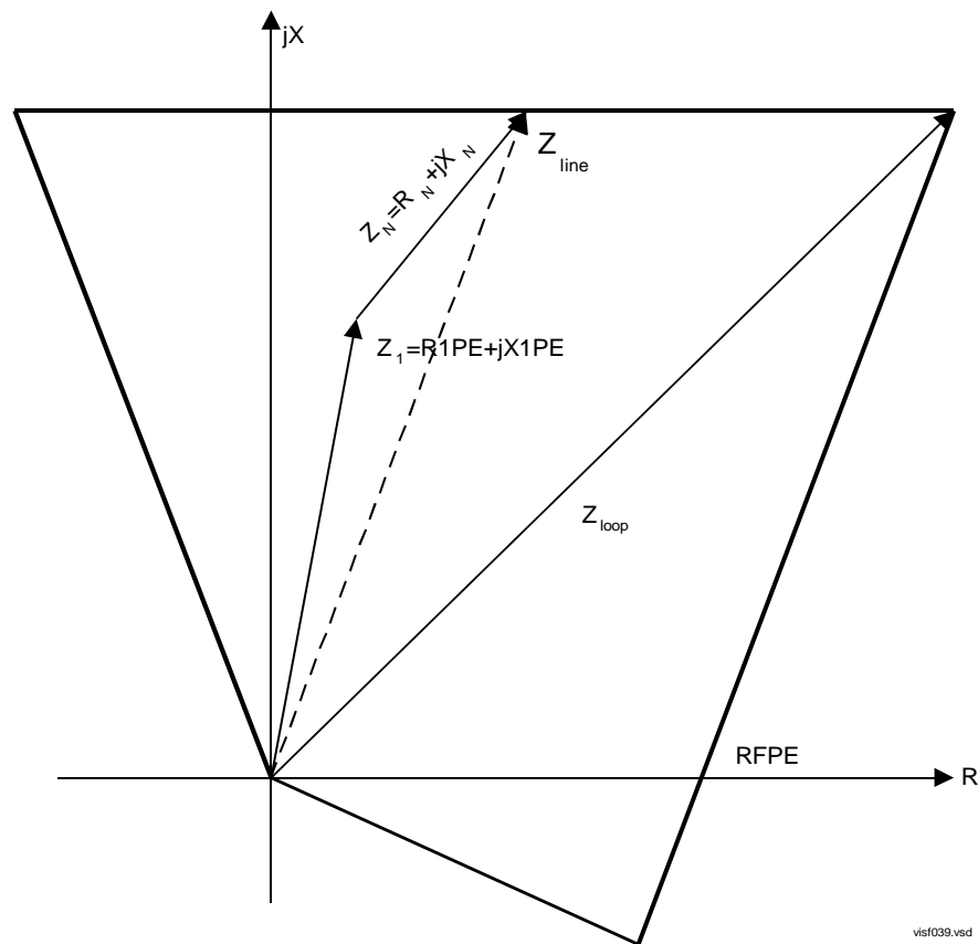
Figure 31: Characteristic of the phase-to-earth measuring loop.
