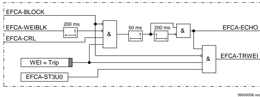
Figure 131: Simplified logic diagram, weak end infeed - Trip.
