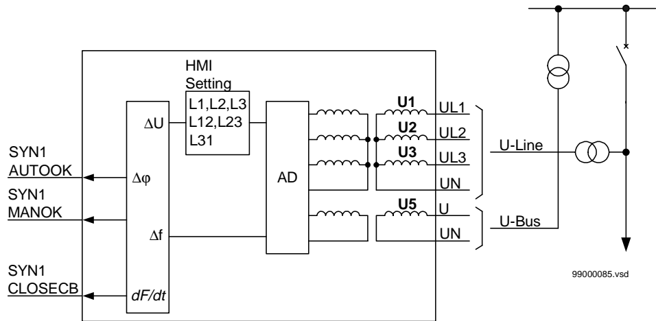
Figure 164: Connection of the phasing and synchrocheck function for one bay.
