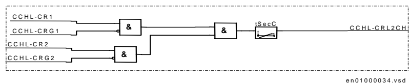
Figure 192: Combination of two communication channels
