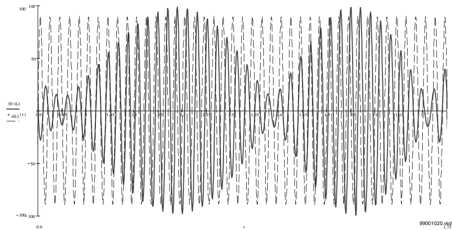
Figure 58: Current (solid line) and voltage (dashed line) in relay point during the pole slip condition.
