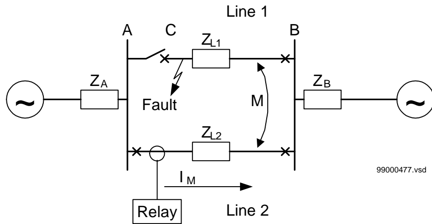
Figure 89: Two parallel lines. Influence from parallel line to the through fault current: I_M
