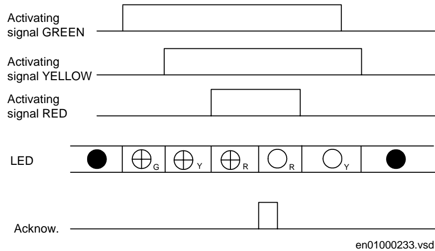
Figure 202: Operating sequence 3, three colors involved, alternative 1
