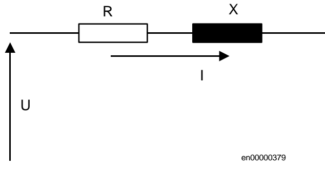
Figure 32: Apparent impedance with resistance and reactance connected in series
