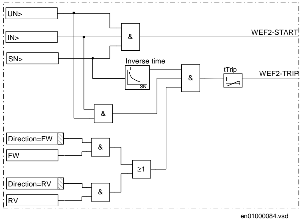
Figure 122: Logic for sensitive directional residual power protection function (WEF2)
