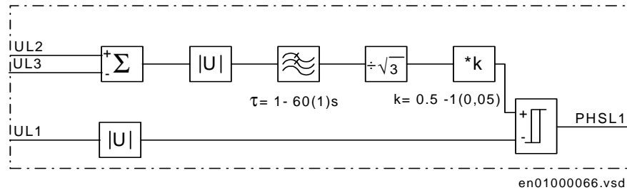
Figure 77: Phase selection function
