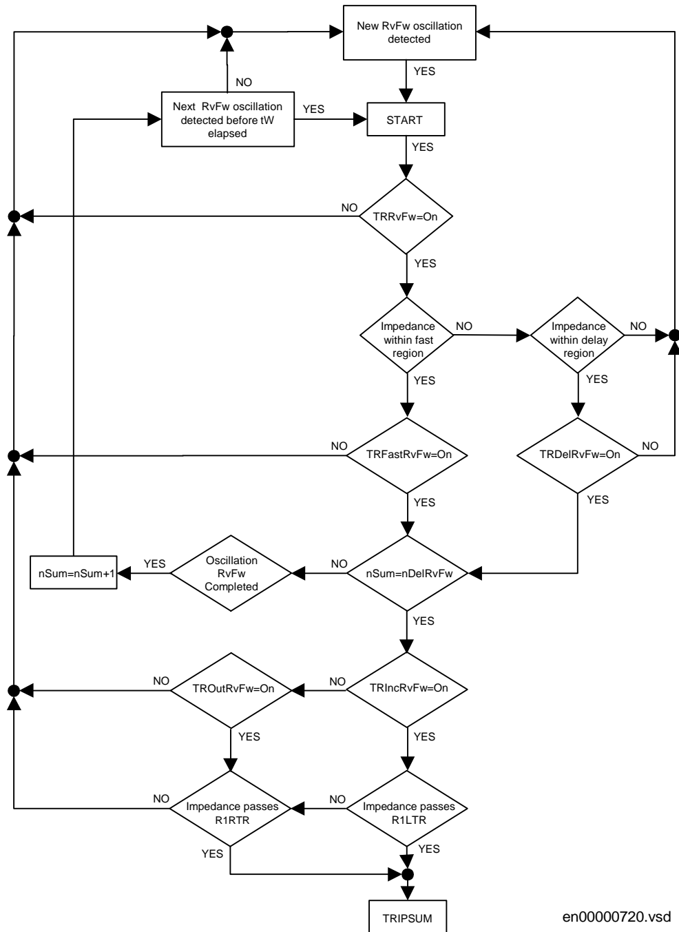
Figure 75: Flow-chart presenting summation trip (TRIPSUM) of the pole slip protection for the reverse to forward transition (RvFw).
