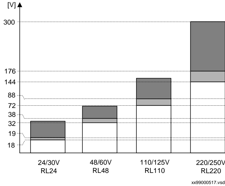
Figure 258: Voltage dependence for the binary inputs
