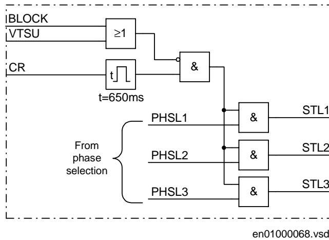
Figure 80: Function for fast fault clearing
