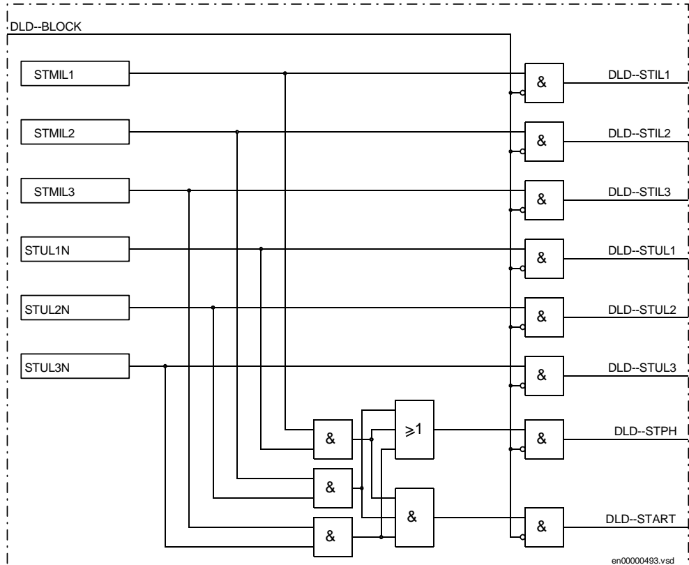
Figure 146: DLD - simplified logic diagram of the dead line detection function
