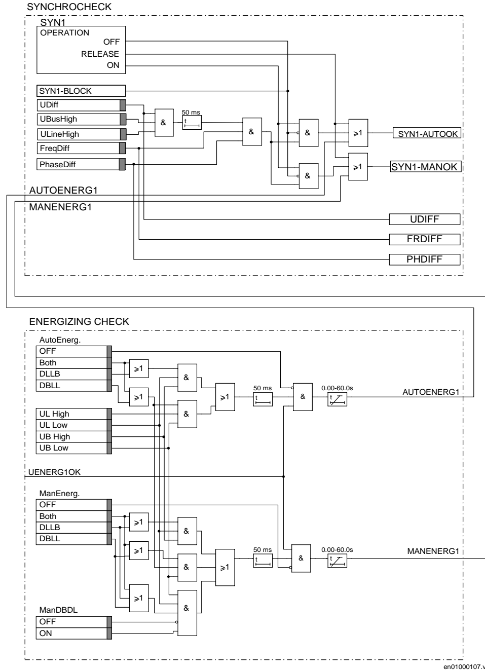
Figure 180: Simplified logic diagram - Synchrocheck and energizing check for one circuit breaker. The internal signal UENERG1OK derives from the external or internal fuse failure inputs SYN1-UB1OK/FF and SYN1-VTSU.
