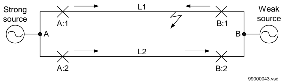
Figure 126: Initial condition
