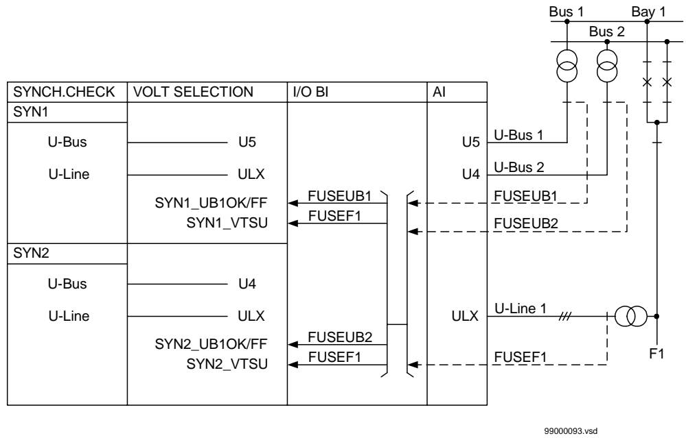
Figure 168: Voltage connection in a double breaker arrangement.
