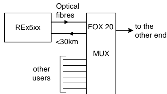
Figure 235: Dedicated link, optical fibre connection.
