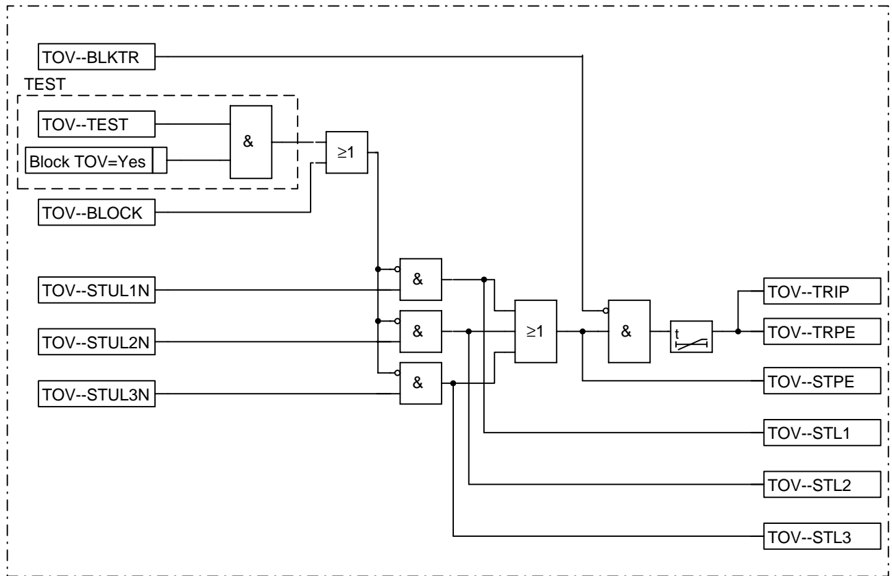
Figure 141: Logic diagram, time delayed overvoltage protection, phase wise
