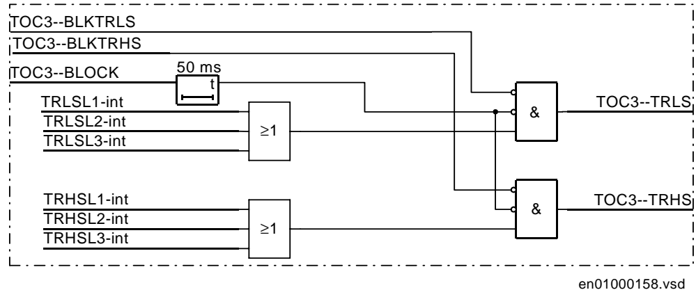
Figure 102: General trip
