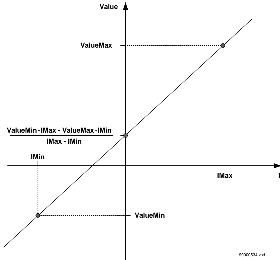
Figure 232: Relationship between the direct current ( I ) and the measured quantity primary value ( Value )
