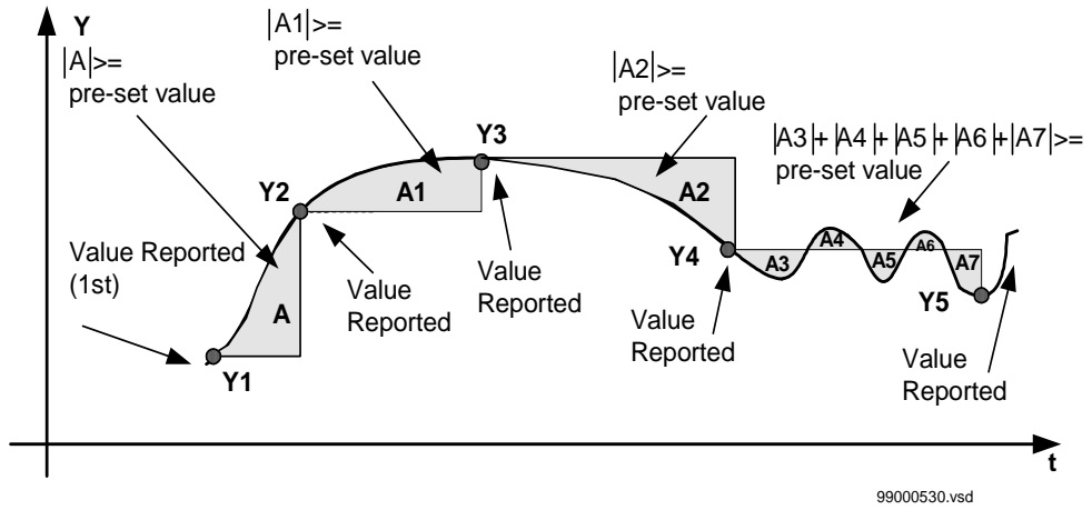
Figure 226: Reporting with integrating dead-band supervision
