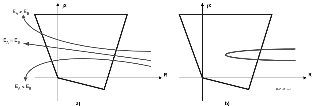
Figure 59: Impedance trajectories in relay point during the pole slip (figure a) and power swing (figure b) phenomena.
