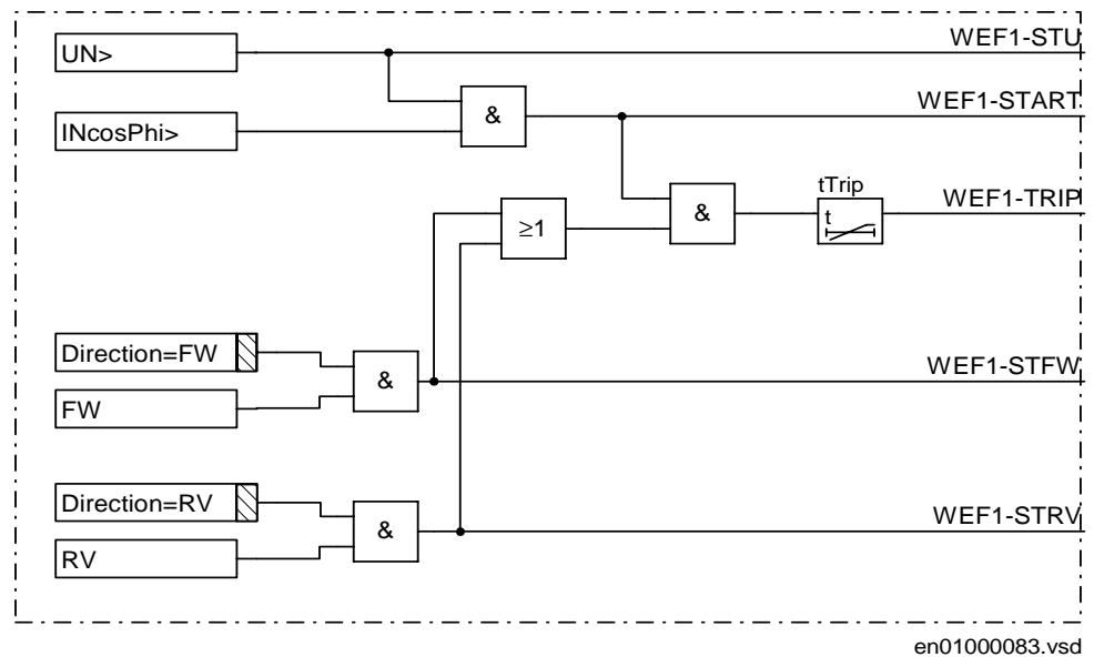
Figure 120: Logic for sensitive directional residual overcurrent protection function (WEF1)
