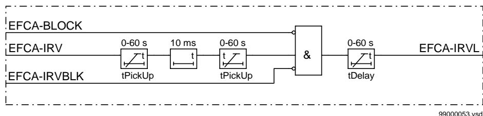
Figure 132: Simplified logic diagram, current reversal
