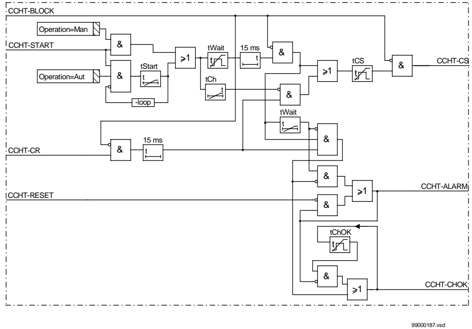
Figure 194: Simplified logic diagram for the CCHT function
