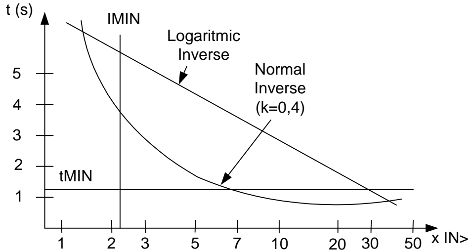
Figure 105: Normal inverse and logarithmic inverse time characteristics.
