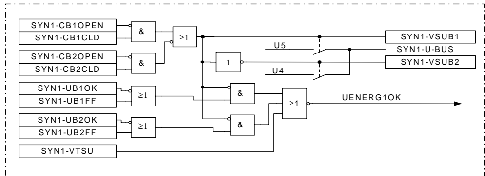
Figure 177: Simplified voltage selection logic in a double bus, single breaker arrangement.
