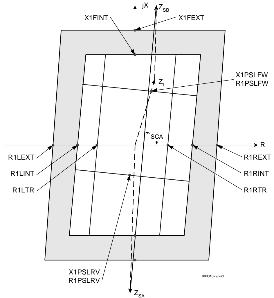
Figure 67: Operating characteristic of the pole slip protection with corresponding settings in the impedance plane.
