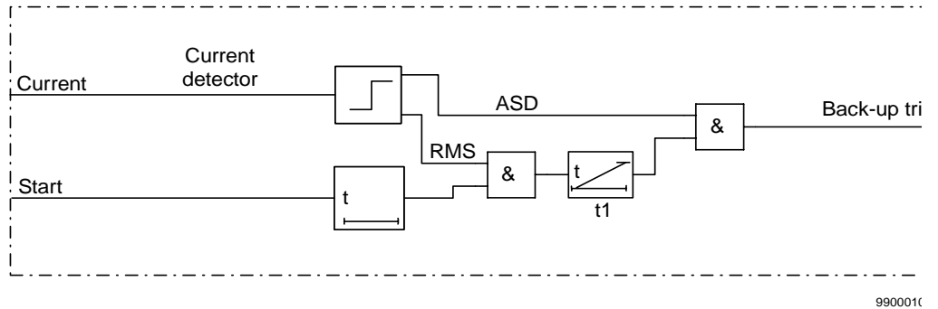
Figure 137: Breaker-failure protection
