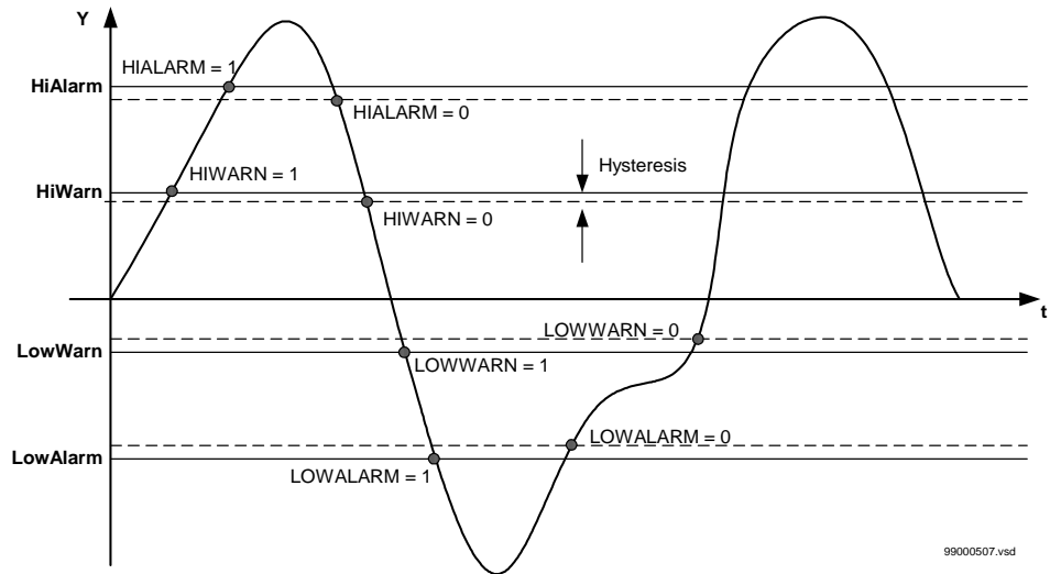
Figure 216: Presentation of the operating limits.
