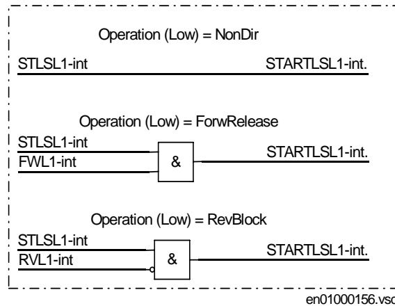
Figure 100: Directional operation modes of TOC3
