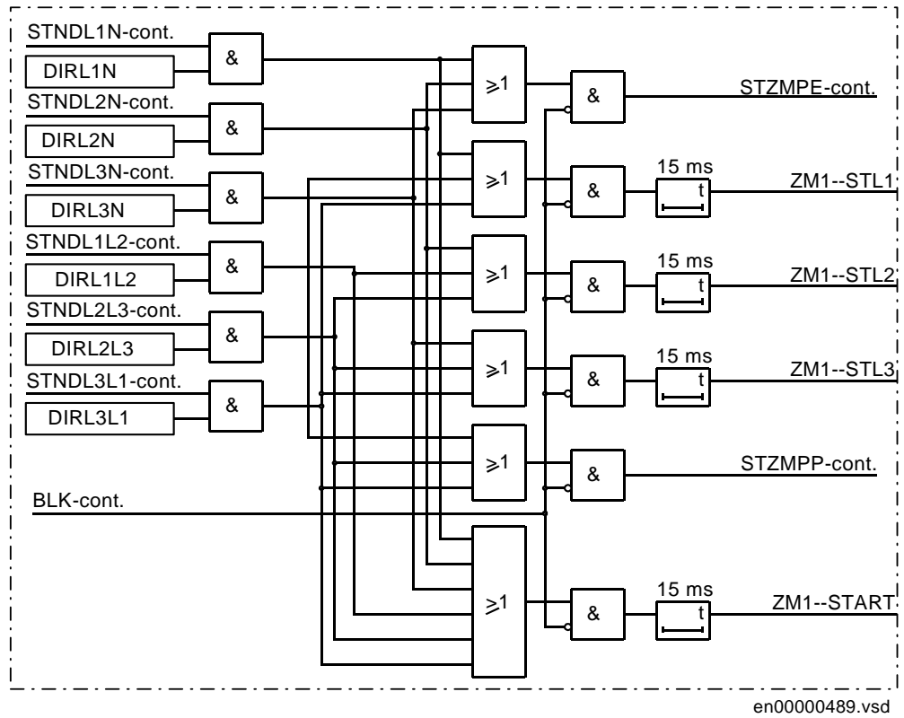
Figure 37: Composition of starting signals in directional operating mode
