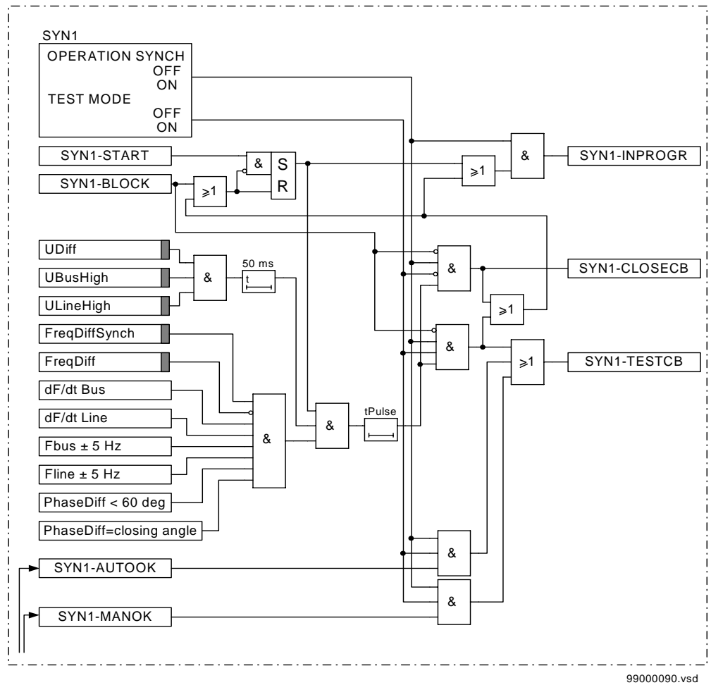
Figure 175: Simplified logic diagram - Phasing. The input signals SYN1-AUTOOK and SYN1-MANOK derive from the synchrocheck and energizing logic.
