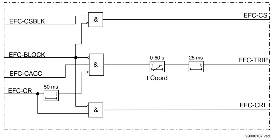
Figure 124: Simplified logic diagram, Scheme type = blocking
