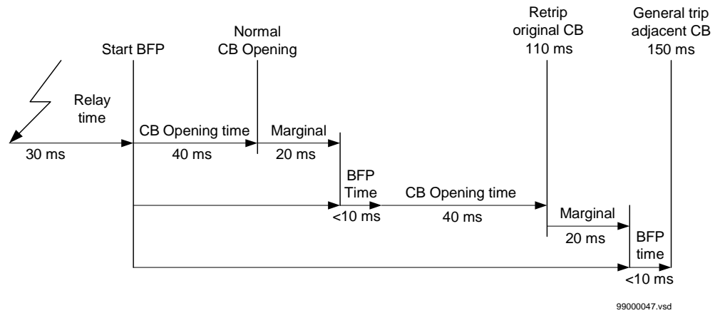
Figure 134: Time sequence
