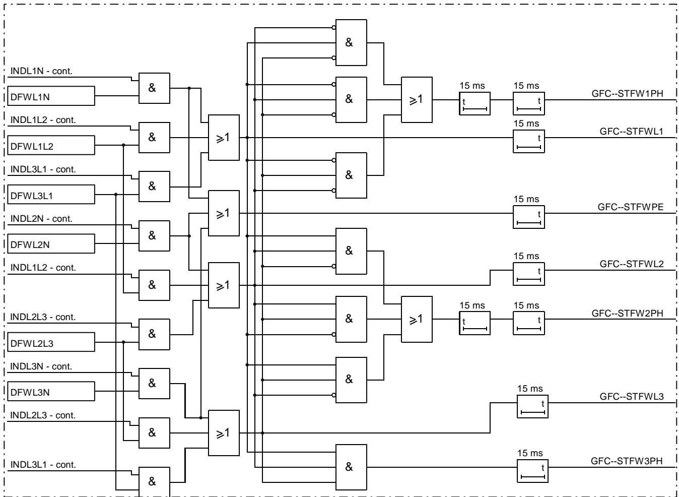
Figure 53: Composition of forward directed GFC signals.
