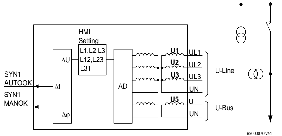
Figure 157: Connection of the synchrocheck function for one bay.
