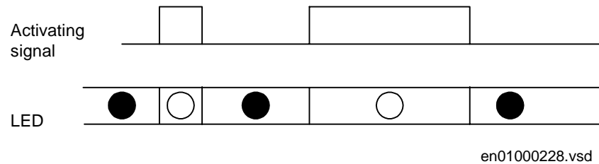
Figure 198: Operating sequence 1 (Follow-S)
