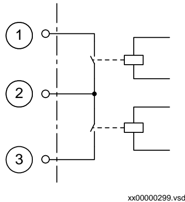
Figure 262: One of twelve binary output groups
