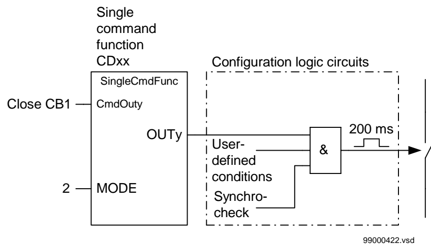
Figure 184: Application example showing a logic diagram for control of a circuit breaker via configuration logic circuits
