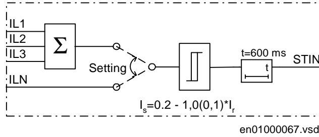
Figure 79: Residual current measurement
