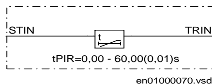
Figure 82: Function for residual current detection
