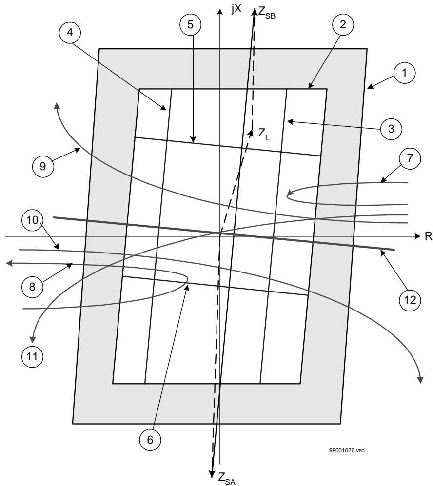
Figure 64: Impedance trajectories during oscillations in power system and basic operating characteristics of the pole slip protection.
