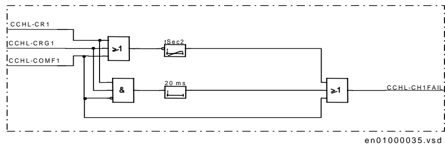
Figure 193: communication channel fail logic.
