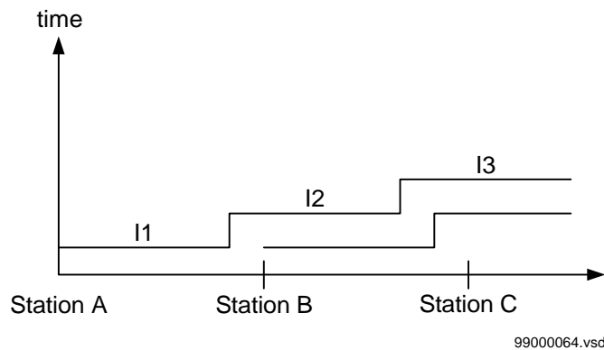
Figure 118: Example of selectivity plan for the directional current steps.
