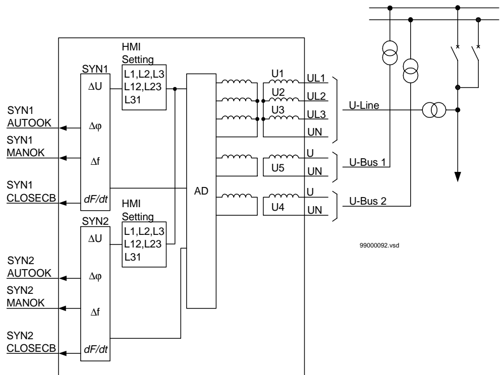
Figure 167: Connection of the phasing and synchrocheck function for one bay.
