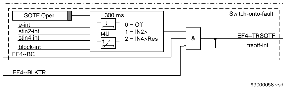
Figure 108: Simlified logic diagram of internal function Switch-onto-fault.
