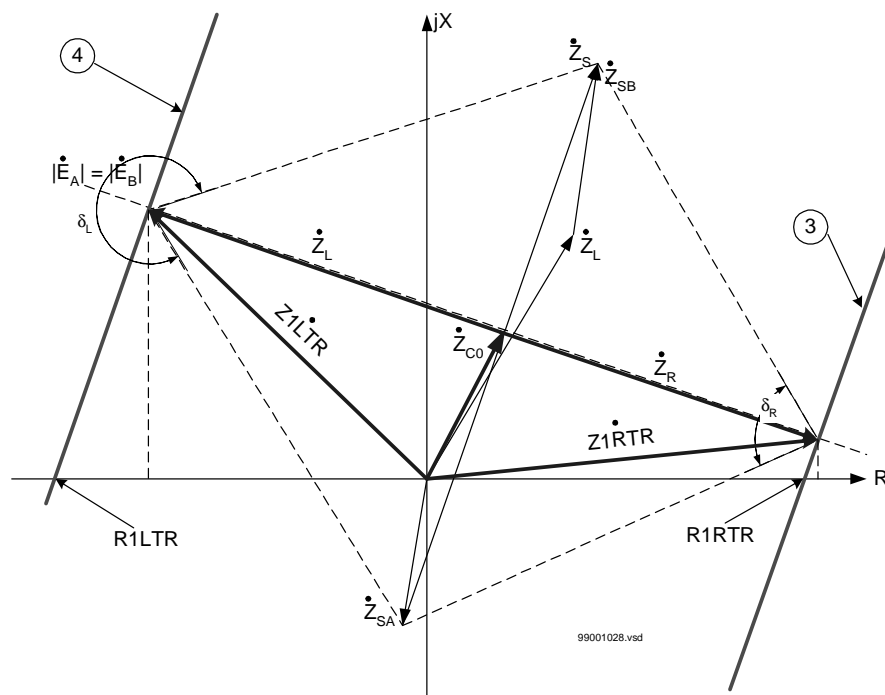
Figure 66: Left (4) and right (3) tripping characteristics and setting of their resistive reach R1LTR and L1RTR respectively.
