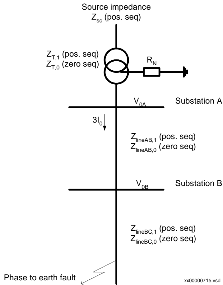
Figure 123: Equivalent of power system for calculation of setting
