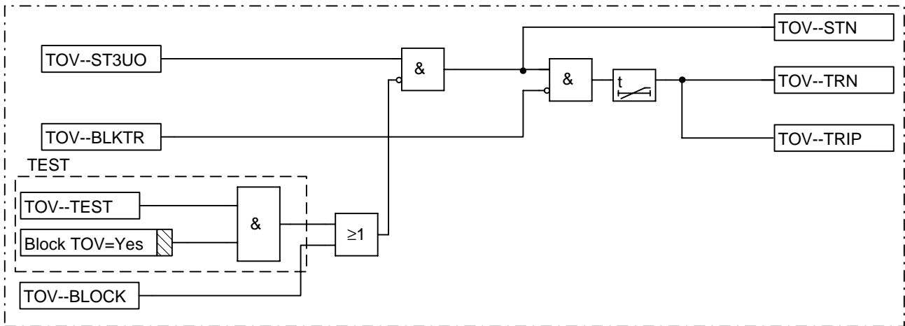
Figure 142: Logic diagram, time delayed overvoltage protection, residual
