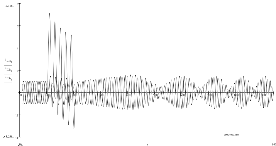
Figure 61: Phase currents in relay point during the pole slip conditions caused by a L1-N fault.
