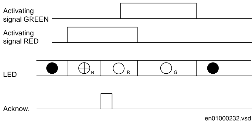
Figure 201: Operating sequence 3, two colors involved
