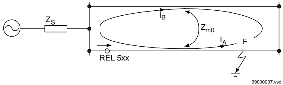
Figure 41: Double-circuit parallel operating line
