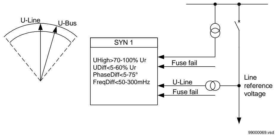
Figure 156: Synchrocheck.
