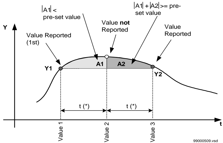
Figure 229: Periodic reporting with amplitude dead-band supervision in series
