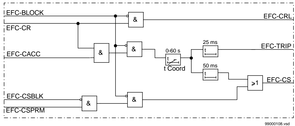
Figure 125: Simplified logic diagram, Scheme type = permissive
