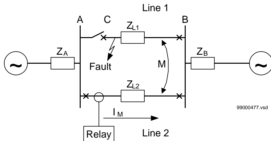
Figure 114: Two parallel lines. Influence from parallel line to the through fault current: I_M
