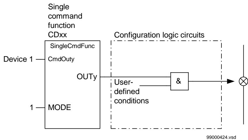
Figure 186: Application example showing a logic diagram for control of external equipment via configuration logic circuits
