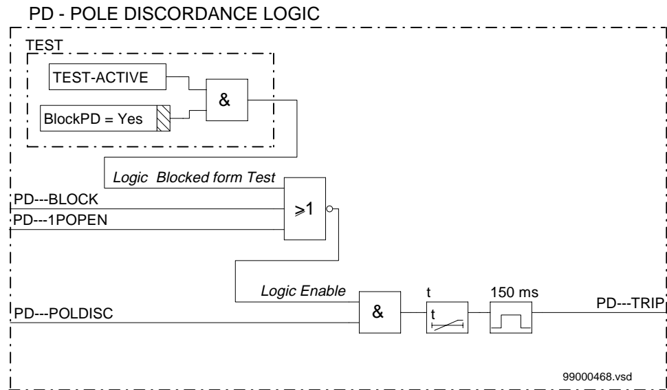
Figure 188: Simplified logic diagram of pole discordance logic - contact based
