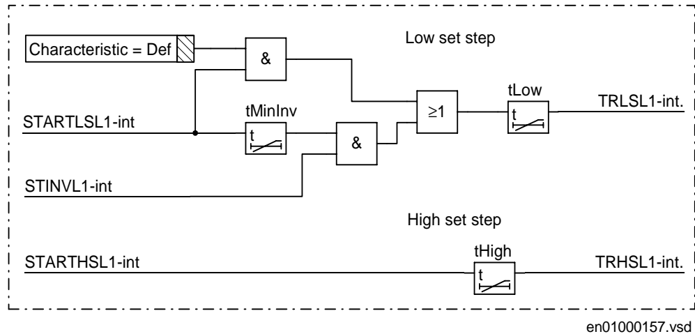
Figure 101: Delayed time operation for low set step and general time delay
