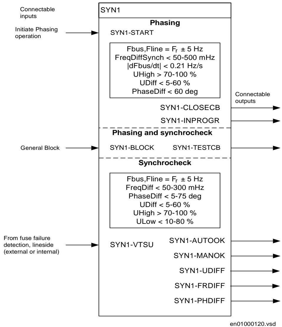
Figure 174: Input and output signals.
