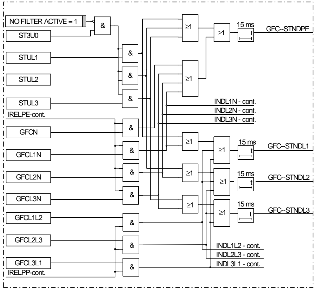
Figure 52: Composition of non-directional GFC signals
