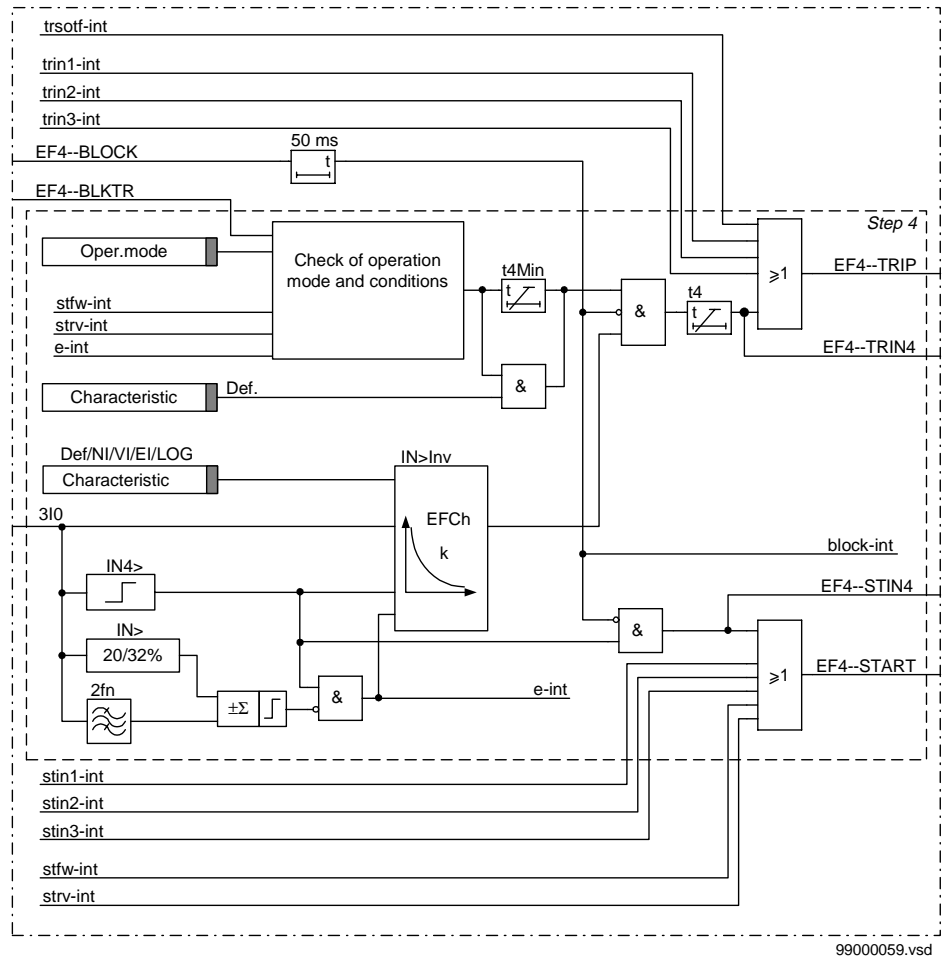
Figure 109: Simplified logic diagram of internal function step 4.
