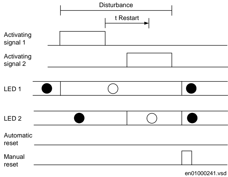
Figure 210: Operating sequence 6 (LatchedReset-S), two indications within same disturbance but with reset of activating signal between
