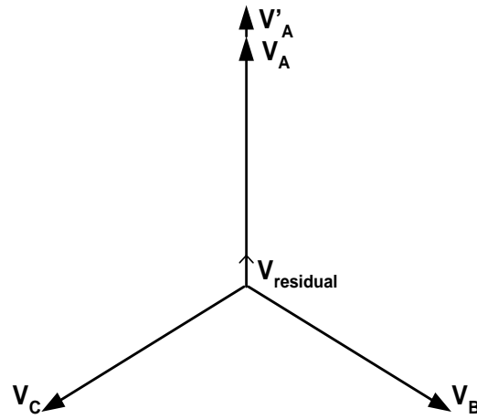
Figure 155: The residual voltage will be equal to the voltage increase in the phase with the broken capacitor element.
