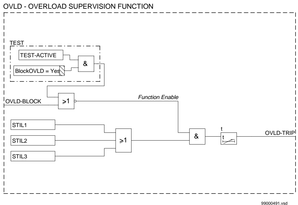
Figure 145: Simplified logic diagram of overload supervision function
