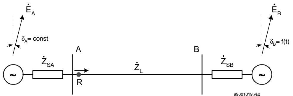
Figure 76: Power system reduced to a two machine system.
