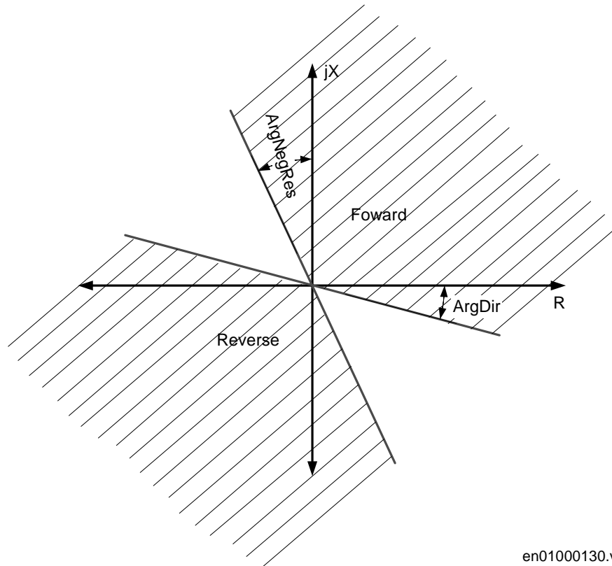
Figure 45: Directional lines define the forward and reverse operating area for each distance protection zone
