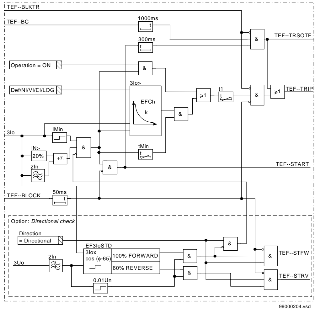
Figure 104: Simplified logic diagram for the residual overcurrent protection
