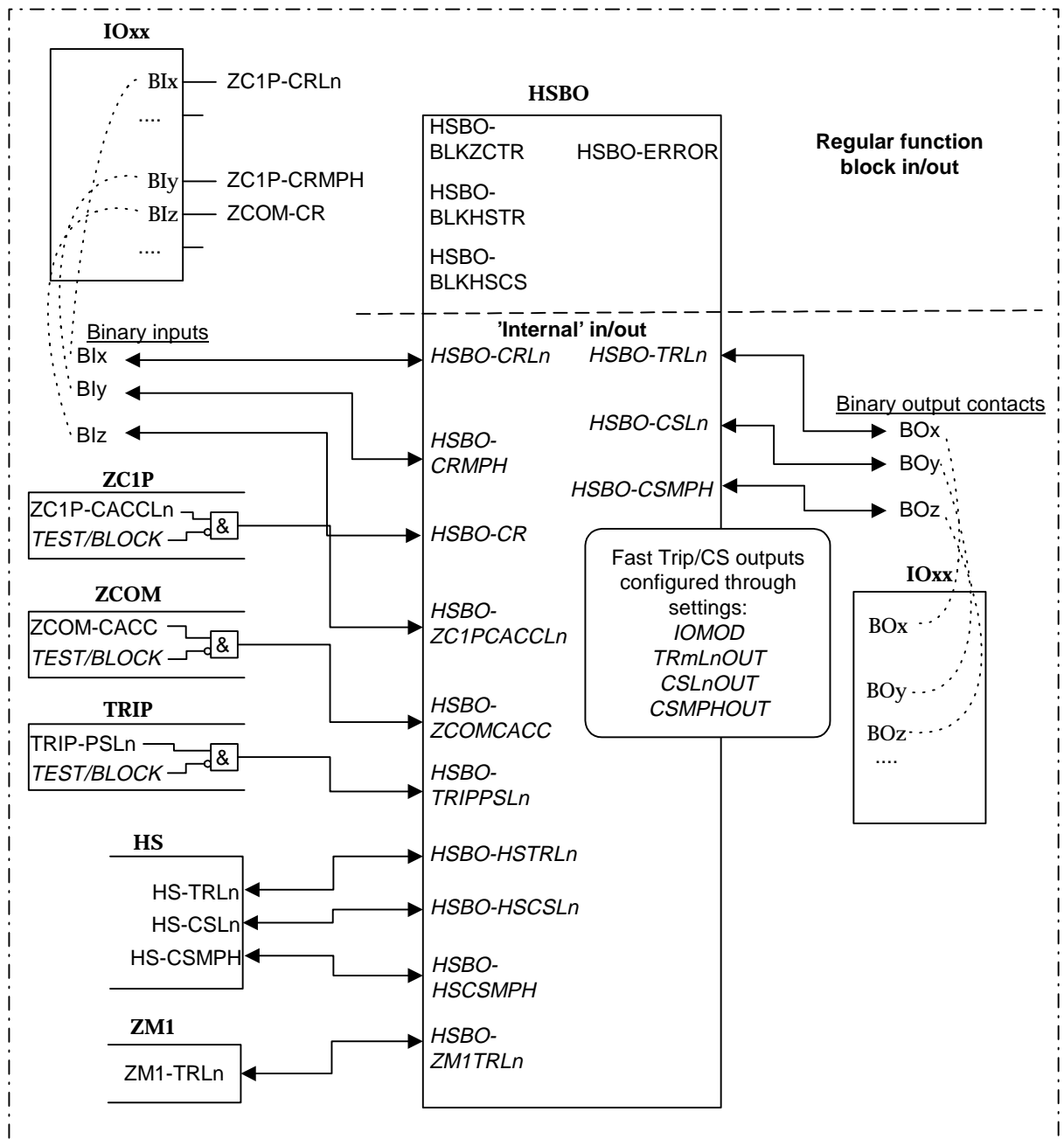
Figure 189: Simplified diagram of the high-speed binary out logic function together with depending functions
