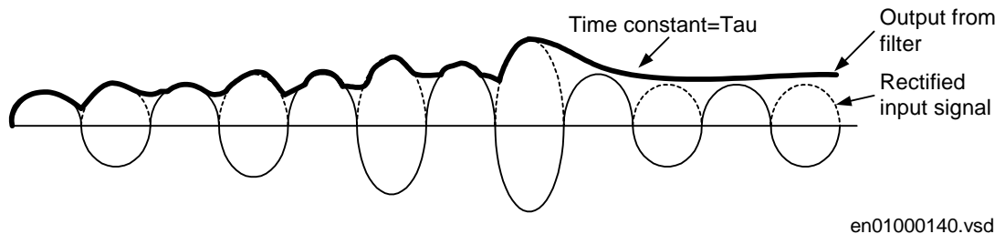
Figure 78: Filtering function
