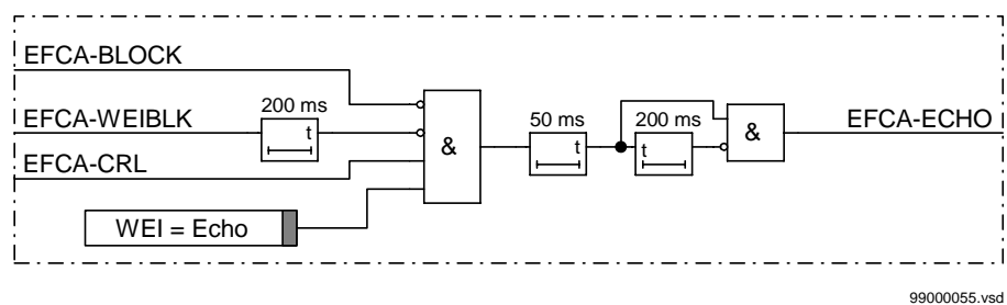
Figure 130: Simplified logic diagram, weak end infeed - echo.
