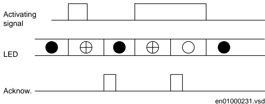
Figure 200: Operating sequence 3 (LatchedAck-F-S)
