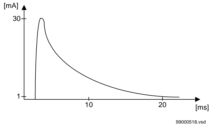
Figure 259: Current through the relay contact
