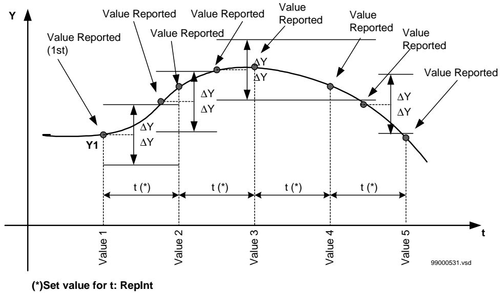
Figure 220: Periodic reporting with amplitude dead-band supervision in parallel.
