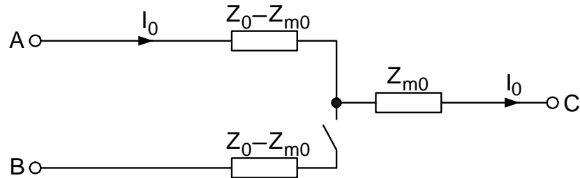
Figure 44: Equivalent zero-sequence impedance circuit for a double-circuit line with one circuit disconnected and not earthed
