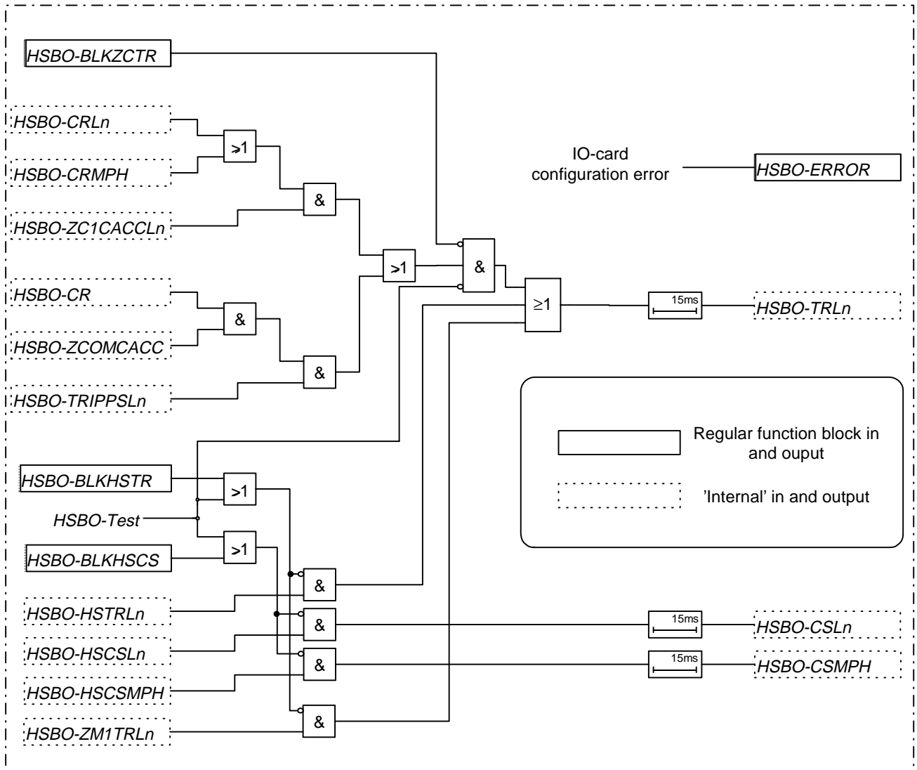
Figure 190: Simplified logic diagram of the function block
