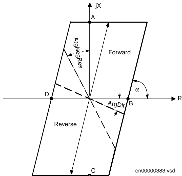
Figure 33: General operating characteristic of impedance measuring elements
