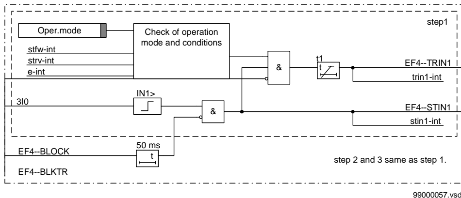
Figure 107: Simplified logic diagram of internal function Step 1. Step 2 and step 3 are the same.
