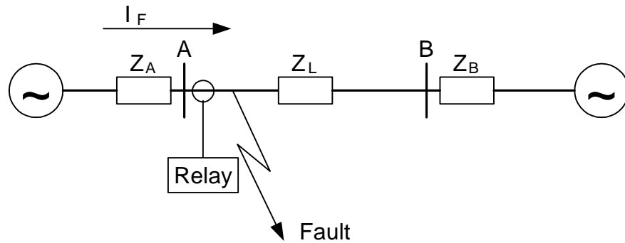
Figure 116: Fault current: I_F
