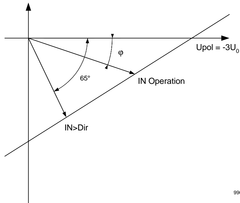
Figure 106: Measuring characteristic of the directional element
