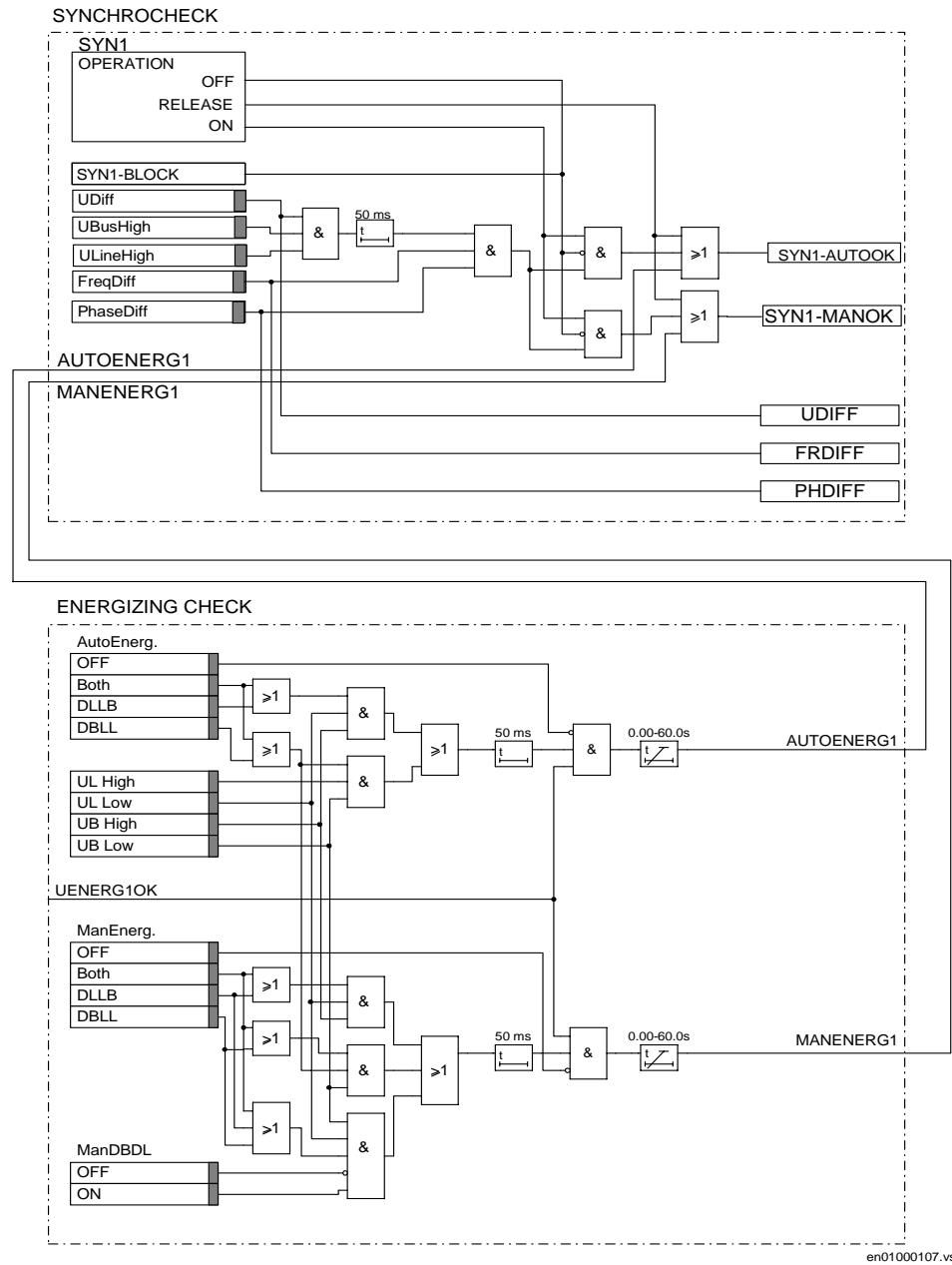
Figure 173: Simplified logic diagram - Synchrocheck and energizing check for one circuit breaker. The internal signal UENERG1OK derives from the external or internal fuse failure inputs SYN1-UB1OK/FF and SYN1-VTSU.
