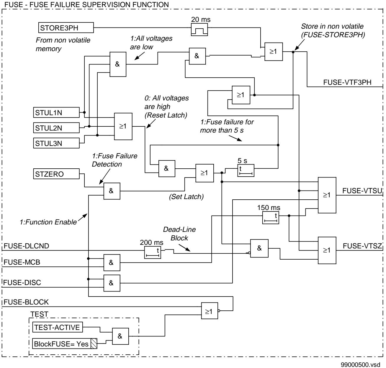
Figure 150: Simplified logic diagram for fuse failure supervisione function, zero se- quence based
