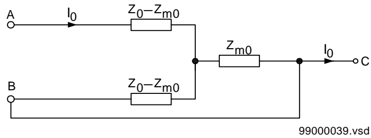
Figure 43: Equivalent zero-sequence impedance circuit for the double-circuit line that operates with one circuit disconnected and earthed at both ends
