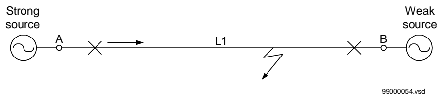
Figure 129: Initial condition
