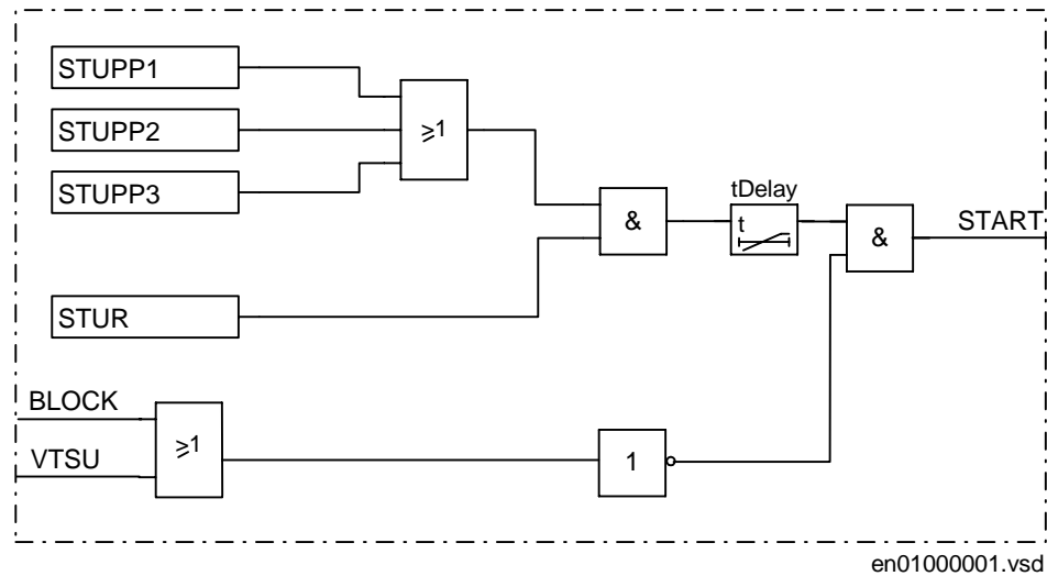
Figure 153: TCT logic
