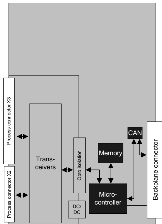
Figure 240: Block diagram for the galvanic communication module
