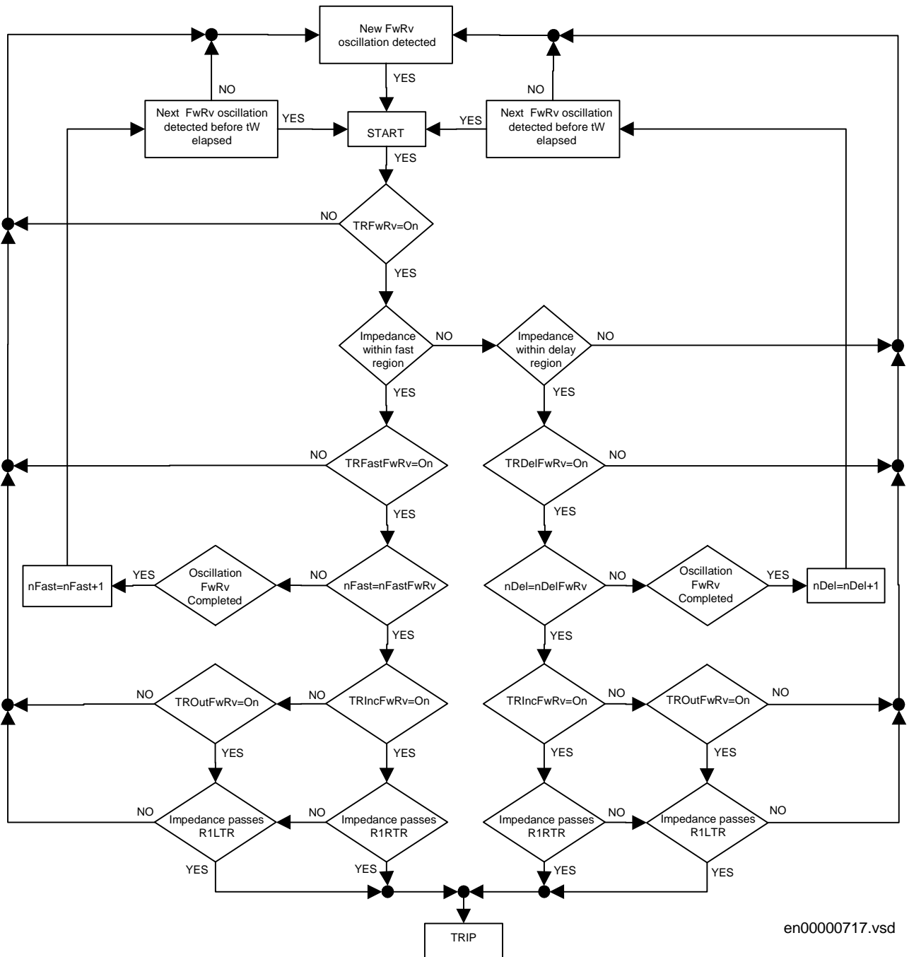
Figure 72: Flow-chart presenting the operation of the pole slip protection for the forward to reverse transition (FwRv) after the oscillation has been detected.
