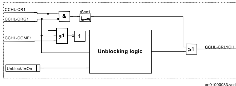
Figure 191: Communication channel logic 1
