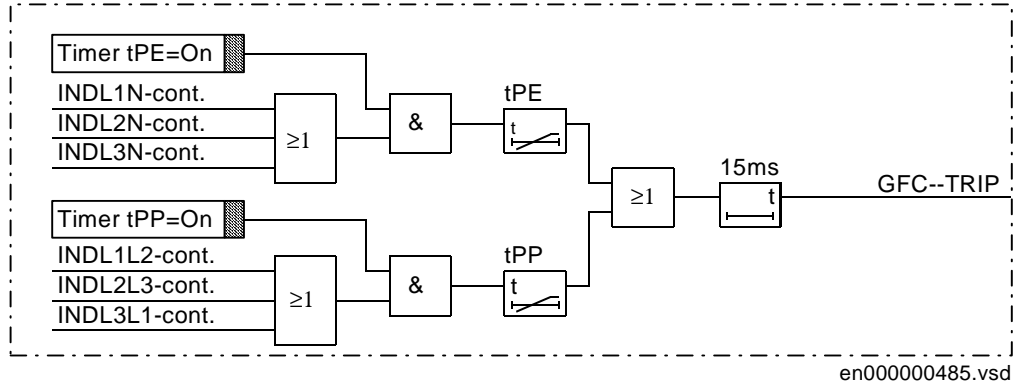
Figure 55: Composition of time-delayed tripping signal
