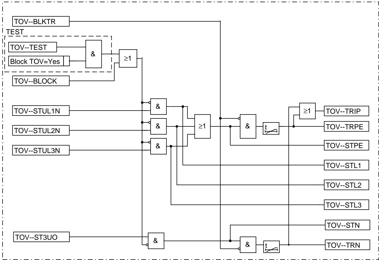
Figure 140: Time delayed overvoltage protection - simplified logic diagram
