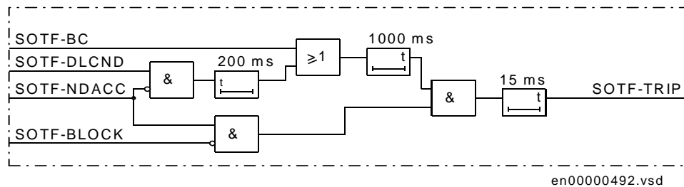
Figure 47: SOTF function - simplified logic diagram
