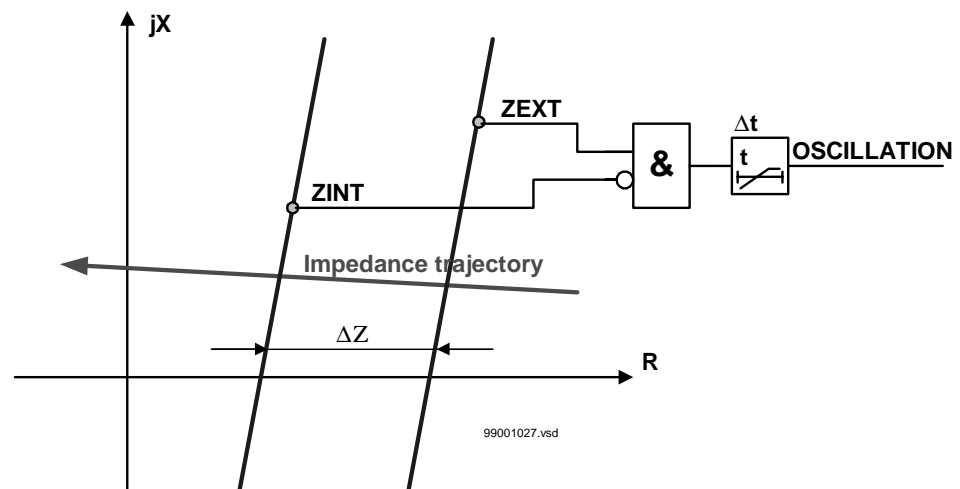
Figure 65: Detection of the oscillation by the (DZ)/(Dt) method.
