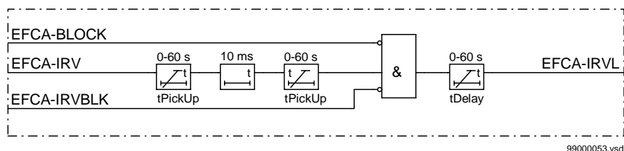
Figure 128: Simplified logic diagram, current reversal
