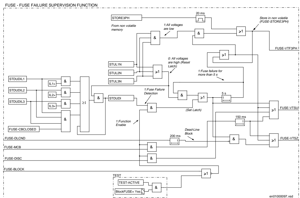
Figure 151: Simplified logic diagram for fuse failure supervision function, du/dt based.
