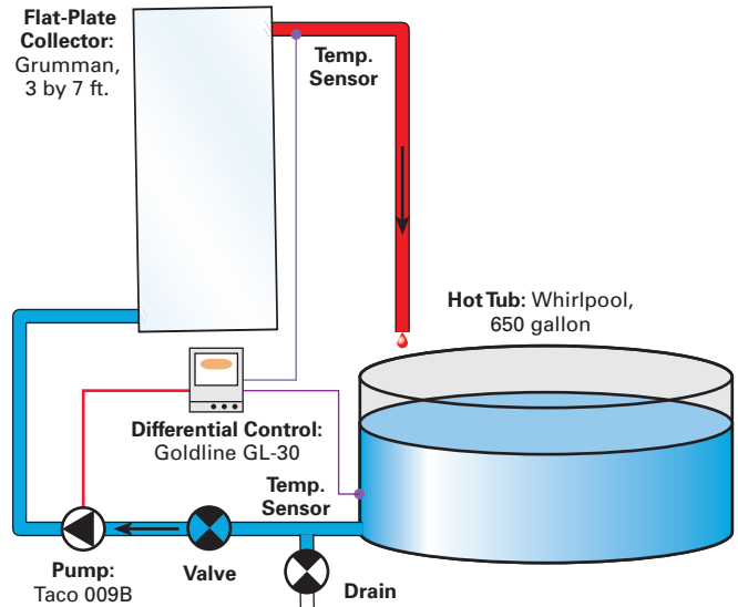
Collectors and pipes should be slightly slanted to allow the water to drain from the collectors.
