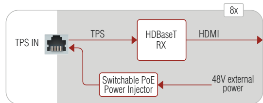
MX-TPS2-IB-P
