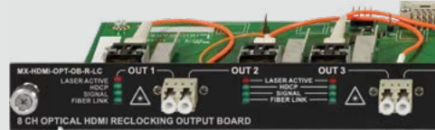
MX-HDMI-OPT-OB-R-LC
