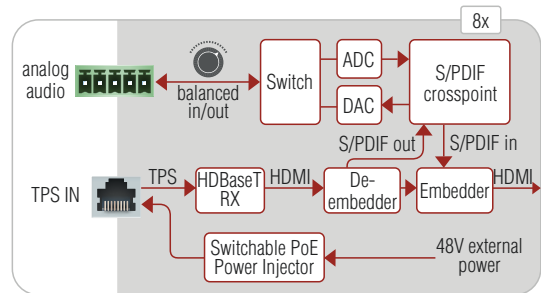
MX-TPS2-IB-AP
