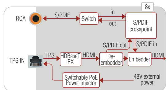
MX-TPS2-IB-SP
