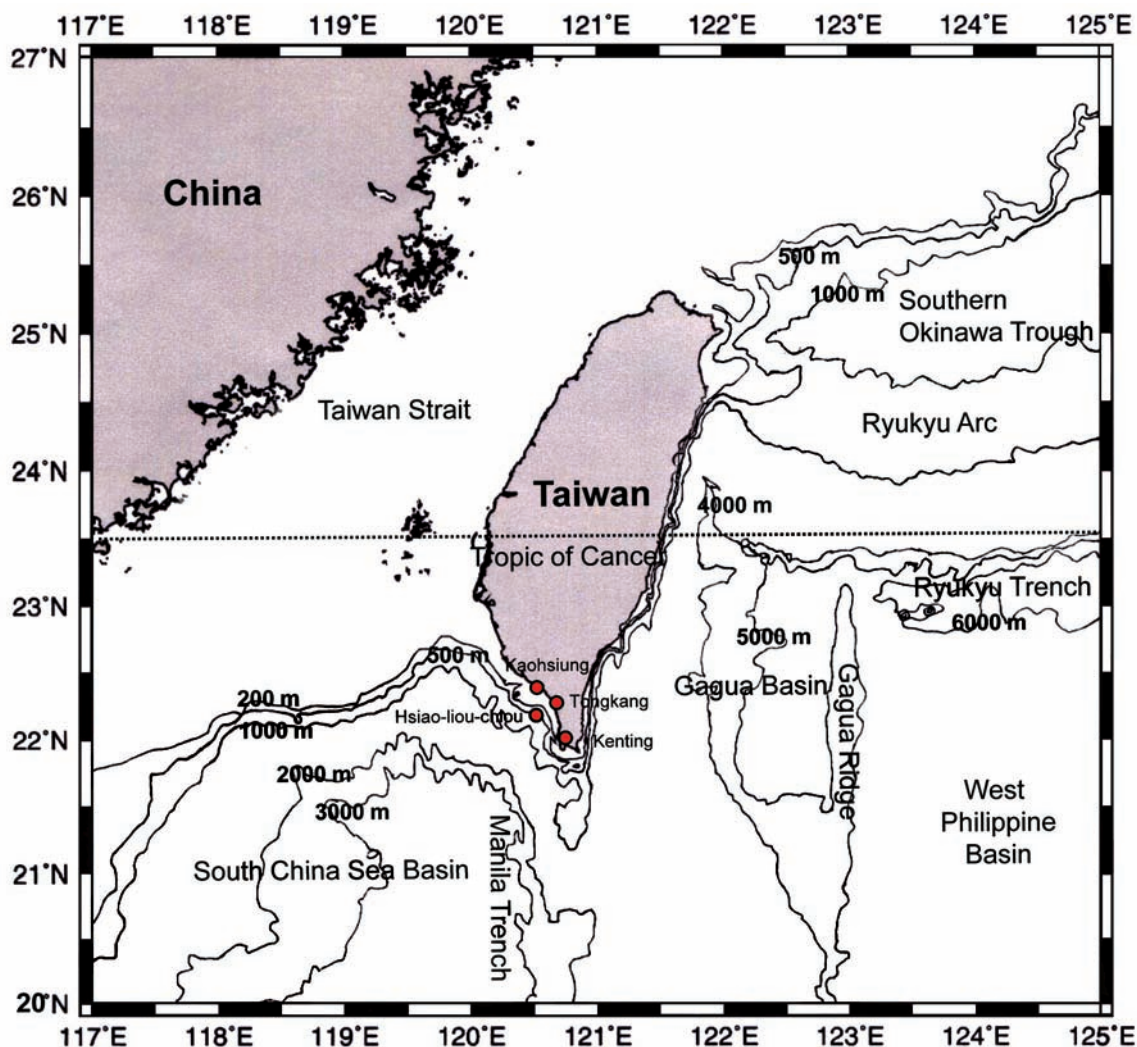
Fig. 1. Map of Taiwan and isobathic lines in adjacent waters showing fishery harbors or locality names using in this paper. The location of Pratas and Spratly Islands in central and southern SCS are beyond the range of this map. Please refer to Randall & Lim (2000: 51).
