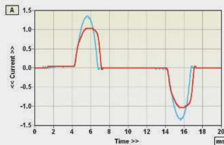
ABOVE: Distorted mains (charging) current waveform (red) versus significantly more linear waveform delivered by the PS Audio P3 Power Plant (blue)
