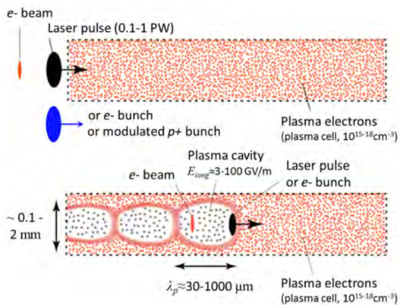
FIG. 37. Concept of the plasma wakefield acceleration driven either by a short laser pulse (LWFA), or by a short electron bunch or by long(er) modulated proton bunch (PWFA, adapted from [518]).
