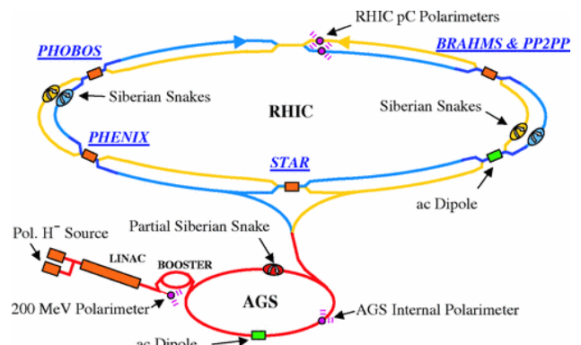
FIG. 13. Layout of the RHIC collider with its injector complex [335]. The two RHIC rings cross in six points. The two principal experiments still running are PHENIX and STAR. The smaller experiments PHOBOS, BRAHMS and PP2PP have been completed. The LINAC is the injector for polarized protons into the Booster/AGS/RHIC chain. A jet target used for precision beam polarization measurements. A tandem injector for ions has been replaced by an Electron Beam Ion Source (EBIS) starting with the 2012 run.
