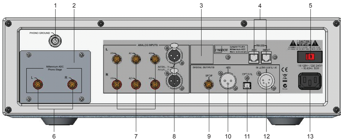
Figure 2: Millennium ADC rear panel.
