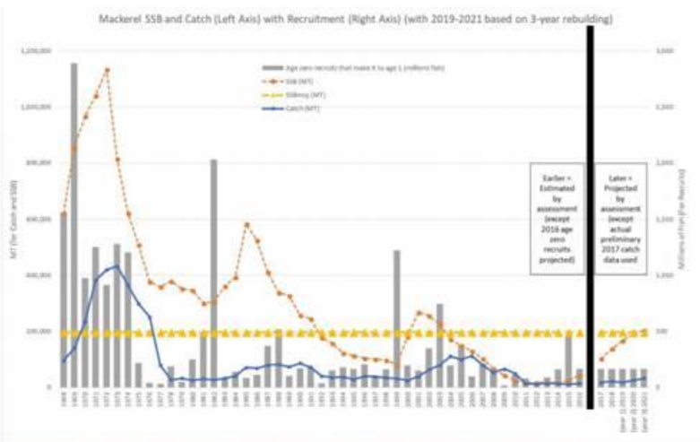
Figure 10. Mackerel SSB and catch including 2019-2021 projections under 1b (3-year rebuilding)
