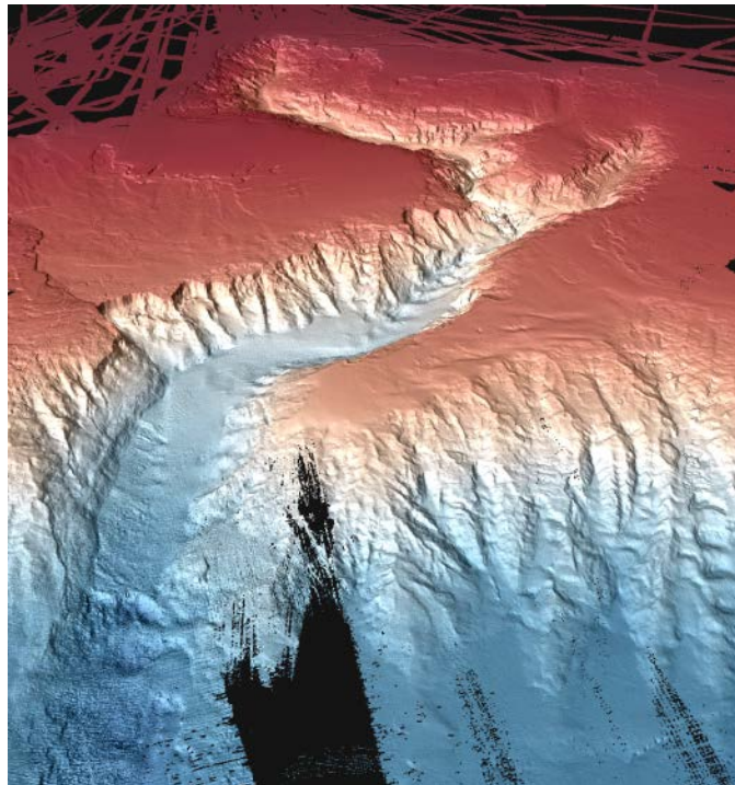
Cover image: 3D view of Perth Canyon looking east
