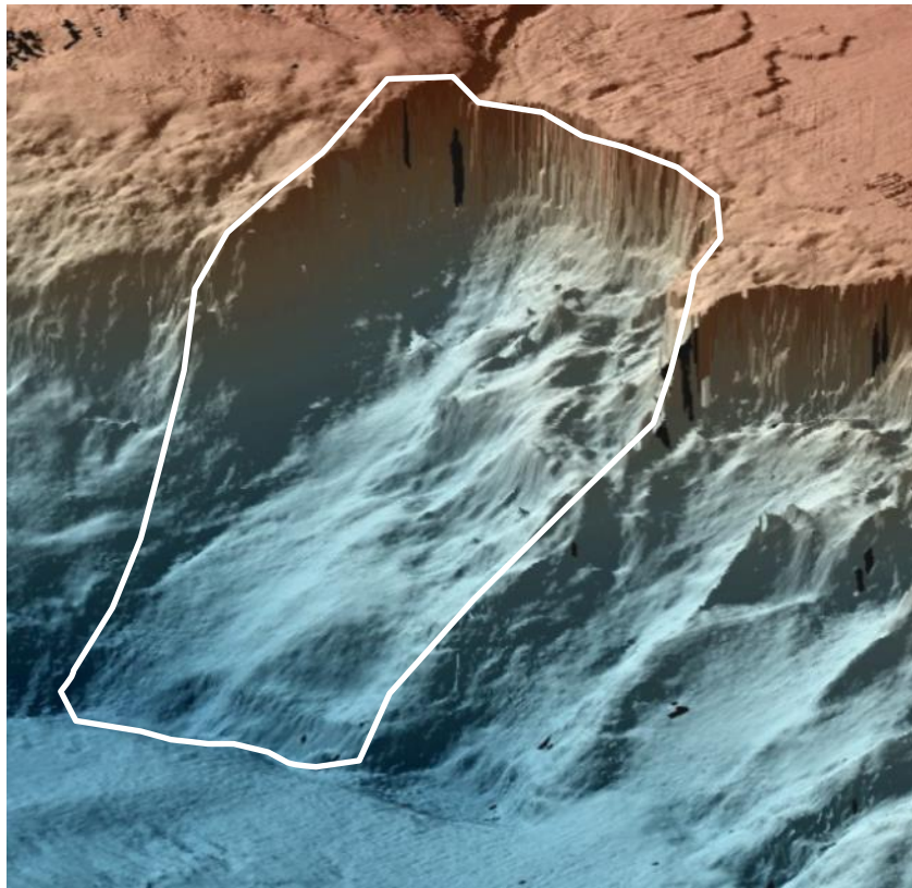
Figure 5: Mass movement feature on the northern wall of Perth Canyon (refer Fig.1 for location). The canyon wall is 1800 m high at this point.
