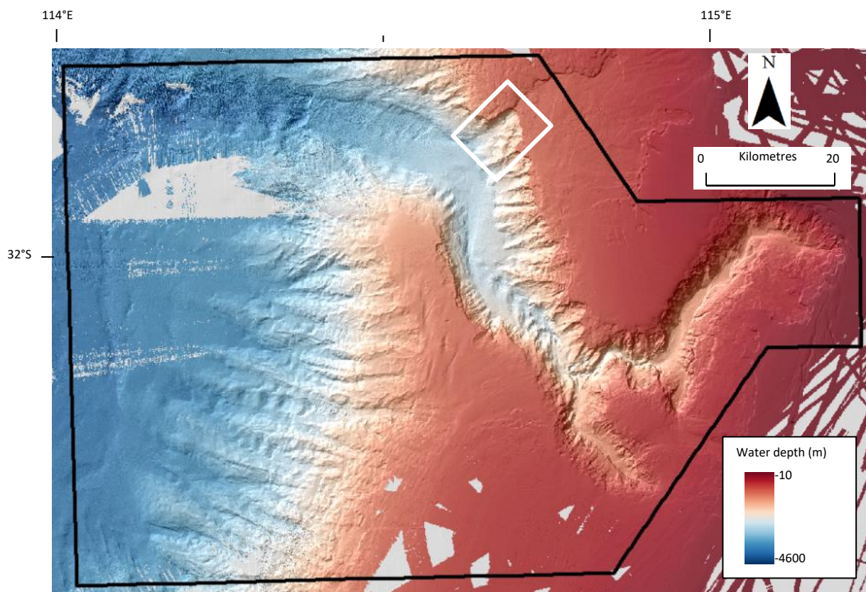
Figure 1: Seabed within Perth Canyon Marine Park, showing hill-shaded high-resolution (40 m) multibeam bathymetry data, which covers 97% of the marine park area. The black outline indicates the Perth Canyon Marine Park boundary, and the white inset box indicates the location of Fig. 5. Grey areas indicate areas with no data in the 40m grid.
