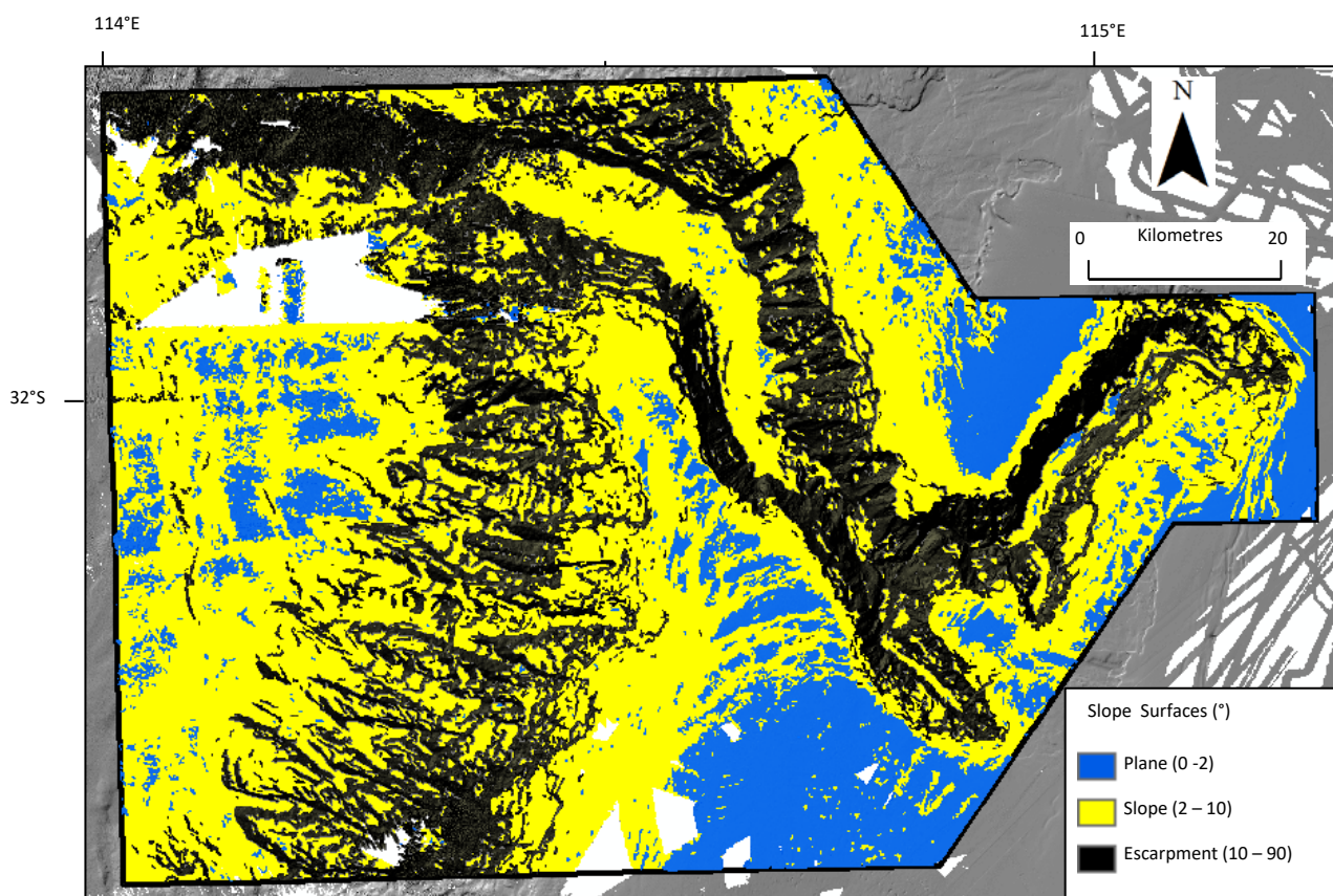
Figure 4: Seafloor Surfaces within Perth Canyon Marine Park mapped from a 40 m bathymetry grid (Fig. 1), using a 40m hillshade grid as the background.
