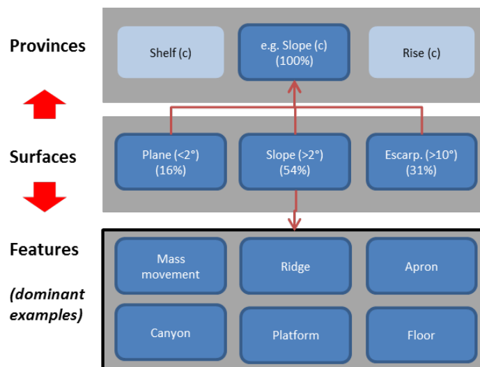
Figure A.1 Surfaces are the building blocks of higher level Provinces and are divided to define Features . Of the 34 Feature types we have described in our glossary, six dominate the Perth Canyon Marine Park survey and their proportions of the survey area are illustrated in this schematic.
