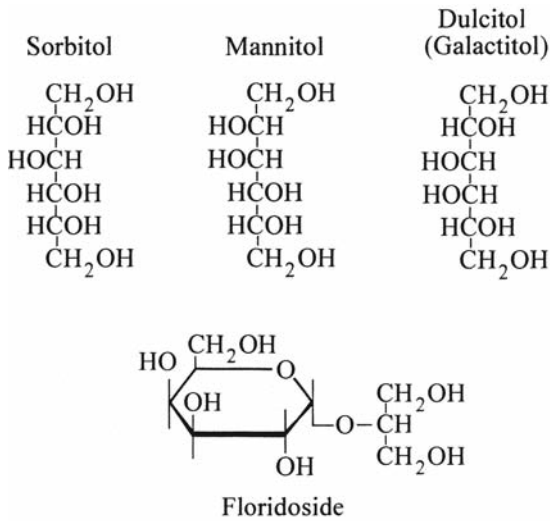
Fig. 4.4 Chemical structure of low molecular polysaccharides that occur in the red algae.
