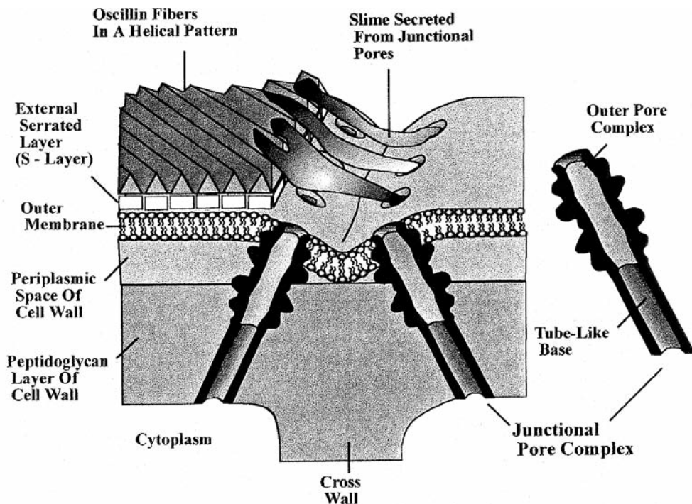
Fig. 2.4 A model of the junctional pore complex of a cyanobacterium. Extrusion of slime through the circumferentially arranged junctional pores on one side of the cross wall results in forward movement of the filament in contact with the substrate. The arrangement of the oscillin fibers in the outer layer of the cell wall determines whether the filament rotates as it glides over the surface. In the drawing, the oscillin fibers are spiraled so the filament rotates as it glides. (Modified from Hoiczky and Baumeister, 1998.)
