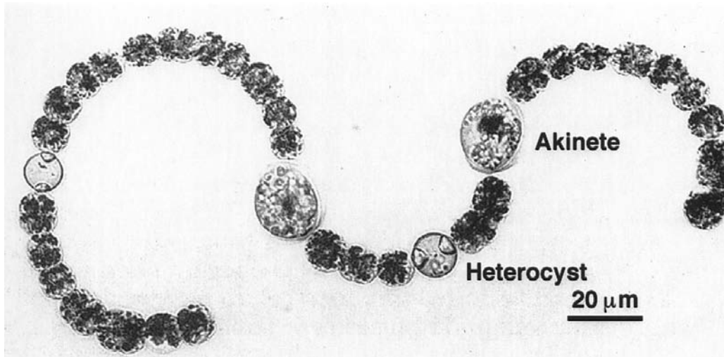
Fig. 2.16 Light micrograph of Anabaena crassa showing vegetative cells, akinetes, and heterocysts. (From Li et al., 1997.)
