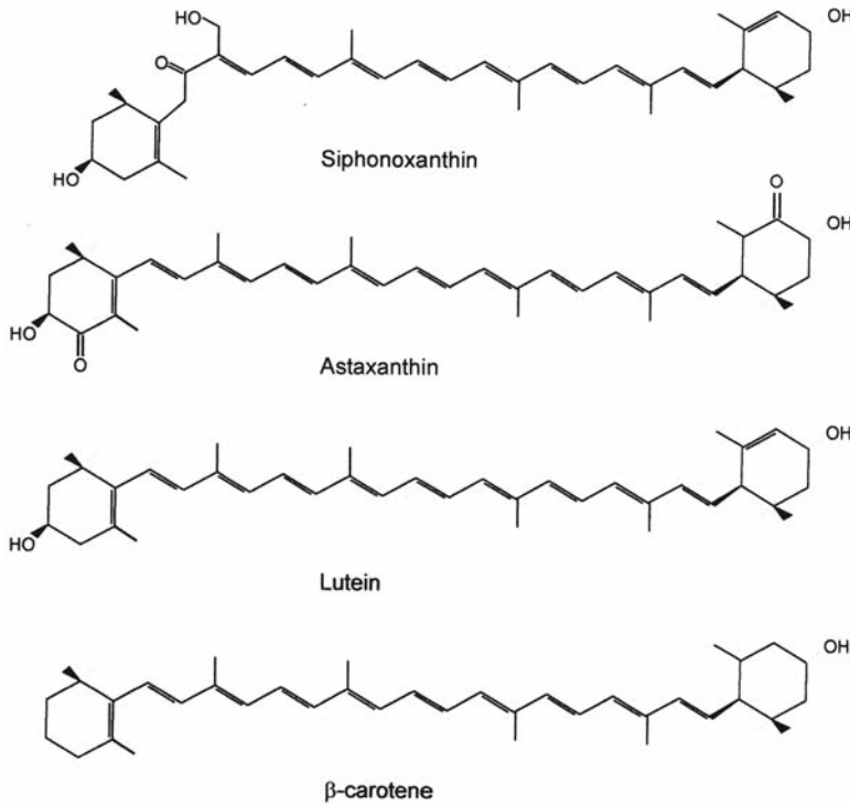
Fig. 5.1 The chemical structures of carotenoids of the Chlorophyta.
