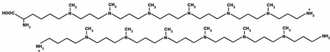
Silaffin
