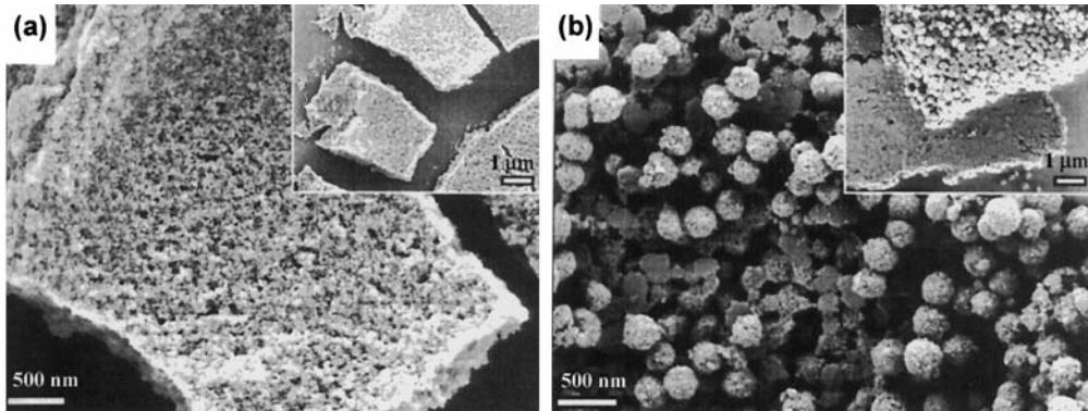
Fig. 17.14 Scanning electron micrographs of silica spheres precipitated out of solution using two different silaffins and polyamines. The silica spheres in (a) are much smaller than the silica spheres in (b). The size of the silica spheres is controlled by the type of silaffin and/or polyamine in the silica deposition vesicle of the diatom. (From Kroger et al., 2000.)
