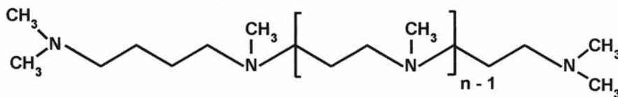
Polyamine
