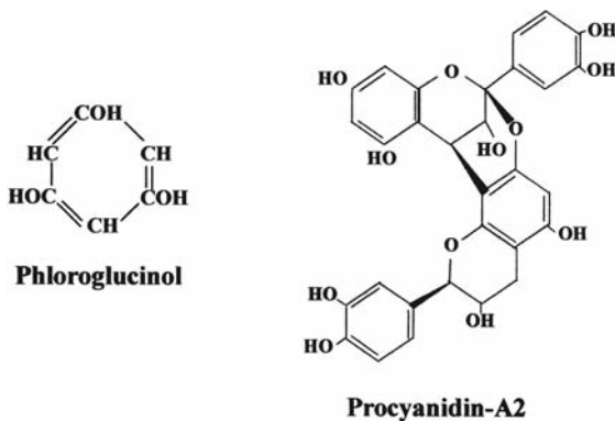
Fig. 21.6 Chemical structure of phloroglucinol, the basic building block of polyphenols and the chemical structure of the polyphenol procyanidin.
