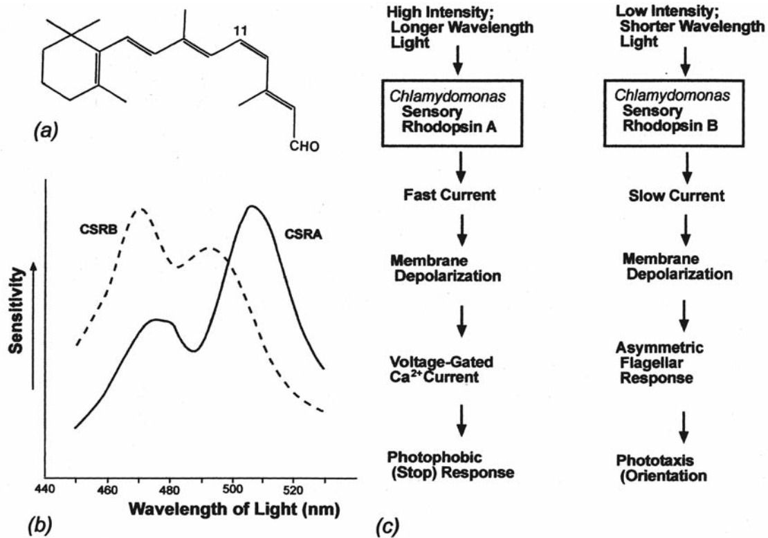
Fig. 5.3 (a) The structure of 11- cis -retinal, part of the photoreceptor molecule in Chlamydomonas . (b) Action spectra showing the sensitivity of the photoreceptors Chlamydomonas sensory rhodopsin A (CSRA) and Chlamydomonas sensory rhodopsin B (CSRB) to different wavelengths of light. (c) Scheme of light signal transduction initiated by the two sensory rhodopsin pigments in Chlamydomonas . ((b),(c) adapted from Sineshchekov et al., 2002.)
