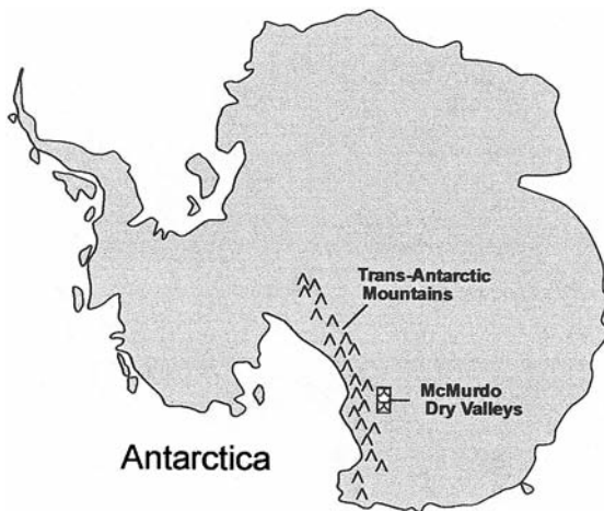
Fig. 9.6 The location of the McMurdo Dry Valleys in Antarctica.
