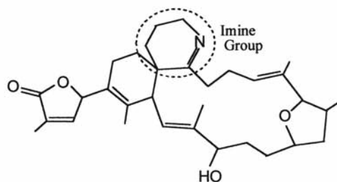
ii. Gymnodimine
