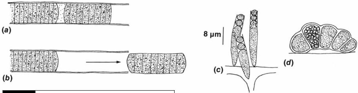
Fig. 2.34 (a),(b) Formation of a hormogonium in Oscillatoria . (c) Baeocyte formation in Chamaesiphon incrustans . (d) Baeocyte formation in Dermocarpa pacifica . (After Smith, 1950.)
