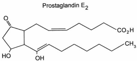
Fig. 4.43 The chemical structure of prostaglandin E 2 .
