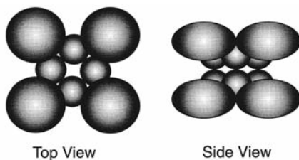
Fig. 1.13 The structure of Form I variation of Rubisco showing the eight large subunits and eight small subunits.
