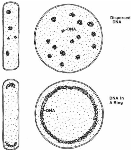
Fig. 1.17 Semidiagrammatic drawing of the two types of distribution of DNA in algal chloroplasts. Side and face views of the plastids are drawn. (Adapted from Coleman, 1985.)
