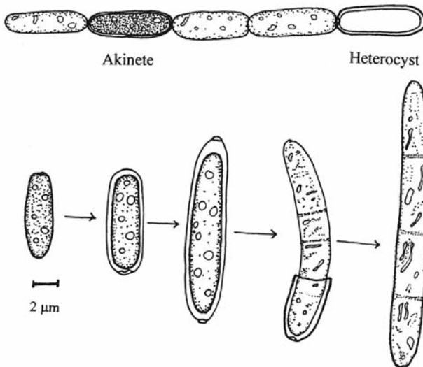
Cylandrospermopsis raciborskii
