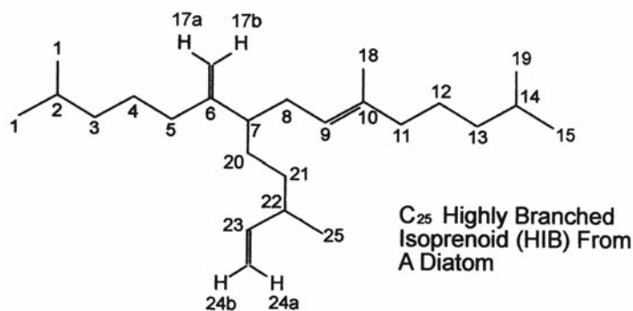
Fig. 17.37 Chemical structure of a highly branched alkene characteristic of diatoms.
