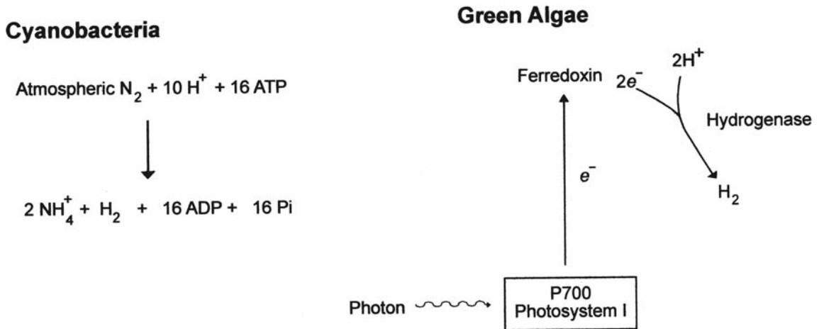
Fig. 23.10 The chemical reactions that result in the formation of hydrogen gas in the cyanobacteria and green algae.
