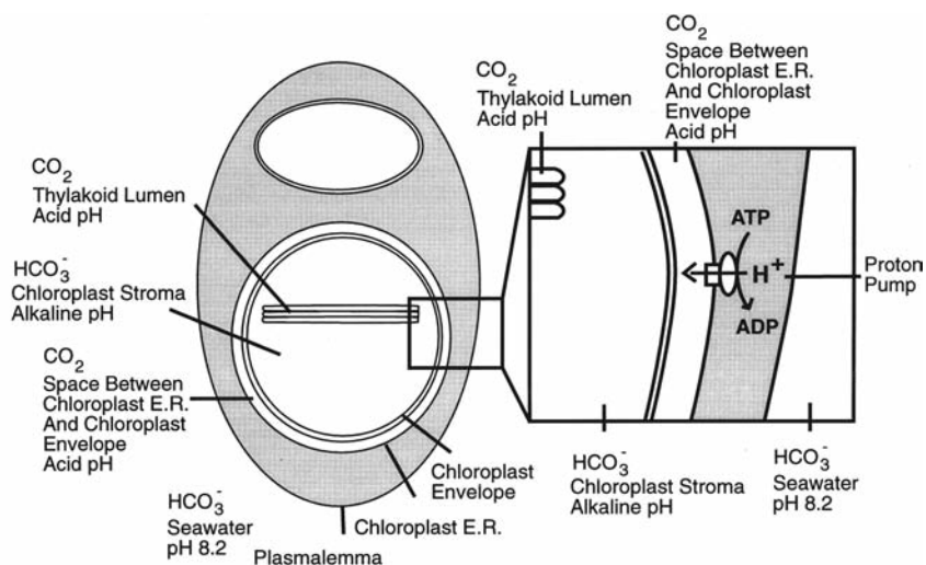
Fig. IV.2 Diagrammatic representation of the compartments present in an alga with one membrane of chloroplast endoplasmic reticulum. The pH and predominant form of dissolved inorganic carbon are indicated for each compartment.
