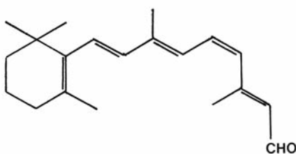
Fig. 1.15 The structure of chlamyrodopsin, the photoreceptor in Chlamydomonas .
