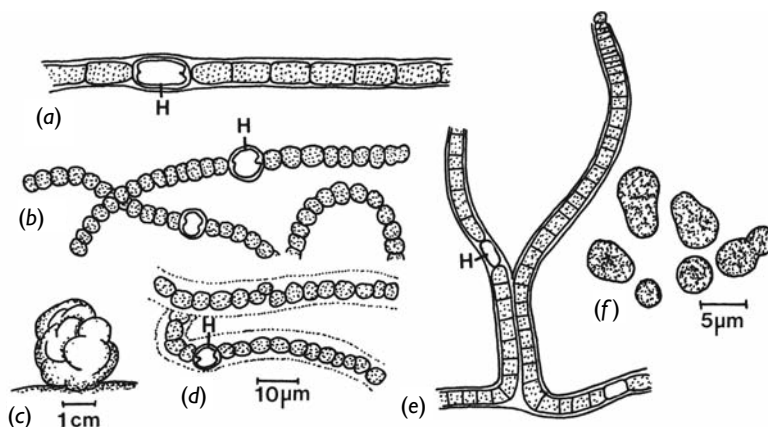
Fig. 2.46 (a) Aulosira fertilissima . (H) Heterocyst. (b) Nostoc commune . (c,d) N. verrucosum . (e) Scytonema hofmanni . (f) Chamaesiphon sp., showing formation of exospores. ((a), (e) after Desikachary, 1959; (b) after Prescott, 1962; (f) after Waterbury and Stanier, 1977.)
