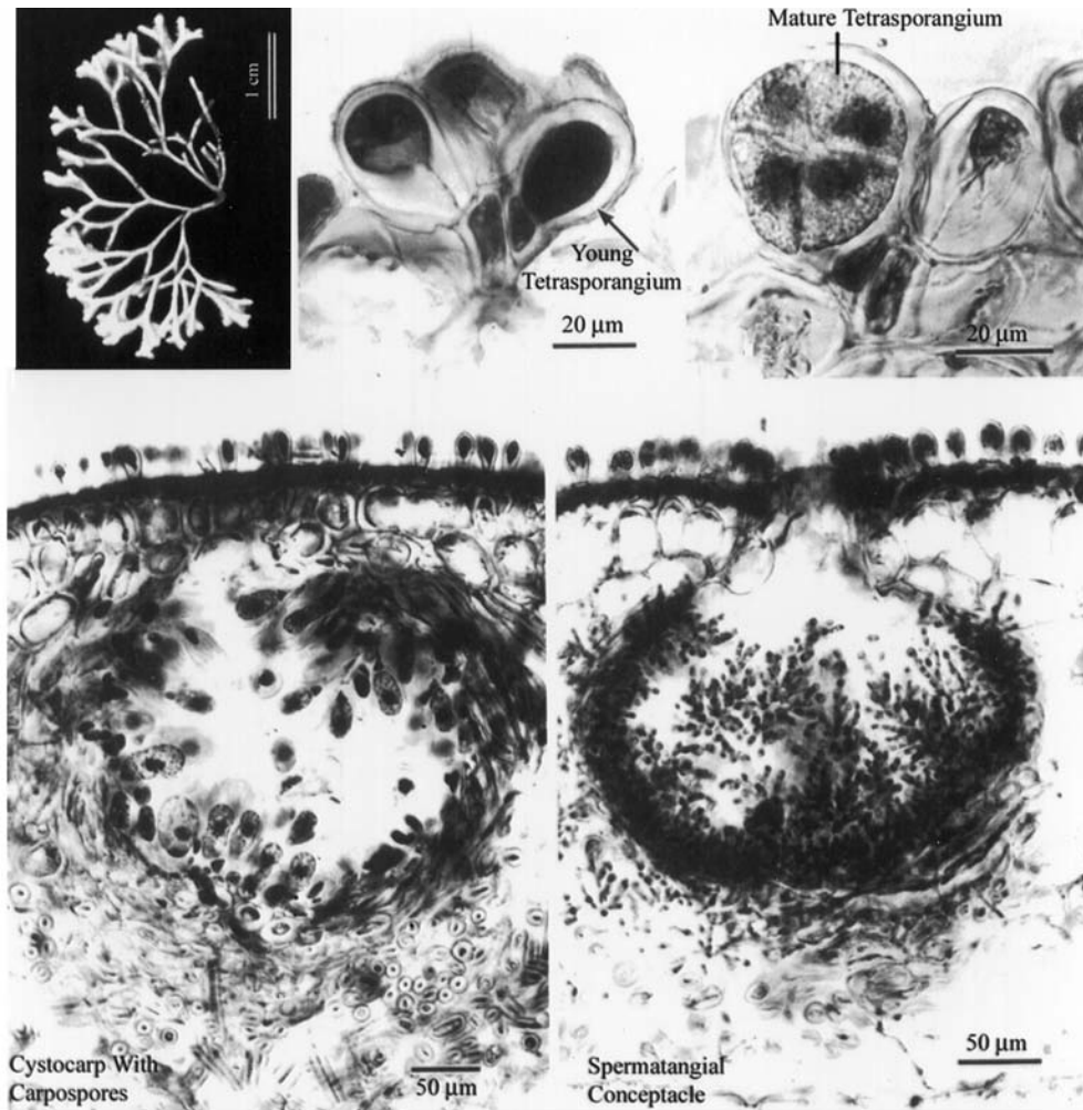
Fig. 4.34 Photographs of vegetative and reproductive structures of Galaxaura apiculata . (From Kurihara et al., 2005.)
