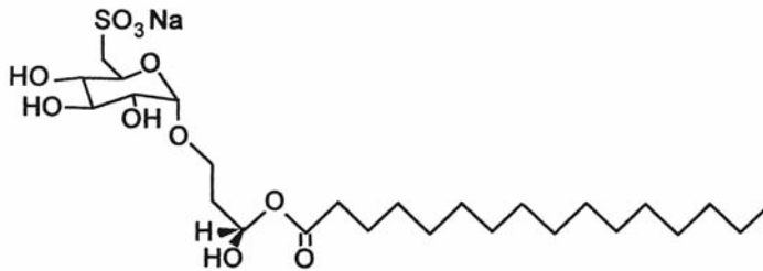
1-O-palmitoyl-3-O-(6'-sulfo-a-D-quinovopyranosyl)-sn-glycerol (PSQG)
