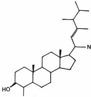
Fig. 7.37 The structure of dinosterol, the major sterol in dinoflagellates.
