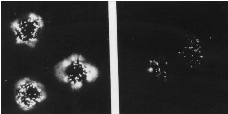
Fig. 7.39 The white spots in these photographs of Lingulodinium cells indicate fluorescence and thus localization of luciferin, the substrate that reacts with the enzyme luciferase and oxygen to produce light. The intensity of the luciferin fluorescence is greater in the night phase (left) of the circadian cycle of bioluminescence than in the day phase (right). The amount of luciferase shows a similar oscillation during the daily cycle. (From Johnson et al., 1985.)
