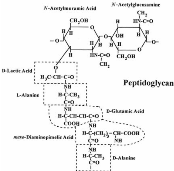
Fig. 2.2 The structure of a peptidoglycan molecule in the cell wall of cyanobacteria.
