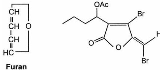
Fig. 4.14 Left: The chemical structure of furan, the basic building block of the furanones. Right: One of the halogenated furanones released by the red alga Delisea pulchra . Halogenated furanones inhibit the growth of epiphytes on this red alga.
