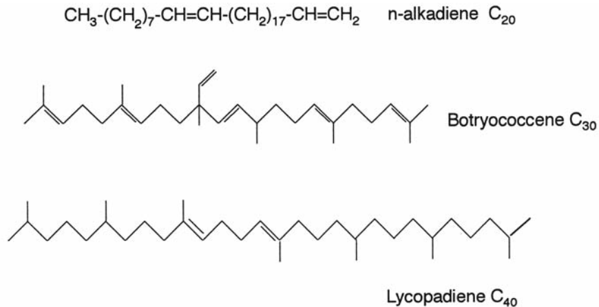
Fig. 5.78 The structure of hydrocarbons isolated from Botryococcus braunii . (Modified from Metzger et al., 1990.)
