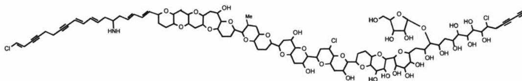
Fig. 23.3 Chemical structure of phycotoxins composed of cyclic imines and non-nitrogen compounds containing linear and macrocyclic polyethers.
