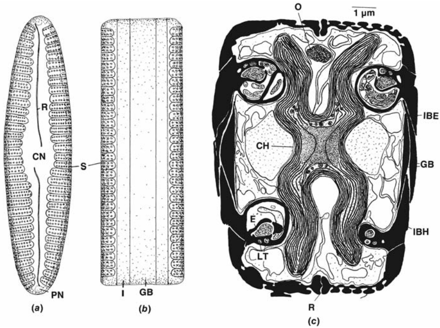
Fig. 17.1 Light microscopical drawing of valve (a) and girdle (b) views of the diatom Mastogloia . (c) Drawing of a transverse section of M. grevillei in the transmission electron microscope. (Ch) Chloroplast; (CN) central nodule; (E) elongate chamber of a septum; (GB) girdle band; (I) intercalary band; (IBE) intercalary band of the epitheca; (IBH) intercalary band of the hypotheca; (LT) locule tubule; (O) oil; (R) raphe; (S) stria. ((c) adapted from Stoermer et al., 1965.)
