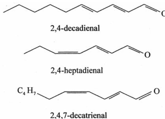
Fig. 10.9 Three unsaturated fatty-acid derivatives produced by chrysophytes that result in rancid or fishy odors.
