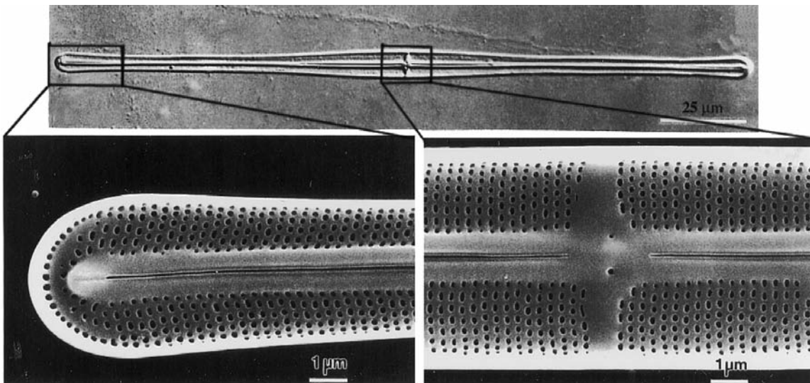
Fig. 17.4 Climaconeis colemaniae . Light and scanning electron micrographs of the frustule. The valve contains linear striae, each with 6–8 poroid areolae. The valve contains a raphe opening. Two pores occur in the area of the central nodule. (From Prasad et al., 2000.)
