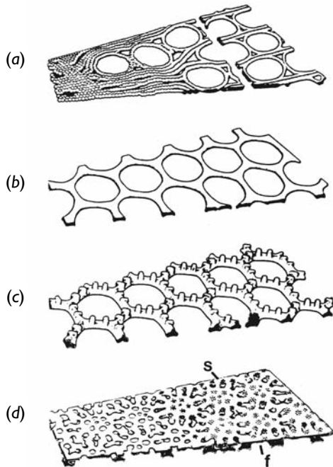
Fig. 17.15 Drawings of the formation of the frustule of the centric diatom Coscinodiscus wailesii . Initially silica is deposited in the part of the frustule that will be next to the plasma membrane in the mature frustule (a) and (b). Subsequently the exterior portion of the frustule is deposited in (c) and (d). The mature frustule has a sieve membrane (s) on the exterior and a foramen (f) on the interior of the loculus. (From Schmid and Volcani, 1983.)
