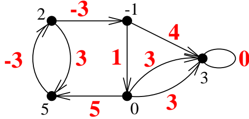
Figure 1: A function and its coboundary
