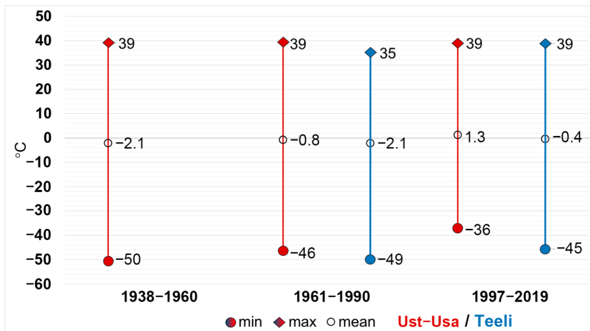
Figure 14. Air temperature values for different periods at two meteorological stations: Ust-Usa (in red) and Teeli (in blue).
