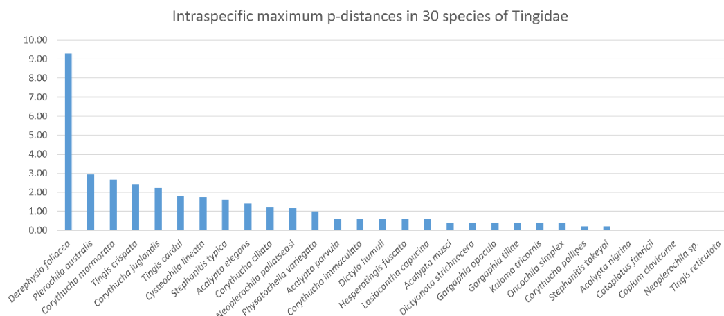
Figure 6. Intraspecific maximum p-distances (%) in 30 species of lace bugs (Hemiptera: Tingidae) based on a 501-bp alignment of the standard COI barcoding region ( n = 349 ).
