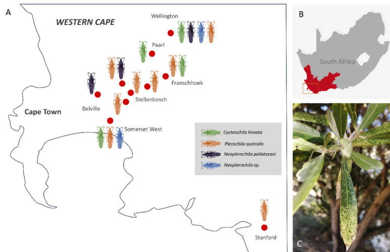
Figure 2. (A) Approximate geographic location of broad sampling areas (red dots) of olive lace bugs ( Cysteochila lineata , Neoplerochila paliatseasi , Neoplerochila sp. and Plerochila australis ) in the Western Cape province of South Africa. (B) Study area in the Western Cape. (C) Characteristic chlorotic spots on the leaves of a cultivated olive tree caused by feeding activity of olive lace bugs.
