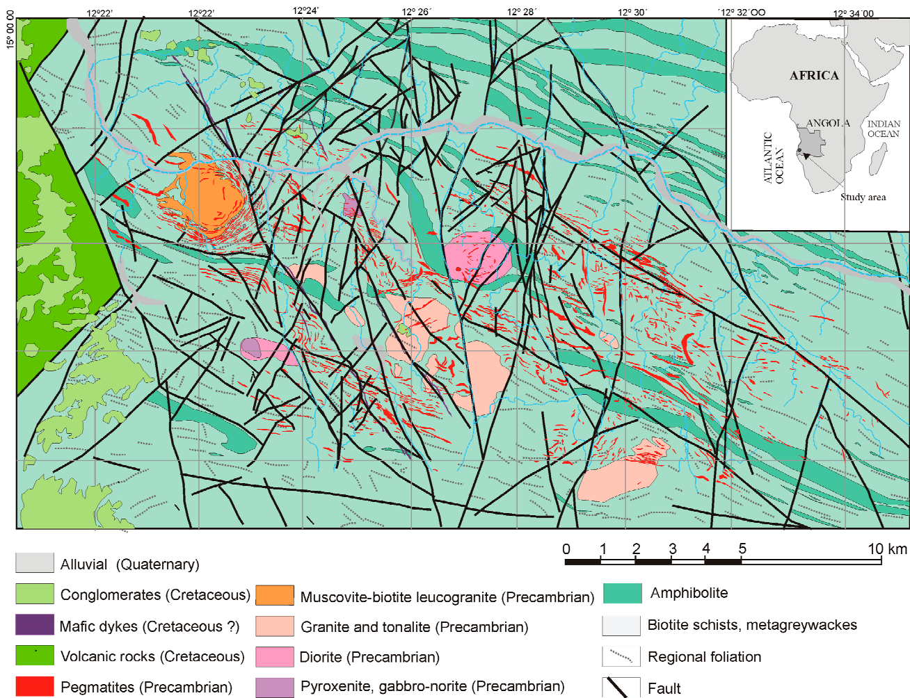
Figure 1. Geological map of the Giraúl pegmatite field.
