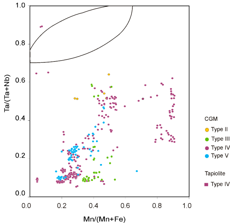
Figure 17. Composition of the CGM (dots) and tapiolite (square) from the Giraúl pegmatites in terms of the columbite quadrilateral (atomic ratios).
