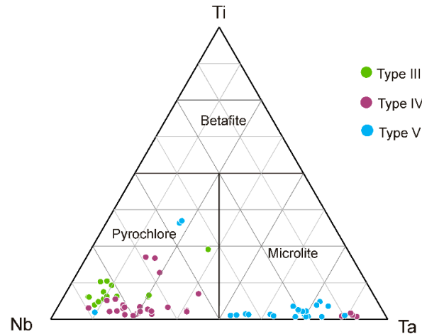
Figure 19. Nb-Ta-Ti compositional plot of the pyrochlore-supergruop minerals from the Giraúl pegmatites. Black solid lines after [45].
