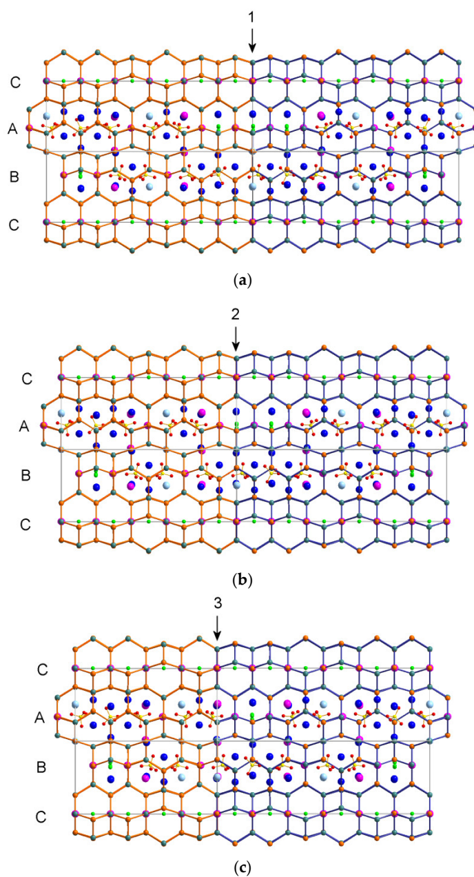
Figure 8. Fragments of the tounkite structure in projection along the [110] axis. The right fragment is rotated relative to the left one by 180^\circ around the c axis. The arrows indicate variants of domain coupling in a twinned crystal (see the text). The letters A, B and C denote the three kinds of layers of tetrahedra. See Figure 7 for legend.
