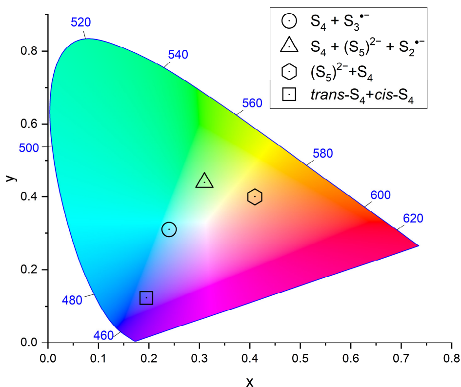
Figure 10. Color space chromaticity diagram of the studied samples' coloration. \text{S}_4 -bearing haiüyne, studied previously [26], contains trans - and cis - \text{S}_4 components. Sulphydrylbystrite [11] contains \text{S}_5^{2-} and minor \text{S}_4 .
