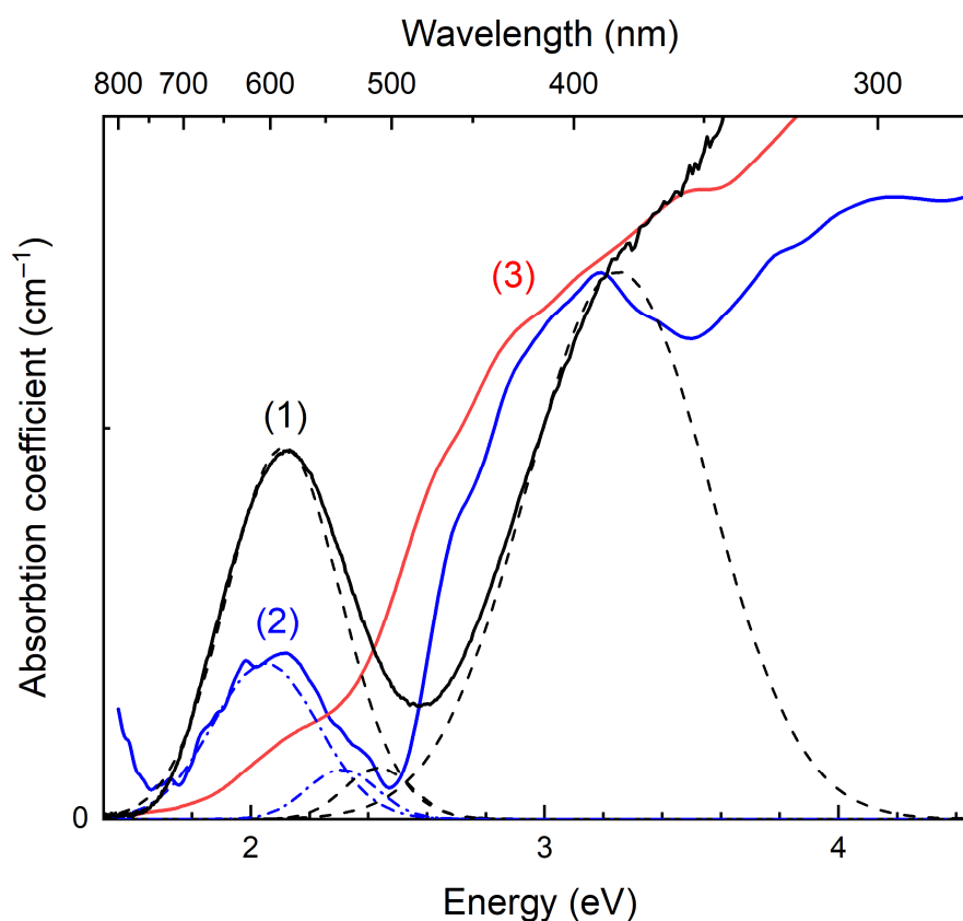
Figure 4. UV–Vis–near-IR absorption spectra of Sample 2 (curve 1), Sample 3 (curve 2) and sulfhydrylbystrite, Na_5K_2Ca(Al_6Si_6O_{24})S_5^{2-}(HS)^- (curve 3). Components of the spectra of Sample 2 and Sample 3 are shown with dashed and dashed-dotted lines, respectively.
