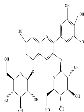
Delphin
