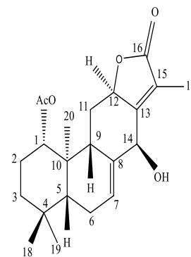
Phorneroids B
