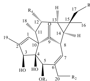
Phonerilins A
