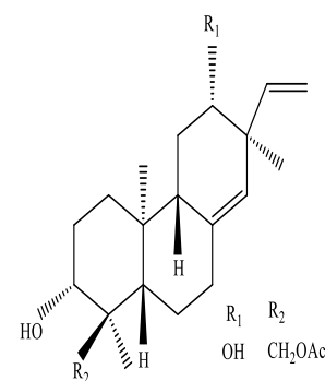
Eurifoloid H
