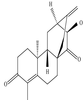
Eurifoloid M
