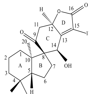
Phorneroids A
