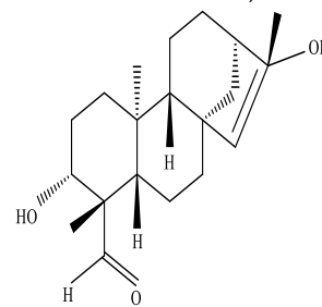
Phorneroids G
