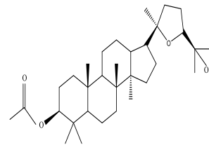
Cabraleadiol monoacetate
