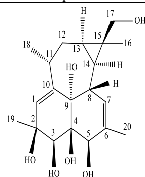
Phonerilins A
