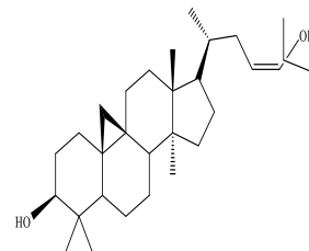
(23Z)-Cycloart-23-ene-3β,25-diol
