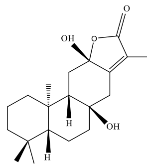
Phorneroids D
