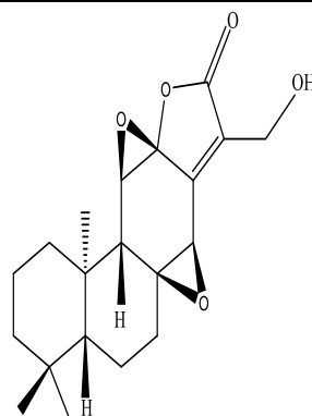
Compound III
