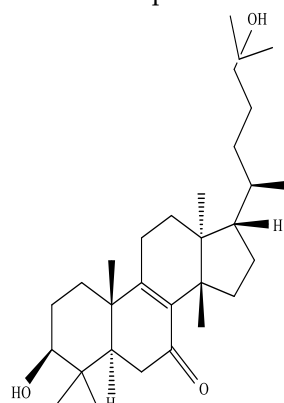
Triterpene
