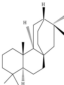
Ent-atisane
