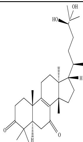
Neritriterpenols G
