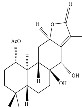
Phorneroids C
