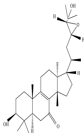
Neritriterpenols F
