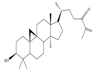
24-Oxocycloart-25-en-3β-ol
