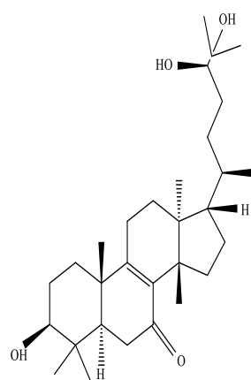
Neritriterpenols D
