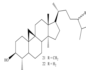
29-Norcycloartanol
