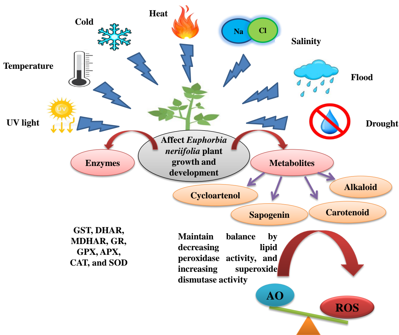
Figure 2. Effect of abiotic stress and plant metabolites on the reactive oxygen species (ROS). (GST: glutathione transferase; DHAR: dehydroascorbate reductase; MDHAR: monodehydroascorbate reductase; GR: glutathione reductase; GPX: glutathione peroxidase; APX: ascorbate peroxidase; CAT: catalase; SOD: superoxide dismutase; AO: antioxidant; ROS: reactive oxygen species).
