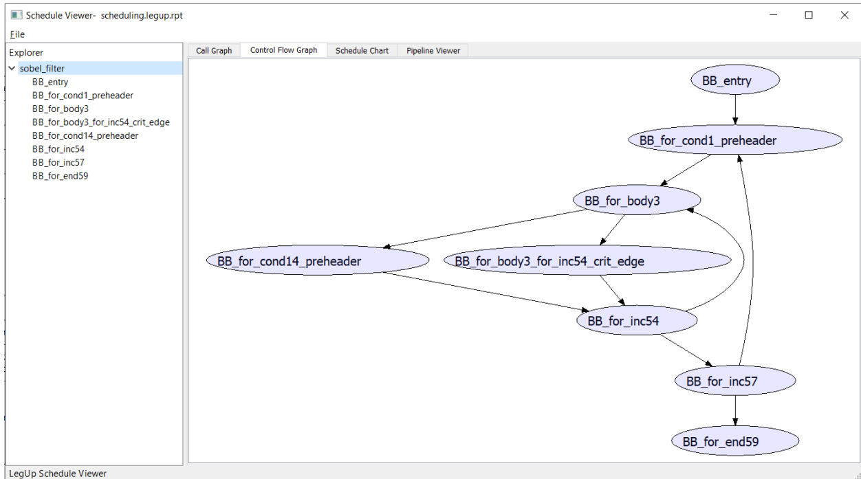
Figure 14: Control-Flow Graph for the Sobel filter.
