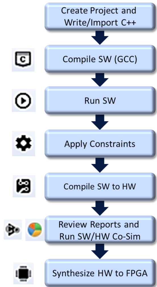
Figure 11: SmartHLS Design Flow Steps
