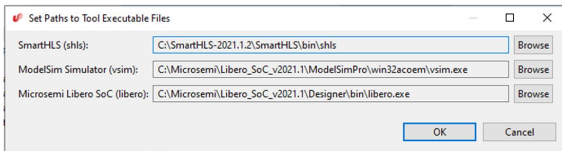
Figure 8: SmartHLS Tool Path Settings.
