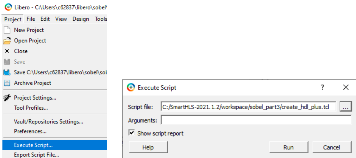
Figure 24: Execute Tcl script to instantiate SmartHLS IP component into SmartDesign.
