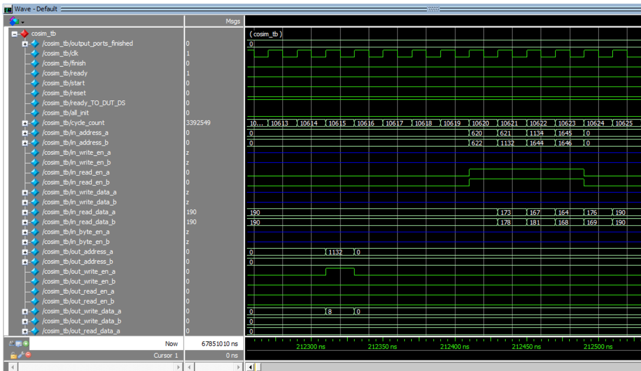
Figure 17: Modelsim waveforms shown during SW/HW Co-Simulation
