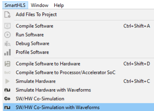
Figure 16: Run SW/HW Co-Simulation with Waveforms
