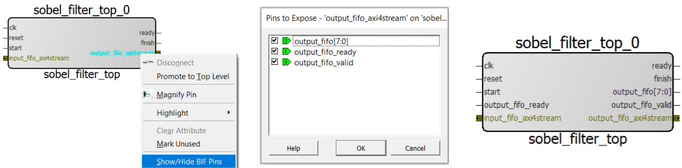
Figure 27: Expose the individual pins contained in the output_fifo AXI4-Stream bus
