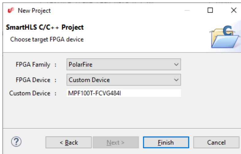
Figure 7: Choose FPGA device
