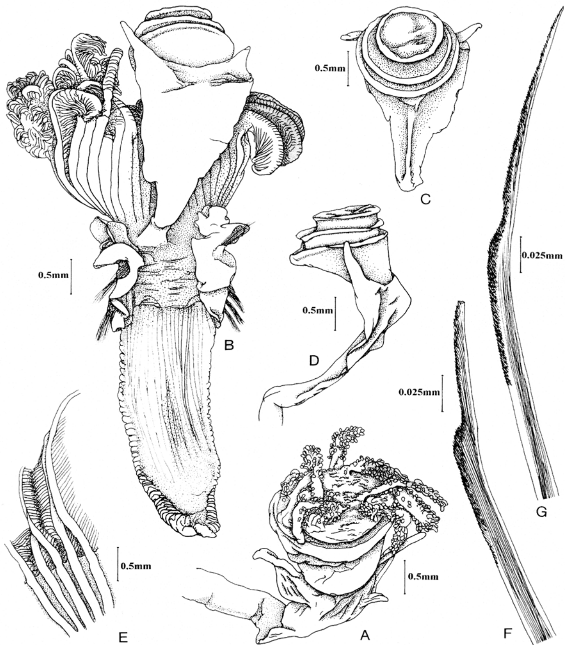
Figure 53. A–G, Spirobranchus murrayi n.sp., from Gulf of Oman, South Arabian coast, Murray Expedition stations 53 & 71, BMNH 1937.9.2.550. (A) operculum of a specimen, with the Hydrozoan Coelenterate Teissiera on its opercular plate; (B) dorsal view of a whole worm; its operculum and peduncle is conspicuously long compared to the rest of the body, and its peduncular wings are unfringed; (C, D) two different views of the 3-tiered operculum of specimen figured in A, also showing the unfringed peduncular wings; (E) some branchial radioles showing the unfringed inter-radiolar membranes; (F, G) bayonet-shaped special collar chaetae showing a squarish boss, an indentation between the boss and the blade, and a corresponding outward bend on the opposite side of the blade, the constancy or otherwise of which needs further investigation. The blade is longer than the serrated distal part of the chaetal shaft plus the boss.
