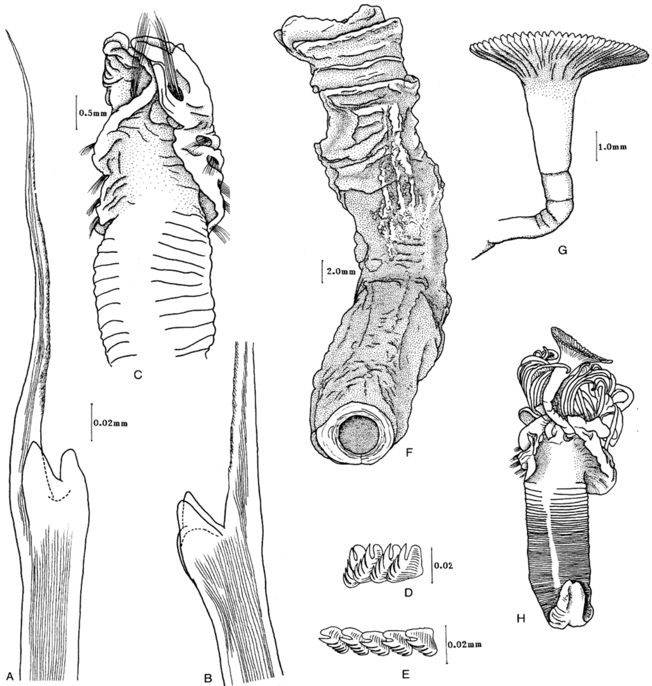
Figure 28. A–E, Serpula amplilobata n.sp., from holotype AM W21410: (A, B) bayonet-shaped collar chaetae; (C) arrangement of anterior abdominal uncinal tori; (D) thoracic uncini; (E) anterior abdominal uncini; F–H, Serpula jukesii Baird, 1865, from AM W21934: (F) tube; (G) lateral view of operculum; (H) arrangement of abdominal uncinal tori.
