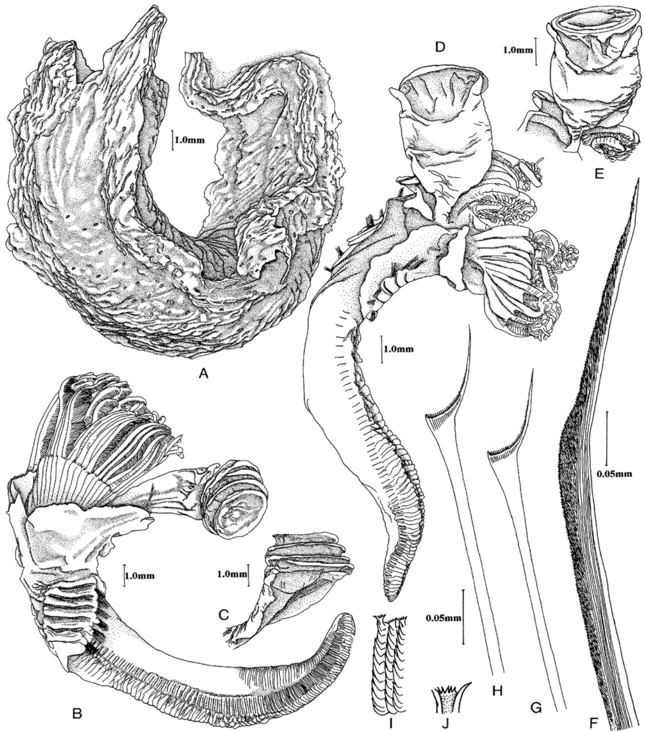
Figure 62. A–J, Spirobranchus zelandicus n.sp., BMNH 1936.2.8.3047–3048, Two specimens, from New Zealand, Discovery Expedition Stn. 941, collected on 20.08.1932. (A) tube of holotype, with tube of a juvenile, paratype, on it. Both are covered over by a thin calcareous encrusting organism having scattered foramina over its surface. A high median longitudinal ridge ends in a conspicuous stout tooth projecting forwards over the aperture in the adult (holotype); yet to be formed in the juvenile tube (paratype); (B) whole worm (holotype), showing its 4-tiered operculum, unfringed inter-radiolar membranes, wide collar and long-shafted abdominal neurochaetae; (C) another view of the 4-tiered operculum of the holotype; (D) whole worm (paratype) with its single-tiered operculum, unfringed peduncular wings and inter-radiolar membranes; (E) operculum of the paratype, another view; (F) bayonet-shaped special collar chaeta showing its boss and the long serrated part of the chaetal shaft preceding the boss. The gradually tapering blade is shorter than the serrated distal part of the chaetal shaft plus boss; boss is not squarish, yet recognizable, smoothly rounded and considerably narrower than blade; (G, H) distal ends of abdominal neurochaetae; (I) thoracic uncini showing serrated gouge; (J) enlarged view of serrated gouge.
