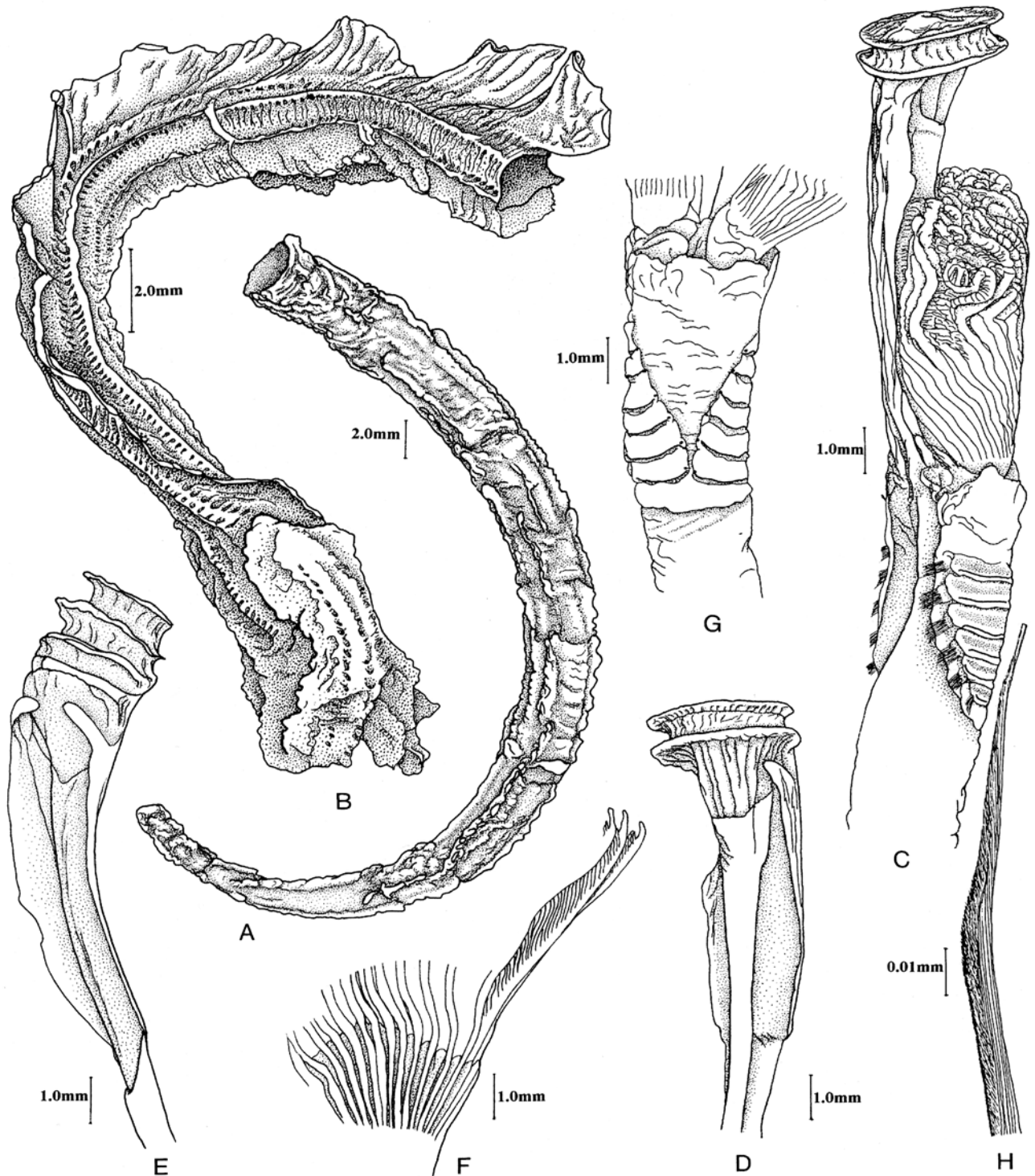
Figure 61. A–H, Spirobranchus tenhovi n.sp., BMNH 1941.3.3.1476, B.A.N.Z.A.R. Expedition, Tasmania Stn. 115, 128 m, labelled Spirobranchus laticapax (Marenz.), but actually containing two genera/species. (A) one of the 8 orange coloured tubes of a Serpula crenata -like species mistakenly included with the new species of Spirobranchus , which also has yellowish-orange tubes. B–H, from holotype and paratype of Spirobranchus tenhovi n.sp; (B) tube of holotype (from which the worm was extracted during the present study); MLR high and consists of forwardly directed fin-shaped sections, most anterior one projecting conspicuously forward beyond the aperture; a row of oblique, forwardly-directed foramina present on either side, at its base. Two, low, narrow, LLRs present on either side of MLR; each also possesses a row of foramina on either side, at its base; (C) dorsolateral view of anterior end of holotype, with a two-tiered operculum; (D) ventrolateral view of latter; (E) left ventrolateral view of paratype showing its four-tiered operculum; (F) part of radiolar crown showing unfringed inter-radiolar membranes; (G) ventral view of thorax of specimen figured in C, showing a dark pigment-spot at the ventral end of each uncinal torus; (H) special collar chaeta; its boss is not squarish but merges gradually between distal end of chaetal shaft and blade; blade is longer than serrated distal part of chaetal shaft plus boss.
