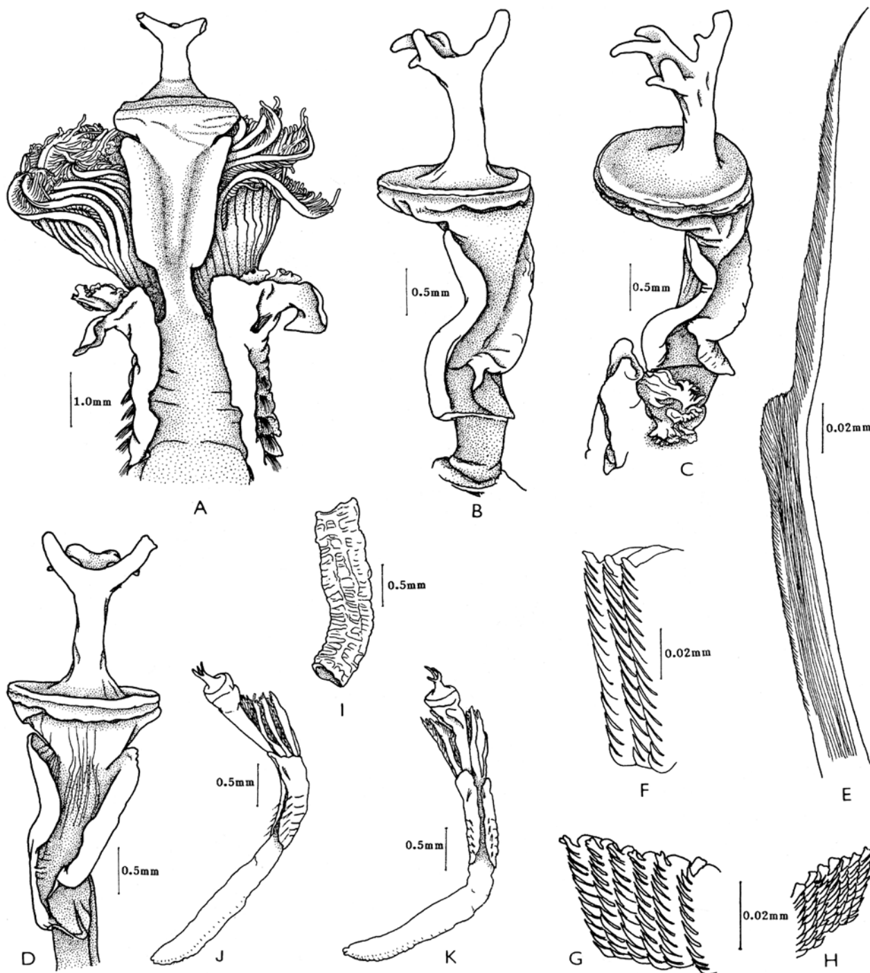
Figure 43. A–H, Spirobranchus richardsmithi n.sp. A–H, from aberrant specimens in AM W21433: (A) anterior end of worm showing opercular disc and processes, unfringed opercular wings and pinnule-free tips of radioles; (B–D) three views of the operculum of another specimen showing the circular opercular disc, abnormal opercular processes, and unfringed opercular wings; (E) bayonet collar chaeta; (F) thoracic uncini; (G) anterior abdominal uncini; (H) posterior abdominal uncini. I–K, early juveniles of Spirobranchus richardsmithi , from AM W21442. I, J, from smallest specimen: (I) dorsal view of tube with worm in situ , showing the single median longitudinal ridge and fine transverse ridges on the tube and the anterior end of the worm; (J) right dorsolateral view of operculum; (K) dorsal view of another juvenile showing left anterolateral view operculum.
