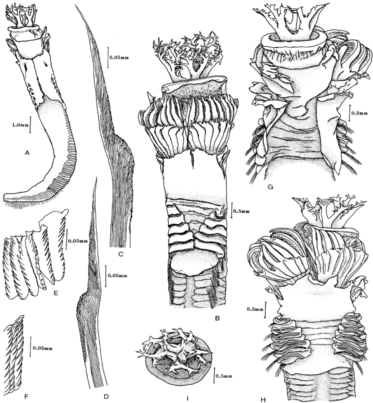
Figure 45. A–I, Spirobranchus tetracerus (Schmarda, 1861). A,B, a worm from AM W21441: (A) dorsal view of whole worm; (B) ventral view of anterior end of the latter worm; shows the branched horns, mottled ventral side of peduncle, fringed interbranchial membranes, pinnule-free radiolar tips, raised uncinal pads, the last two meeting mid-ventrally and the apron which is contracted into a triangular lobe, since the worm was fixed within its tube, and the long-shafted abdominal chaetae. C–F, chaetae from same specimen: (C,D) bayonet-shaped special collar chaetae; (E,F) thoracic uncini. G–I, a specimen from AM W21441: (G) dorsal view of anterior end, highly contracted, showing fringed opercular wings and fringed inter-radiolar membrane; (H) ventral view of anterior end showing inter-radiolar membranes, ventral lobe of collar, thoracic tori not meeting ventrally since the worm was evidently fixed outside its tube, the apron, and anterior abdominal chaetae with long shafts; (I) opercular spines viewed from the anterior end showing three main horns.
