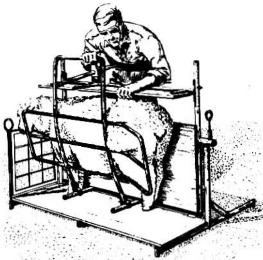
Figure 5.—Tilting squeeze for sheep. (USDA Plan 6006)
