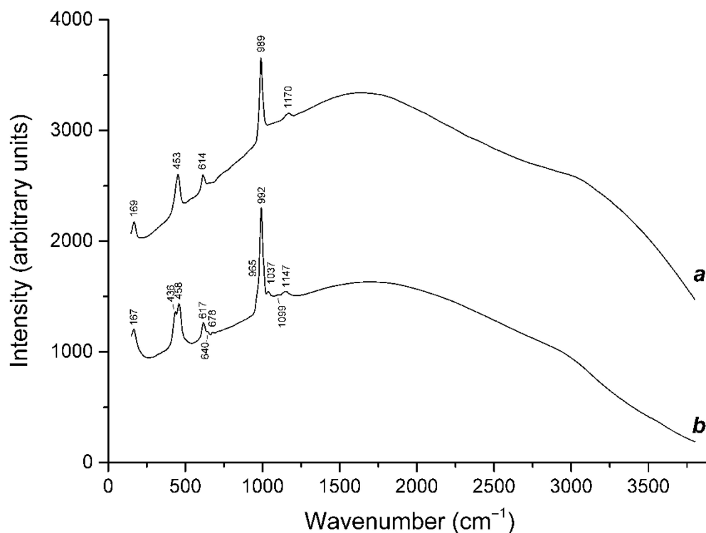
Figure 21. Raman spectra of (a) biachellaite (Sample 14) and (b) \text{SO}_3^{2-} -bearing analogue of marinellite (Sample 13a).
