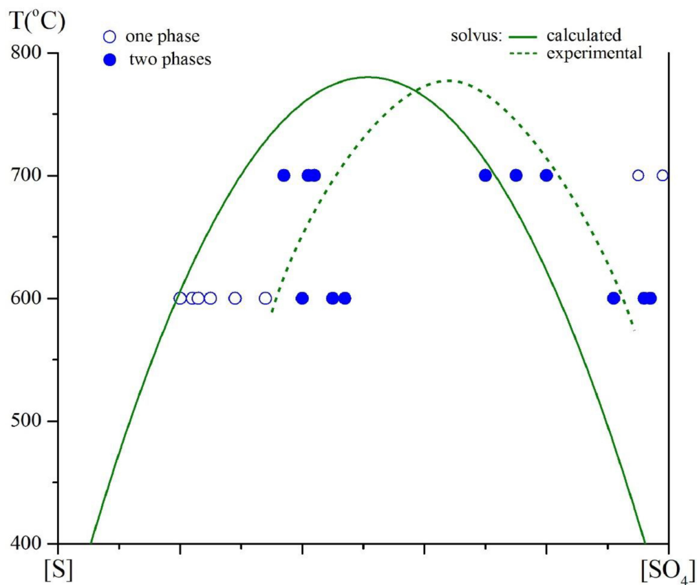
Figure 15. Calculated miscibility diagram in the Ca-bearing S-sodalite–häuyne system and experimental data.
