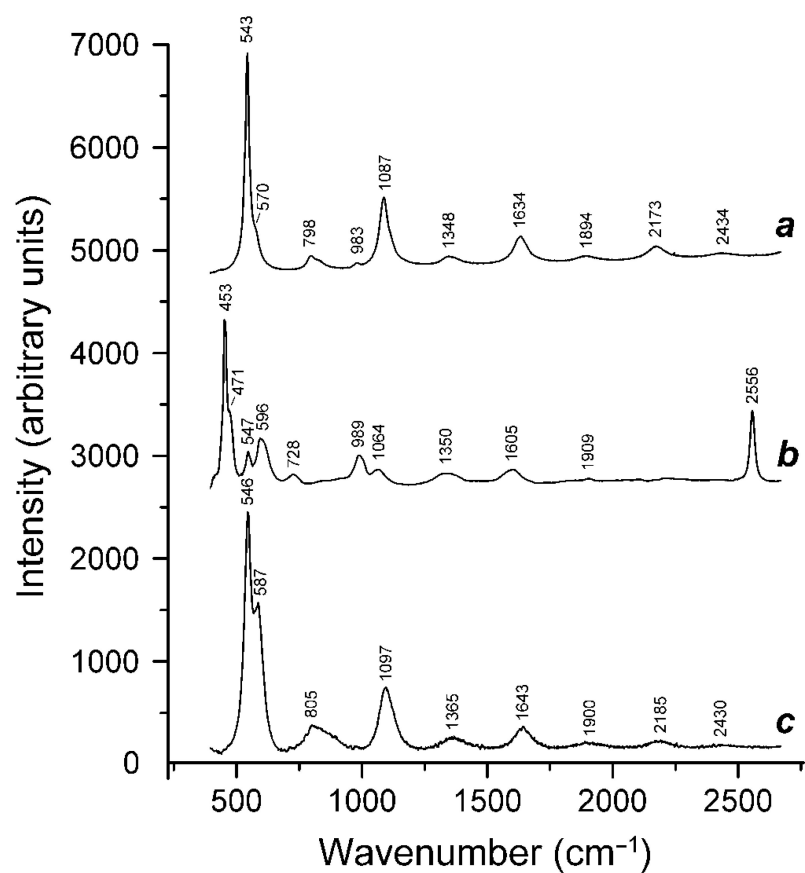
Figure 13. Raman spectra of (a) initial \text{S}_4 -bearing haüyne (Sample 5), (b) Sample 5 preheated for three days at 700 °C, over the Fe-FeS buffer and (c) preheated Sample 5 additionally annealed at 800 °C in air for one day.
