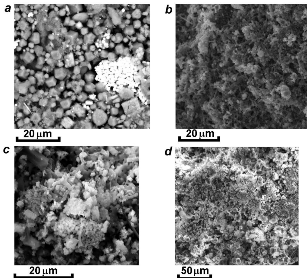
Figure 26. Aggregates of (a) synthetic analogue of sapoznikovite obtained in Experiment 1, (b) intimate intergrowth of sodalite- and cancrinite-type phases mixture from Experiment 2, (c) product of Experiment 2a and (d) cancrinite-type phase from the Experiment 6. SEM photos obtained in the BSE (a) and SE (b–d) modes.
