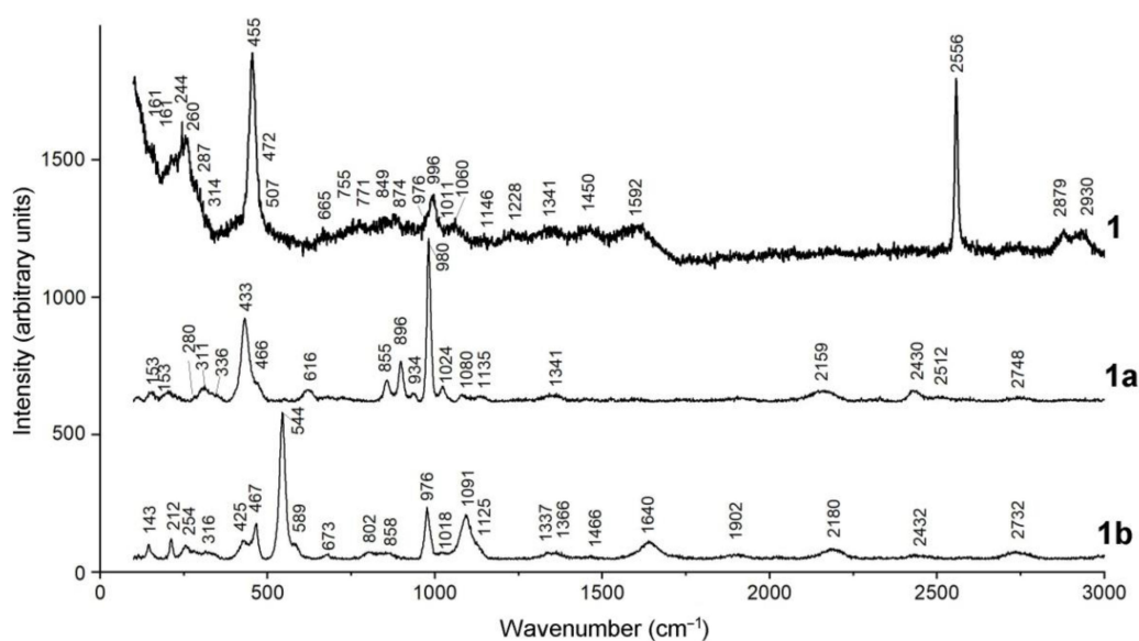
Figure 27. Raman spectra of powders obtained in Experiments 1, 1a and 1b. The description of the experimental conditions is given in Table 4.
