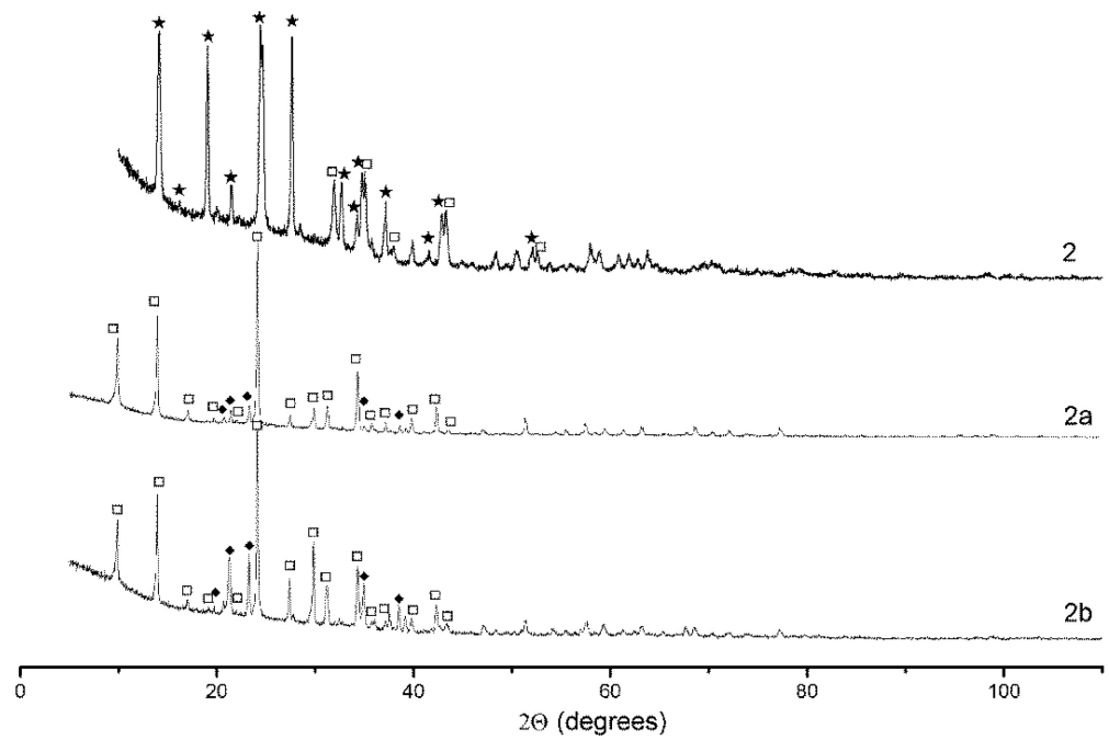
Figure 30. Powder X-ray diffraction patterns of the products of Experiments 2, 2a and 2b. The characteristic non-overlapping reflections of cancrinite-type (□), sodalite-type (★) and nepheline-type (◆) phases are indicated.
