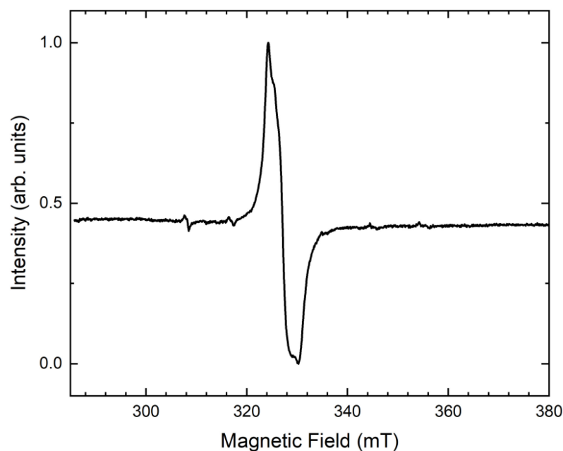
Figure 20. The ESR spectrum of vladimirivanovite (Sample 7).
