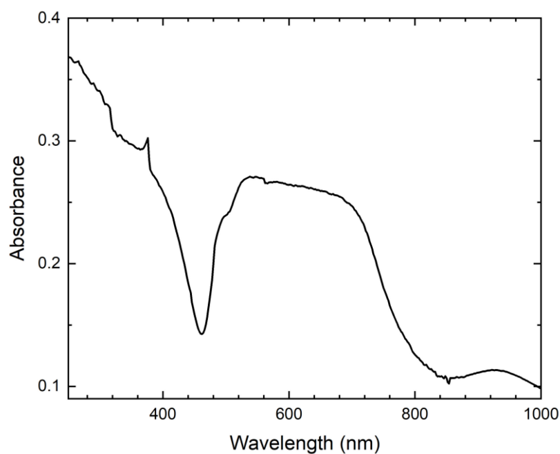
Figure 19. The absorption spectrum of vladimirivanovite (Sample 7).
