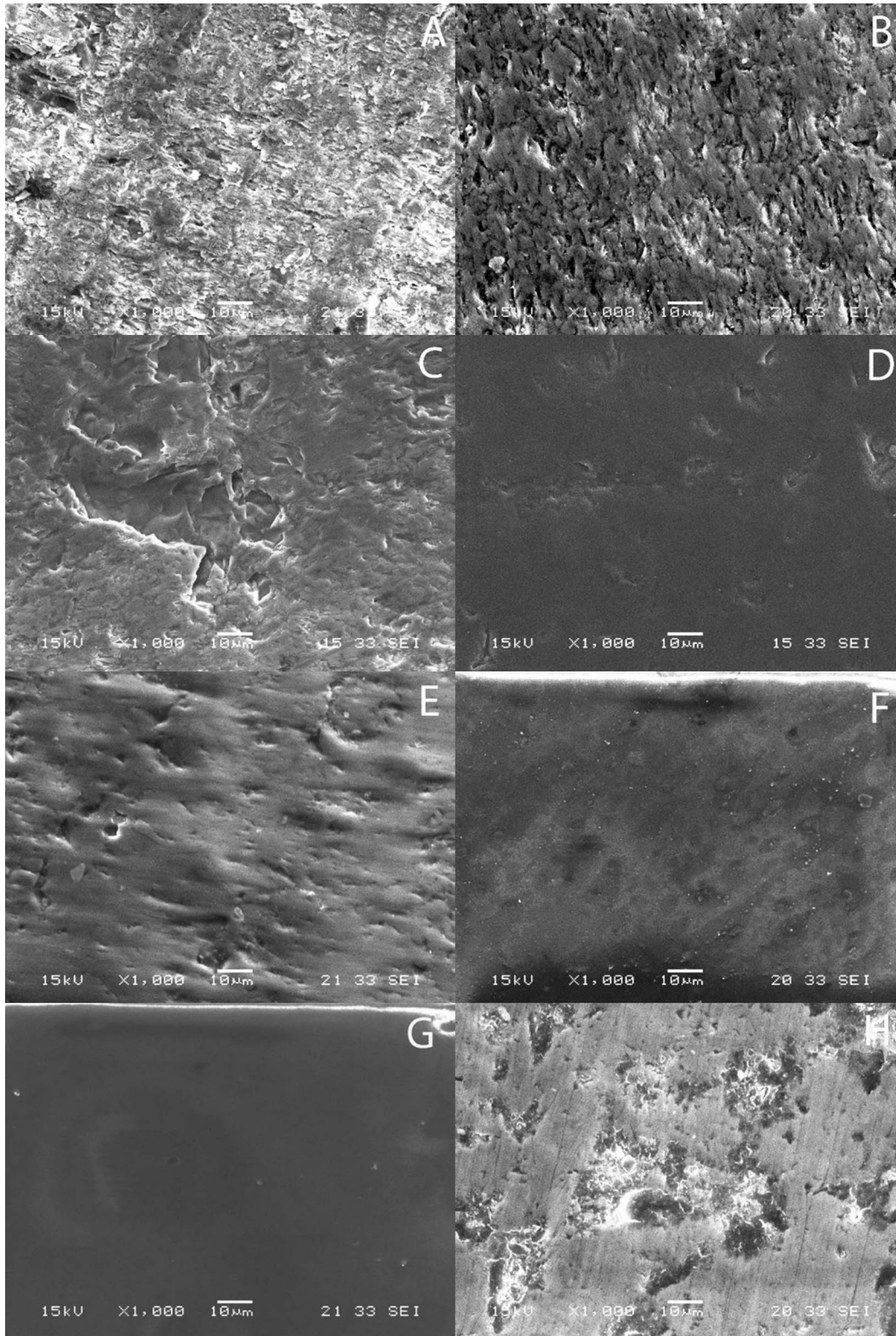
Figure 4. (A-H): Scanning electron micrograph at 1000 \times of the different porcelain surfaces analyzed. (A): Baseline specimen. (B): Identoflex NG-Porcelain Polisher (INP). (C): Identoflex Diamond Ceramic Polisher (IDP). (D): HiLuster Polishing System (HPS). (E): Opra-Fine (OP). (F): Identoflex Lucent (IL). (G): Vita Akzent Glaze Spray (AGS). (H): Vita Shading Paste and Liquid (SPL).
