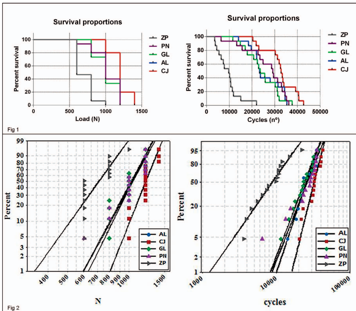
Figure 1. Survival curves according to the steps of load (A, B) and number of cycles (C, D) in which each crown failed. Figure 2. Weibull analysis according to the steps of load (A) and number of cycles (B) in which each crown failed.
