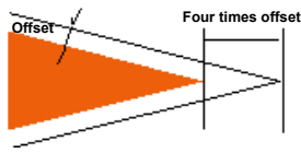
When corner factor = 4: The cut line's corner is projected out to a distance from the object's corner that is equal to four times the offset. (In this figure, cutting-off of the line's corner stops being applied at factor 4, and setting a corner factor that is any higher than this will have no further effect on the shape.)
