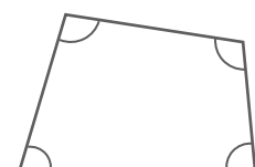
Trubbig vinkel
