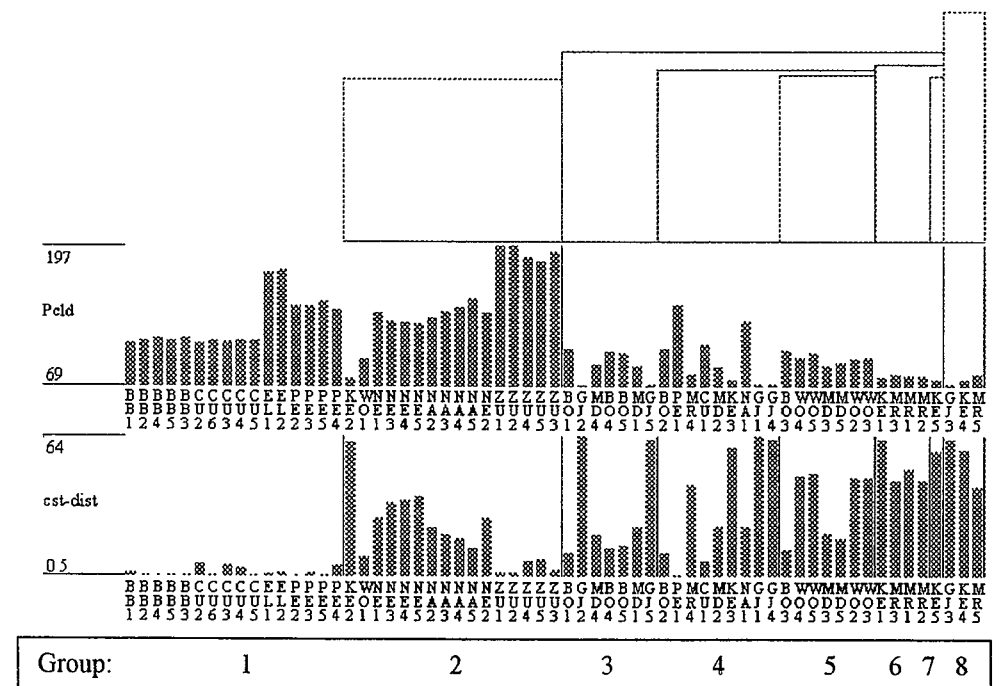
Figure 8 Attribute values for 'precipitation in the coldest quarter' (Pcld) and 'distance to coast' (cst-dist) superimposed as histograms on the dendrogram structure derived from the classification of the 63 quadrats in terms of species belonging to assemblage-11. Quadrat codes are printed vertically. The relevant re-ordered data matrix is provided in Figure 12.
