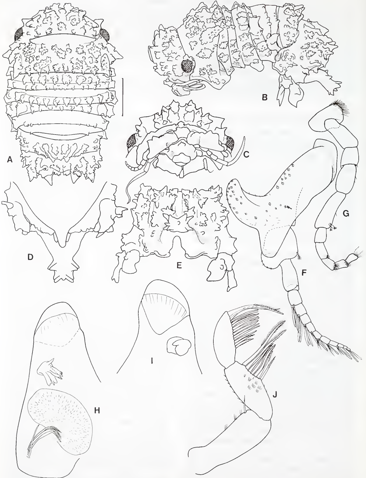
Figure 18. Cercosphaera wirritin sp. nov. A-E holotype, remainder \delta paratype 4.5 mm, AM P41121. A, dorsal view; B, lateral view; C, frons; D, pleotelson, ventral view; E, pleotelson, posterior view; F, antennule; G, antenna; H, right mandible; I, left mandible; J, mandible palp. Scale 1.0 mm.
