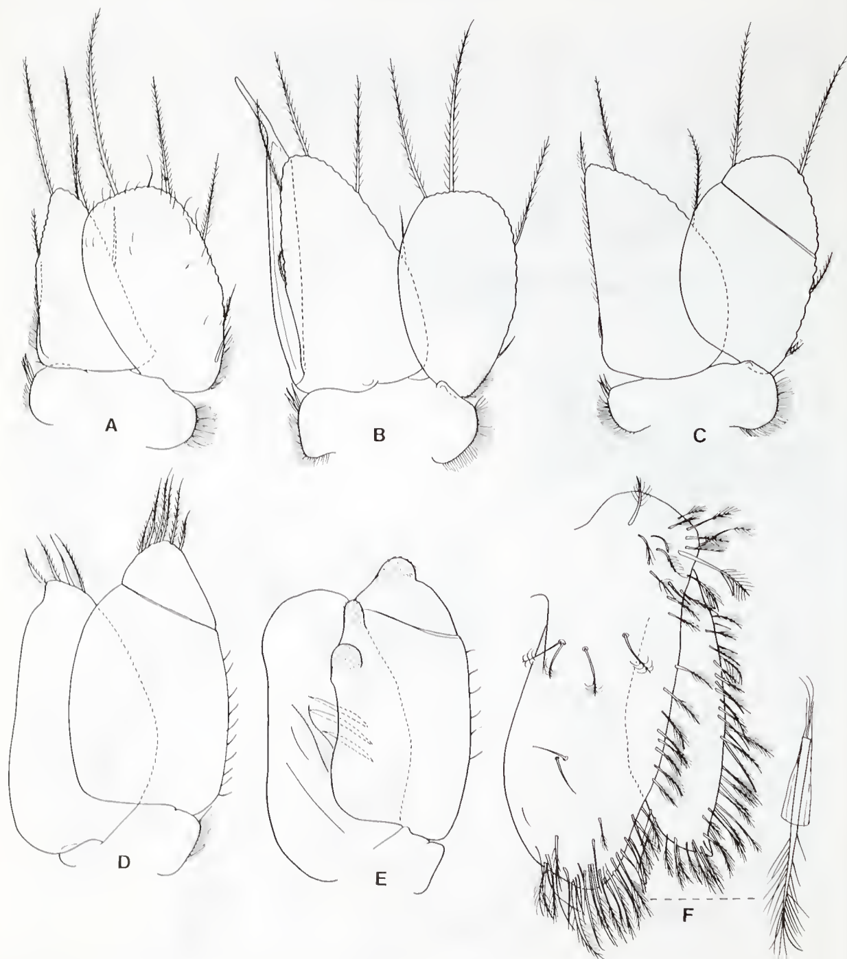
Figure 4. Benthosphaera arkoala sp. nov. All figs \delta 5.0 mm, NMV J19162. A-E, pleopods 1-5, respectively; F, uropod.
