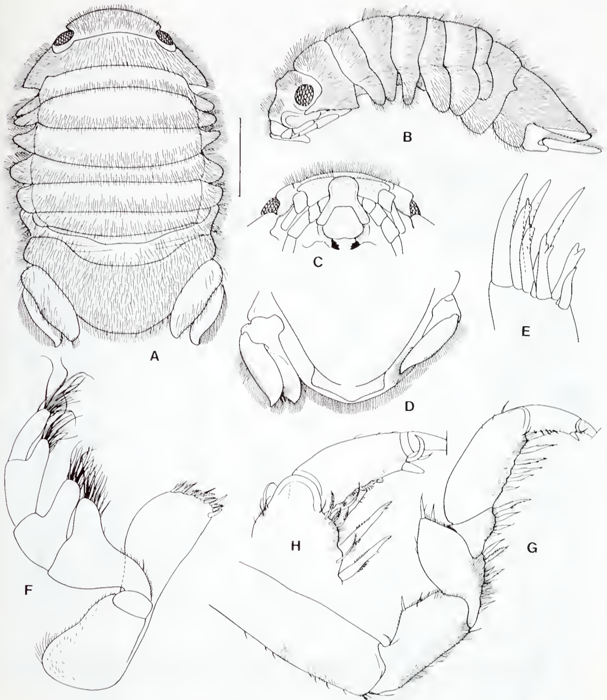
Figure 6. Benthosphaera reburra sp. nov., holotype. A, dorsal view; B, lateral view; C, frons; D, pleon, ventral view; E, maxillule, apex of lateral lobe; F, maxilliped; G, pereopod I; H, pereopod I dactylus. Scale 2.0 mm.
