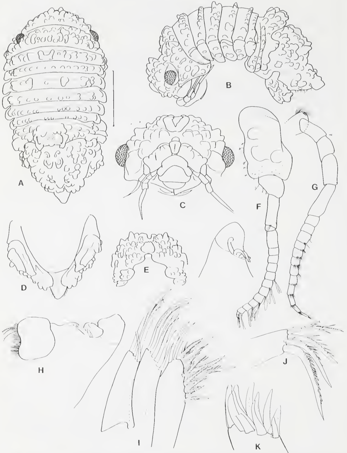
Figure 27. Cercosphaera coloura sp. nov. A-F holotype, remainder paratype, SAM C5544. A, dorsal view; B, lateral view; C, frons; D, pleon, ventral view; E, pleon, posterior view; F, antennule; G, antenna; H, left mandible; I, right mandible; J, maxilla; K, maxillule endopod; L, maxillule, exopod. Scale 2.0 mm.
