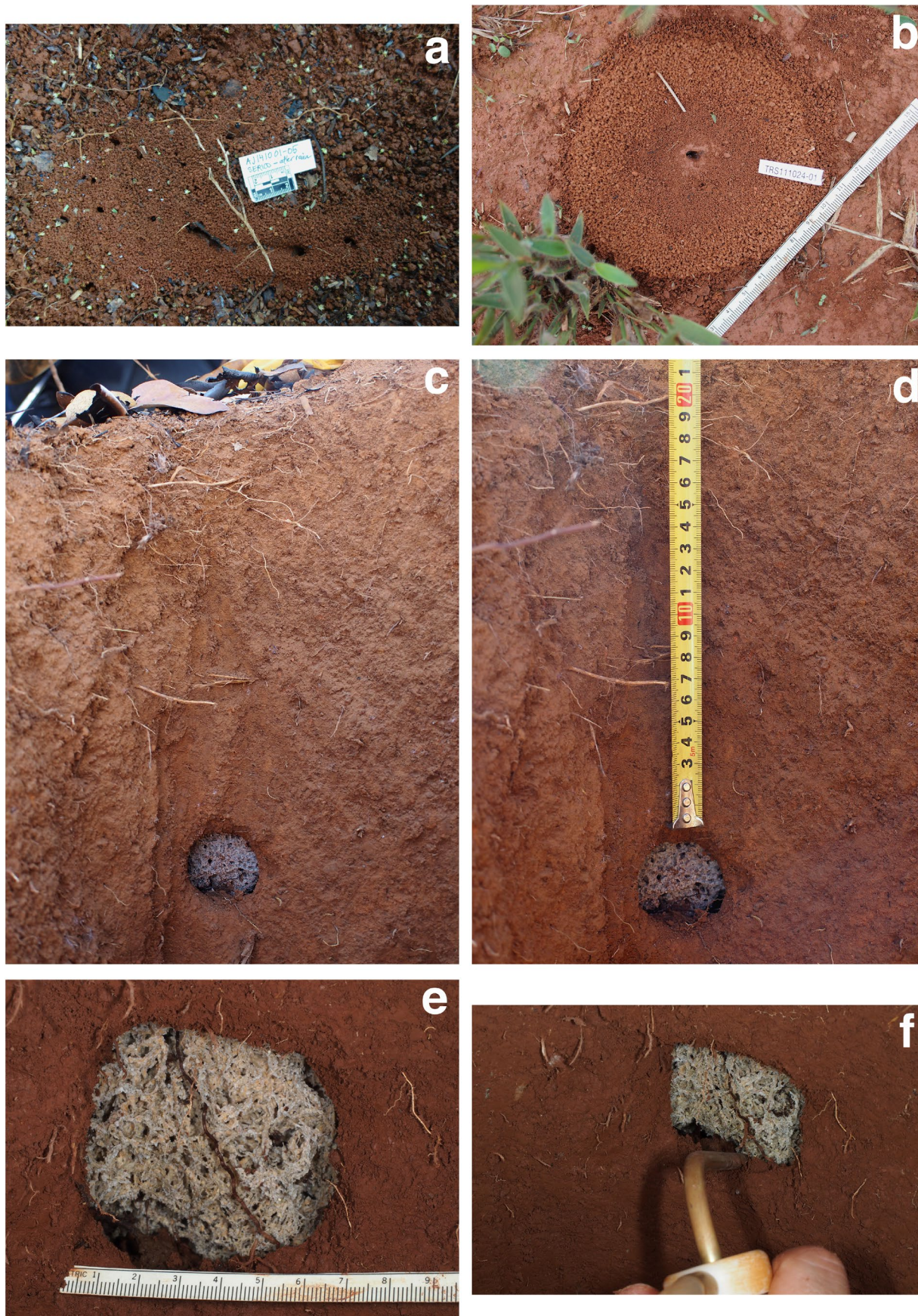
Fig 1. Nests of ground-nesting non-leaf-cutting fungus-farming ants. a. Nest entrance of Sericomyrmex sp. (AJ141001–05) with multiple entrances after rain. b. Nest entrance of Myrmicocrypta sp (TRS111024–01) with small single entrance surrounded by circular dirt mount. c. Subterranean subspherical garden chamber of Myrmicocrypta sp. d. Subterranean garden chamber of Myrmicocrypta sp. with depth record (see text). e. Subterranean chamber of Apterostigma sp. f. Subterranean chamber of Apterostigma sp. demonstrating collection of ants with receptacle aspirator.
