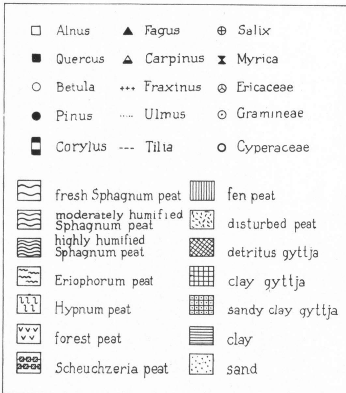
Fig. 2. Key to symbols for pollen diagrams.
