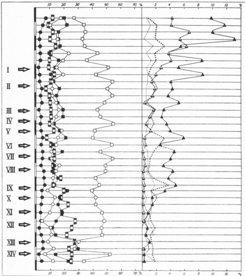
Fig. 25. In this diagram the position is indicated of the Grenzhorizont in the profiles summed up on the opposite page. The Roman figures left of the diagram correspond with those of the profiles.
