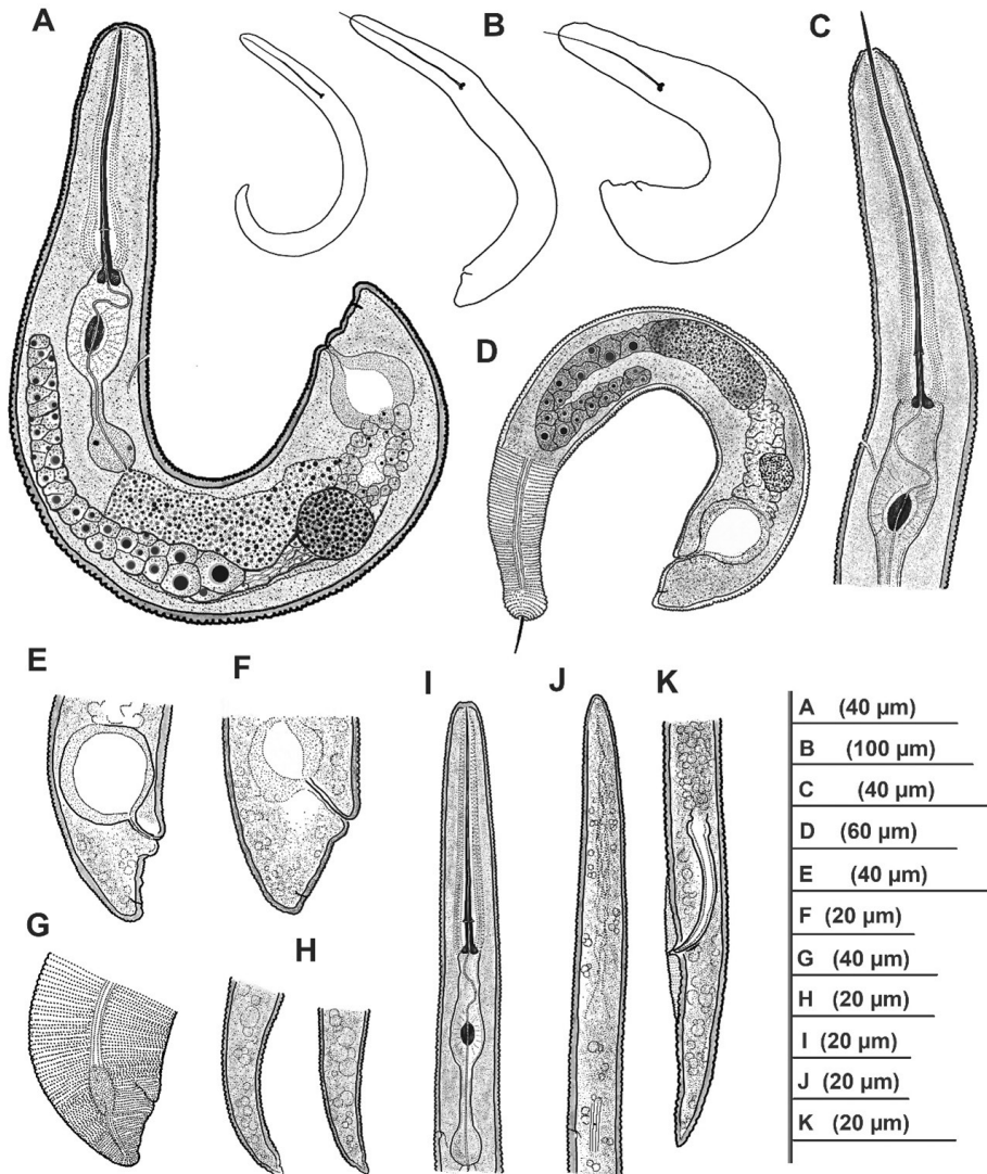
Figure 3: Line illustrations of Paratylenchus ilicis n. sp. paratypes. A, B, D: Total bodies showing developmental stages from juvenile (J2) to slightly obese to fully obese females; C: Anterior region of female showing stylet, pharynx, and SE pore position; E–G: Tail regions showing vulva, lateral field differentiation, tail shape, and tips of females; H: Tails of J2; I: Anterior region of J2; J: Anterior region of male; K: Posterior region of male. SE pore: secretory-excretory pore.
