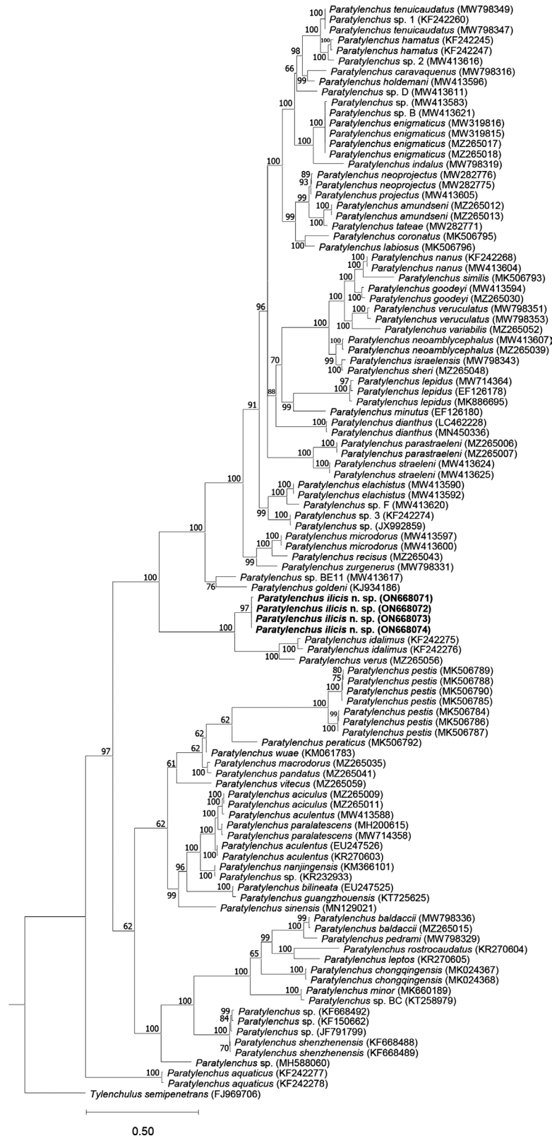
Figure 5: Phylogenetic tree generated using BI based on alignment of ITS rRNA gene sequences of Paratylenchus species using the GTR + G + I nucleotide substitution model. Bayesian posterior probabilities (in percentage) are given next to each node and sequences of Paratylenchus ilicis n. sp. are highlighted. BI: Bayesian inference.
