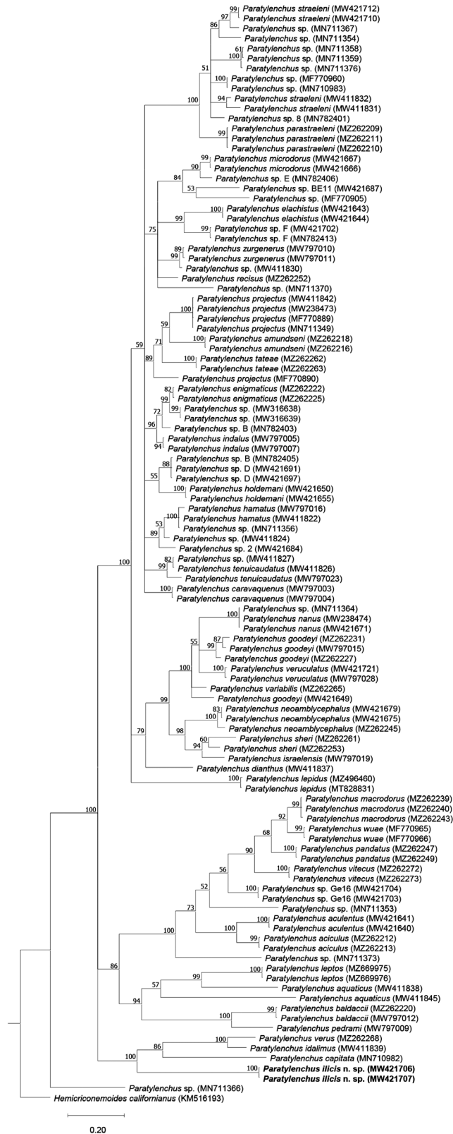
Figure 6: Phylogenetic tree generated using BI based on alignment of cox1 gene sequences of Paratylenchus species using the GTR + G + I nucleotide substitution model. Bayesian posterior probabilities (in percentage) are given next to each node and sequences of Paratylenchus illicis n. sp. are highlighted. BI: Bayesian inference.
