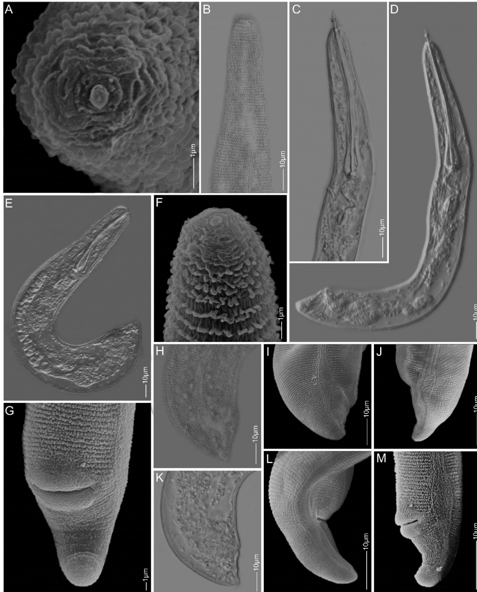
Figure 1: Light and SEM images of Paratylenchus ilicis n. sp. paratype females. A: En face ; B, C, F: Anterior regions showing cuticular ornamentation, stylet, pharynx, and SE pore position; D–E: Total body of (slightly) obese bodies showing major internal structures; G–M: Tail regions showing lateral field, vulva, and tail termini. SE pore: secretory-excretory pore; SEM: scanning electron microscopy.
