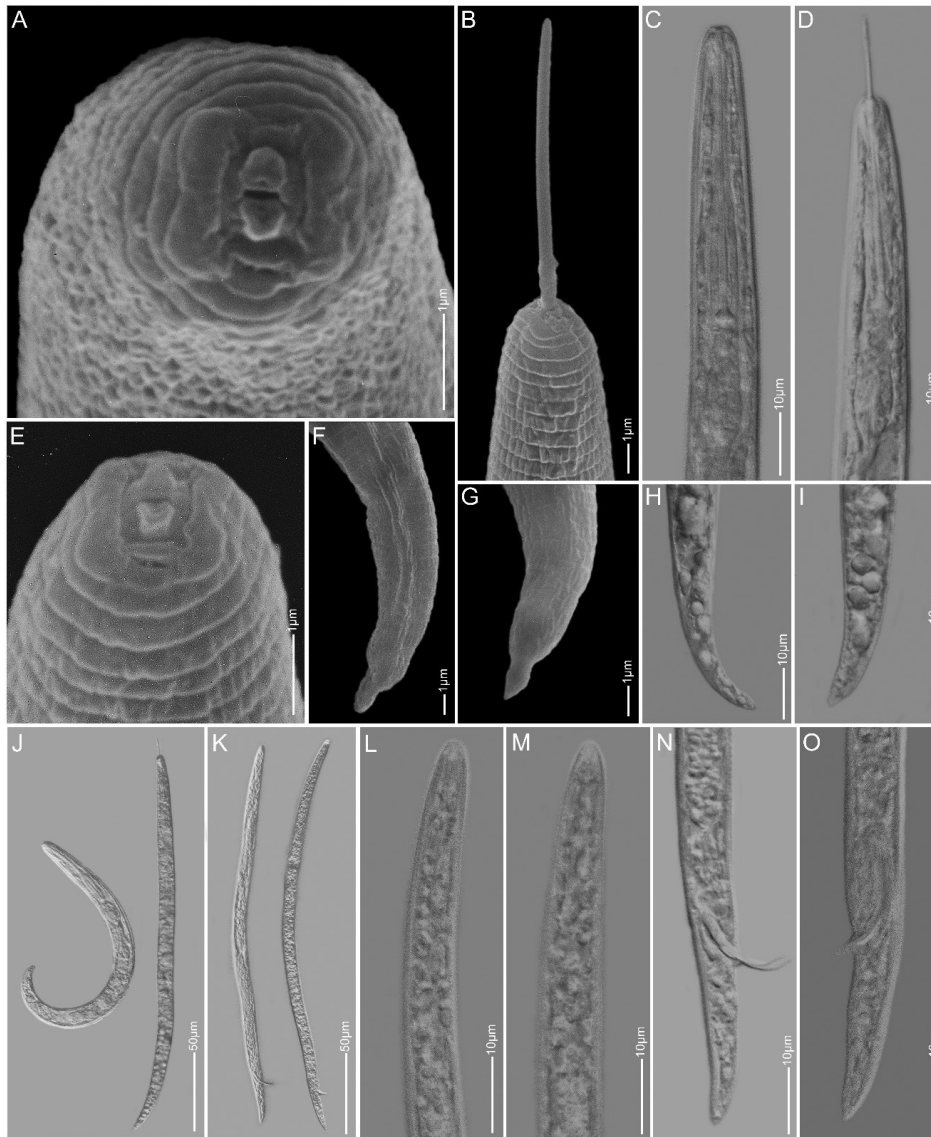
Figure 2: Light and SEM images of Paratylenchus ilicis n. sp. paratype juveniles (J2) and males. A, E: en face of J2; B–D: Anterior regions showing stylet and pharynx of J2; F–I: Tail regions showing characteristic finger-like tip of J2; J: Total bodies of J2; K: Total bodies of males; L–M: Anterior regions of males showing absence of stylet; N–O: Tail regions showing spicules. SEM: scanning electron microscopy.
