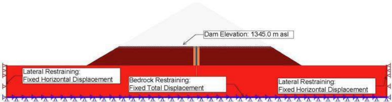
Figure 4.3.3.2. Stress-deformation analysis: first stage of impounding
