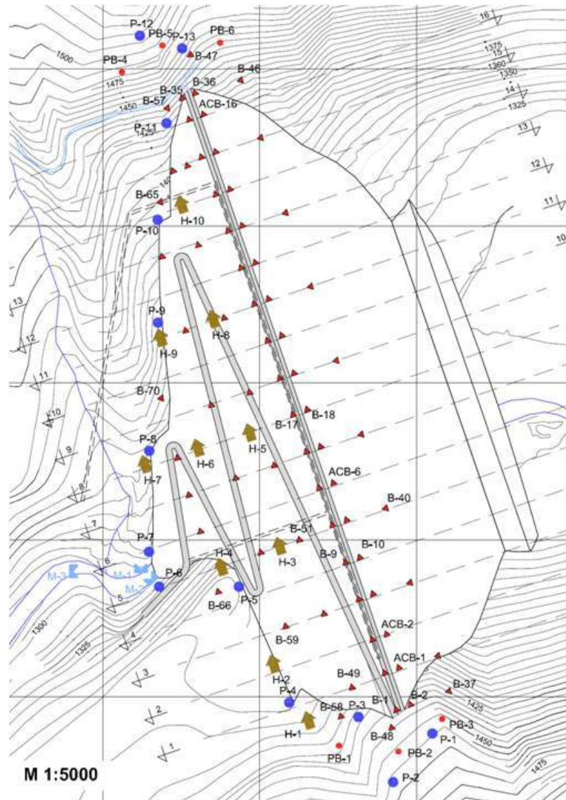
Figure 4.2.4. Layout plan of control-measuring systems of Nenskra dam
