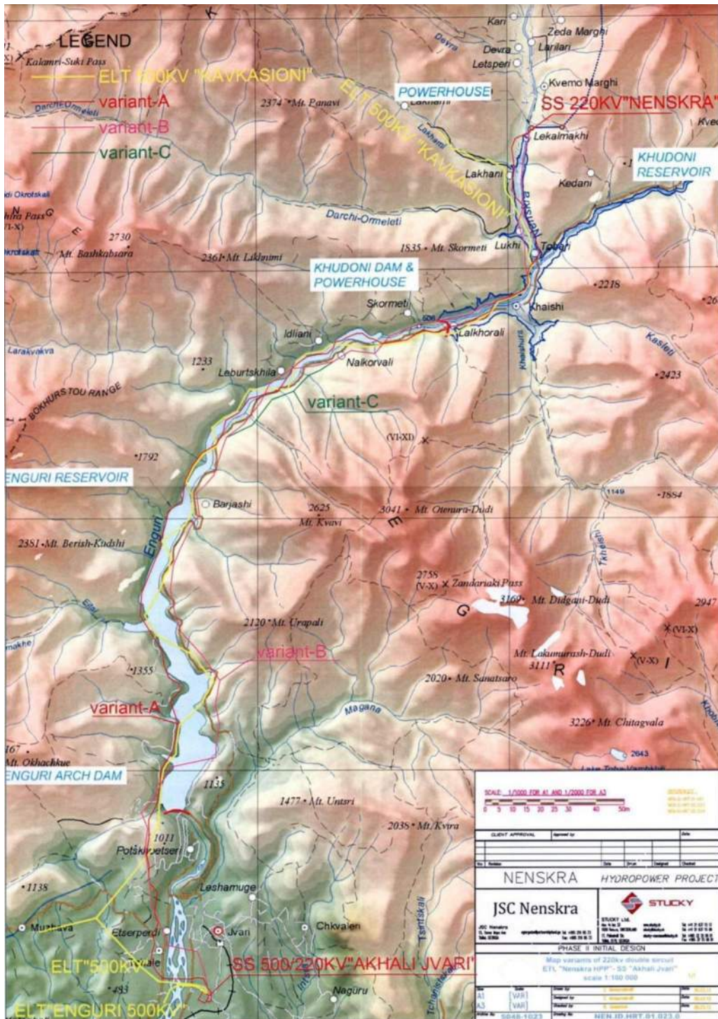
Figure 4.6.1. Scheme of alternatives of transmission lines
