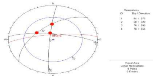
Analysis against to Wedge Failure;
