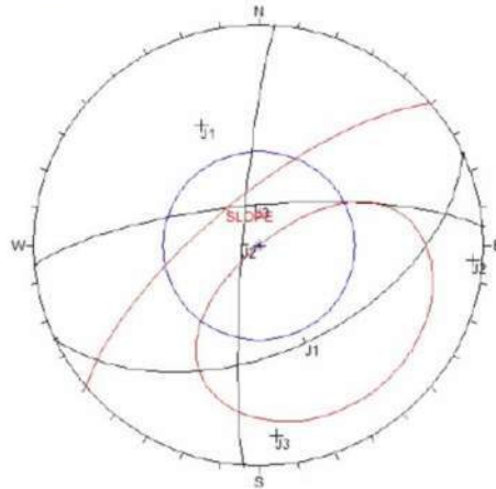
Figure 5.2.3.6.1.5.1. The kinematic analysis of left bank of dam axis
