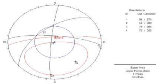
Analysis against to Planer Slip;
