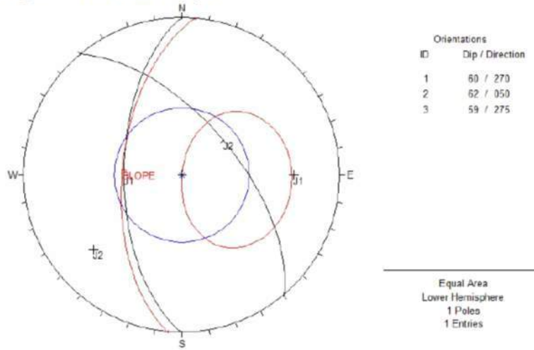
Figure 5.2.3.6.4.4.1. The kinematic analysis of outlet portal of the Nakra tailrace tunnel
