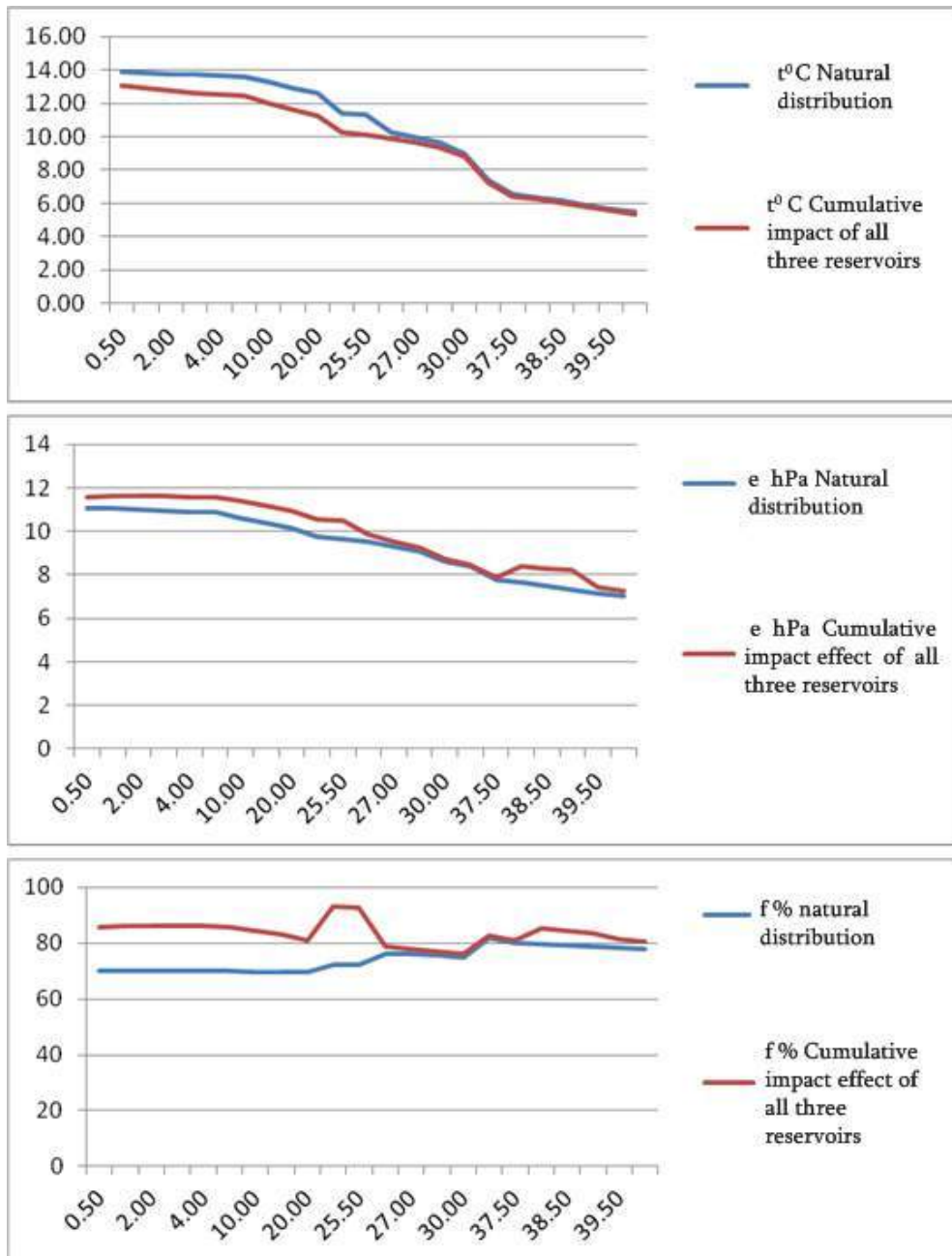
Figure 13.1.2. Transformation of temperature (a), partial pressure (b) and relative humidity (c) caused by Jvari, Khudoni and Nenskra impact for Z=2m height.
