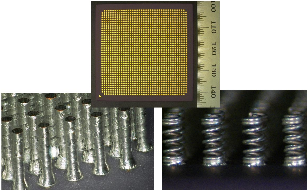
Figure 3. Land grid array (LGA) before column attachment (top) and after both copper-wrapped solder column attachment (left) and microspring attachment (right).
