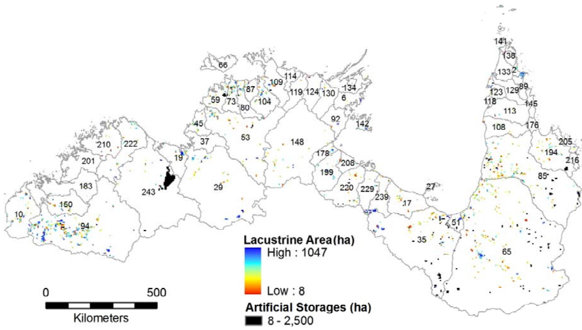
Figure 3.4. The area in hectares of lacustrine aquatic systems in 5 km 2 grids across northern Australia
