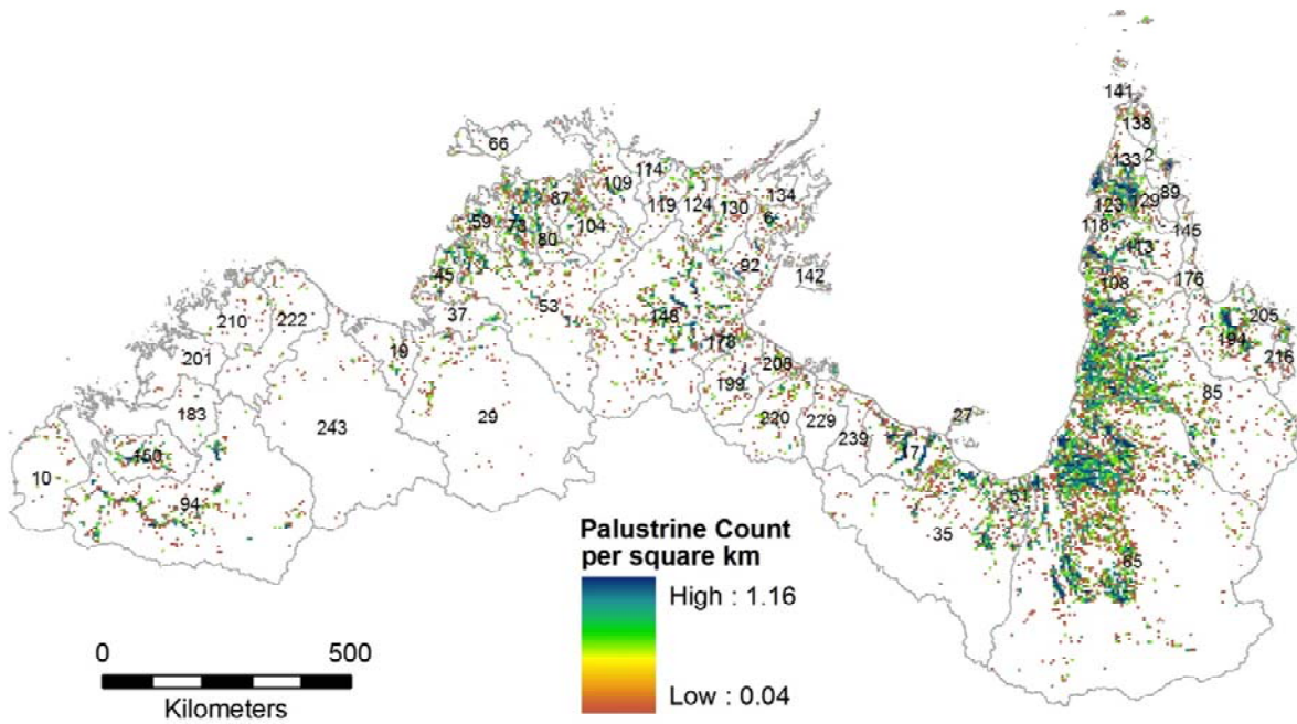
Figure 3.3. The number of palustrine aquatic systems per km 2 across northern Australia.
