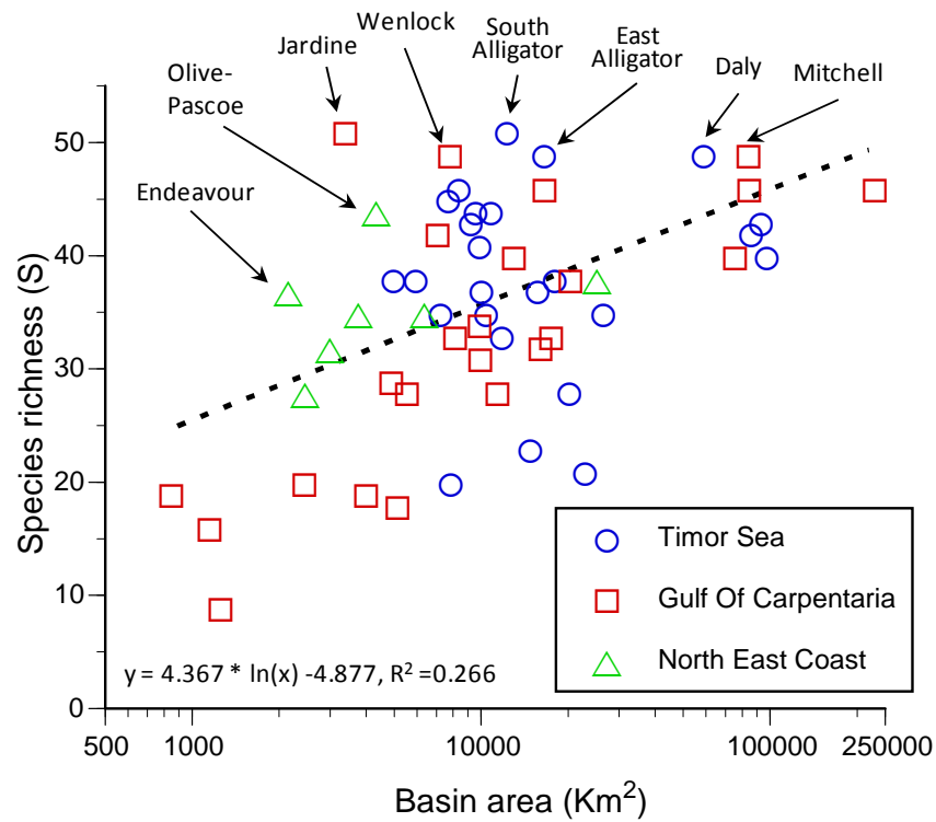
Figure 3.11. Fish species richness versus basin area (Km 2 ) for river basins of northern Australia.
