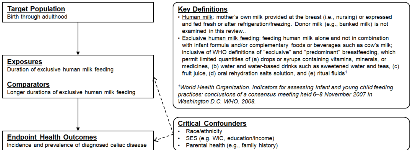
Figure 1: Analytic framework
