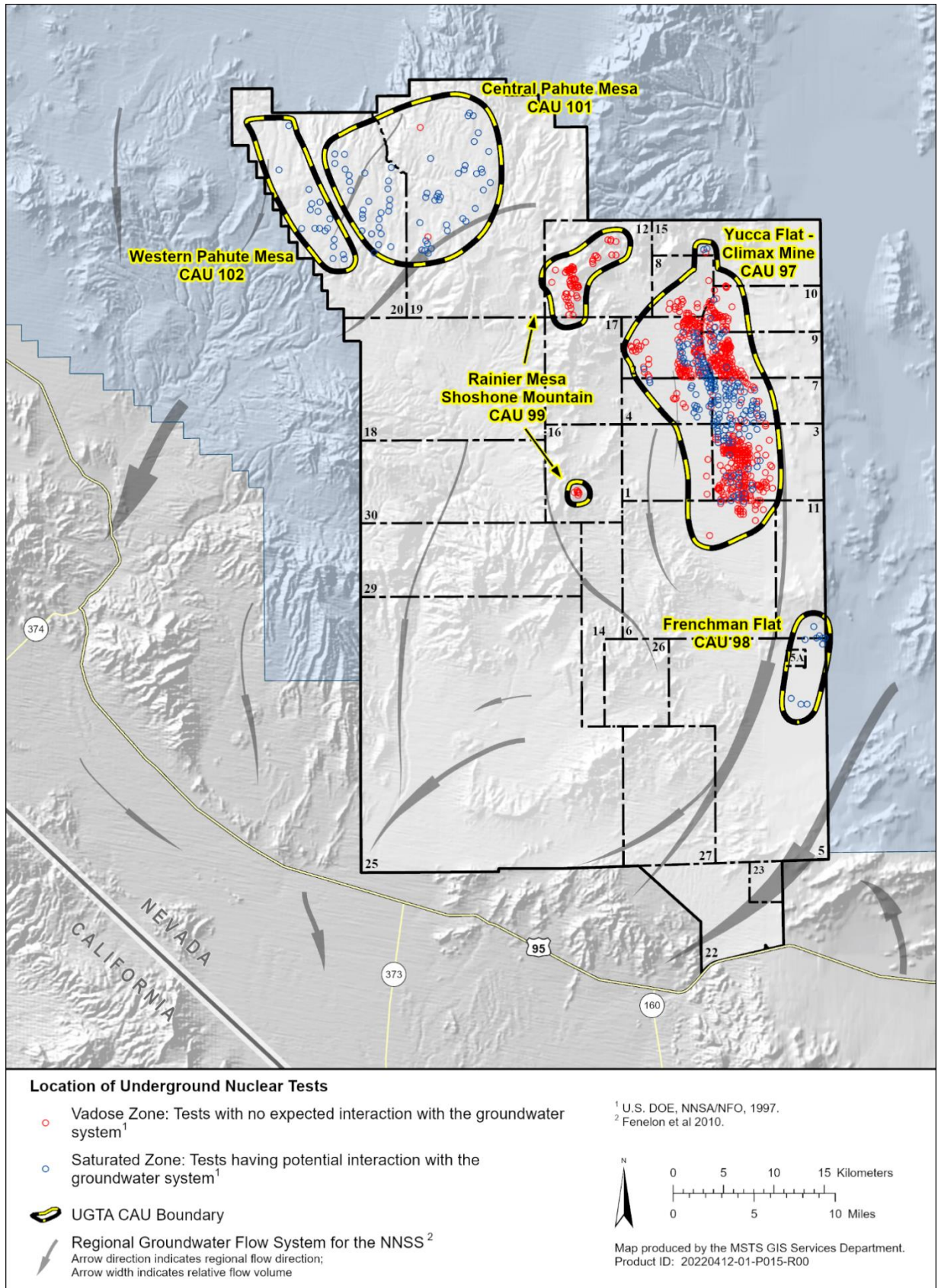
Figure A-7. Locations of UGTA CAUs and historical underground nuclear tests (not including test locations at Buckboard Mesa [Area 18] and Dome Mountain [Area 30])
