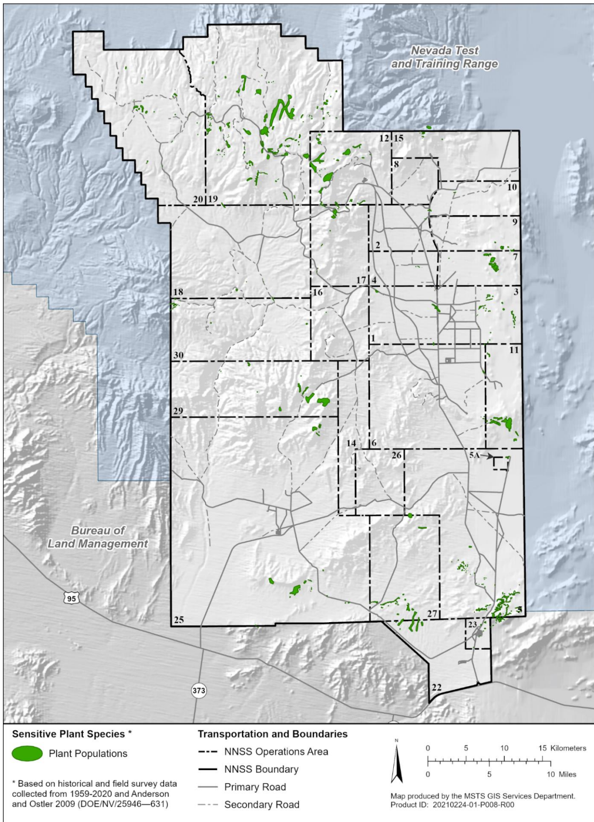
Figure A-20. Known locations of sensitive plant species on the NNSS (Anderson and Ostler 2009)
