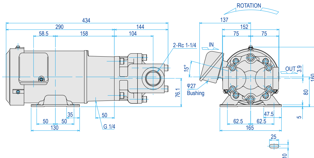
Model : TOP-3MF750-N3**FB-** IE3
