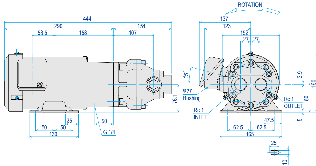
Model : TOP-3MF750-N3**FB-** IE3
