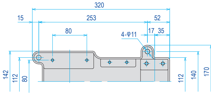
Model : TOP-1MBT200-1*HGI-**
