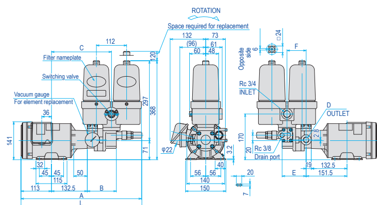
Model : TOP-2MY750-2**HWMDPVDE-005 IE3
