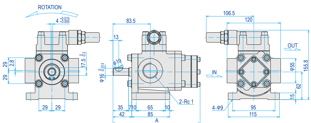
Model : TOP-25**HGAR-**
