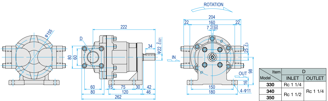
Model : TOP-3**VVB-**
