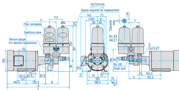
Model : TOP-2MY1500-2**HWMDPVDE-005 IE3
