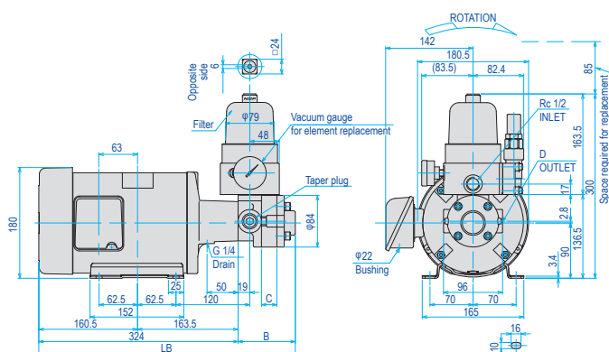
Model : TOP-2MY1500-2**HWMPVBE IE3
