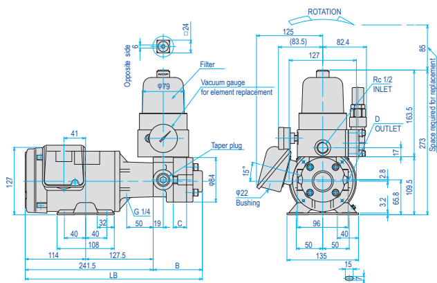
Model : TOP-2MY400-2**HWMPVBE
