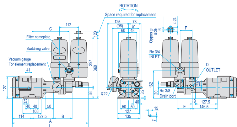
Model : TOP-2MY400□-2**HWMDPVDE-005
