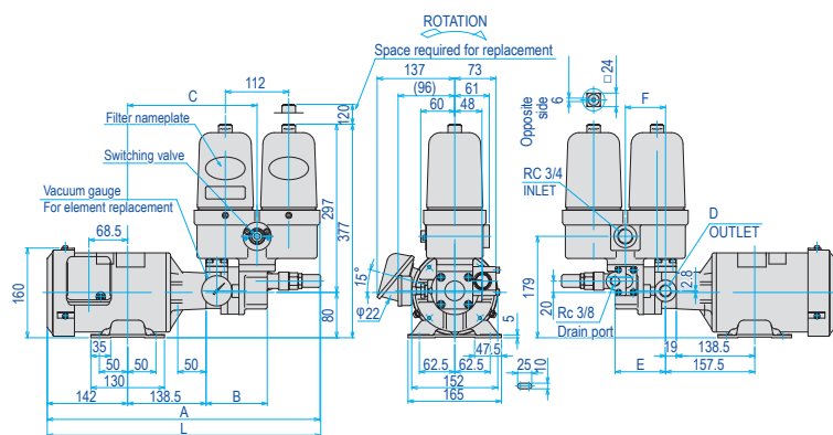
Model : TOP-2MY750-2**HWMDPVDE-005 IE3
