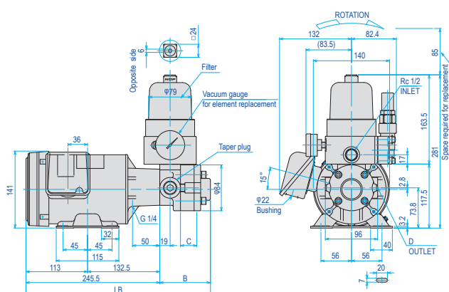
Model : TOP-2MY750-2**HWMPVBE IE3
