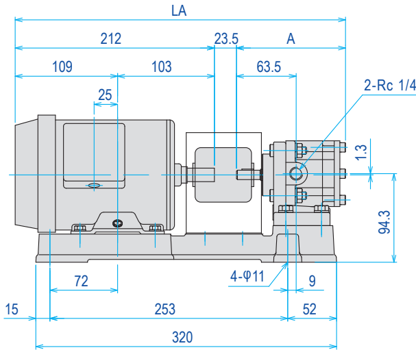
Model : TOP-1MBT400-1*HGI-**
