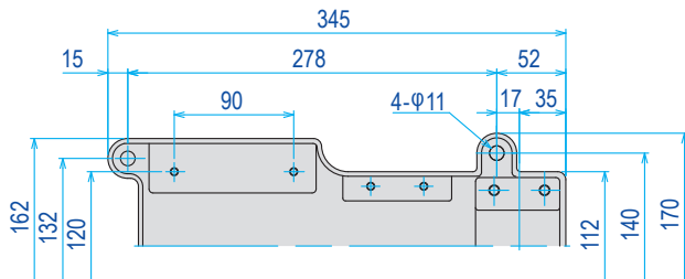
Model : TOP-1MBT400-1*HGI-**
