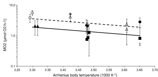
Fig. 3 Calculated mass-normalized SMR ( MO_2 \pm 1 SE, calculated for each species and normalised to 223 mg AFDM) against Arrhenius body temperature. Separate regression lines were fitted to Northern (open symbols, dashed line) and Southern (closed symbols) Hemisphere species, comprising 477 individuals across 17 species: bivalves of the genus Laternula (circles), gastropods of the family Buccinidae (triangles), echinoids of the infraorder Echinidae (diamonds), brachiopods (squares). Solutions fitted from results of a linear mixed effects model which accounted for the significant random effects of species nested in family. Note natural logarithm scale on the y-axis. Species tested at an Arrhenius body temperature of 3.48 K were slightly offset for clarity
