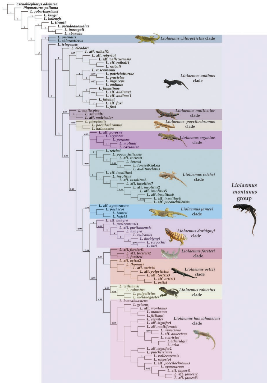
Figure 7. Mixed Bayesian hypothesis.
